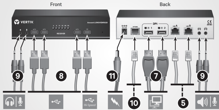
LongView™ Extender Configuration (Receiver)
