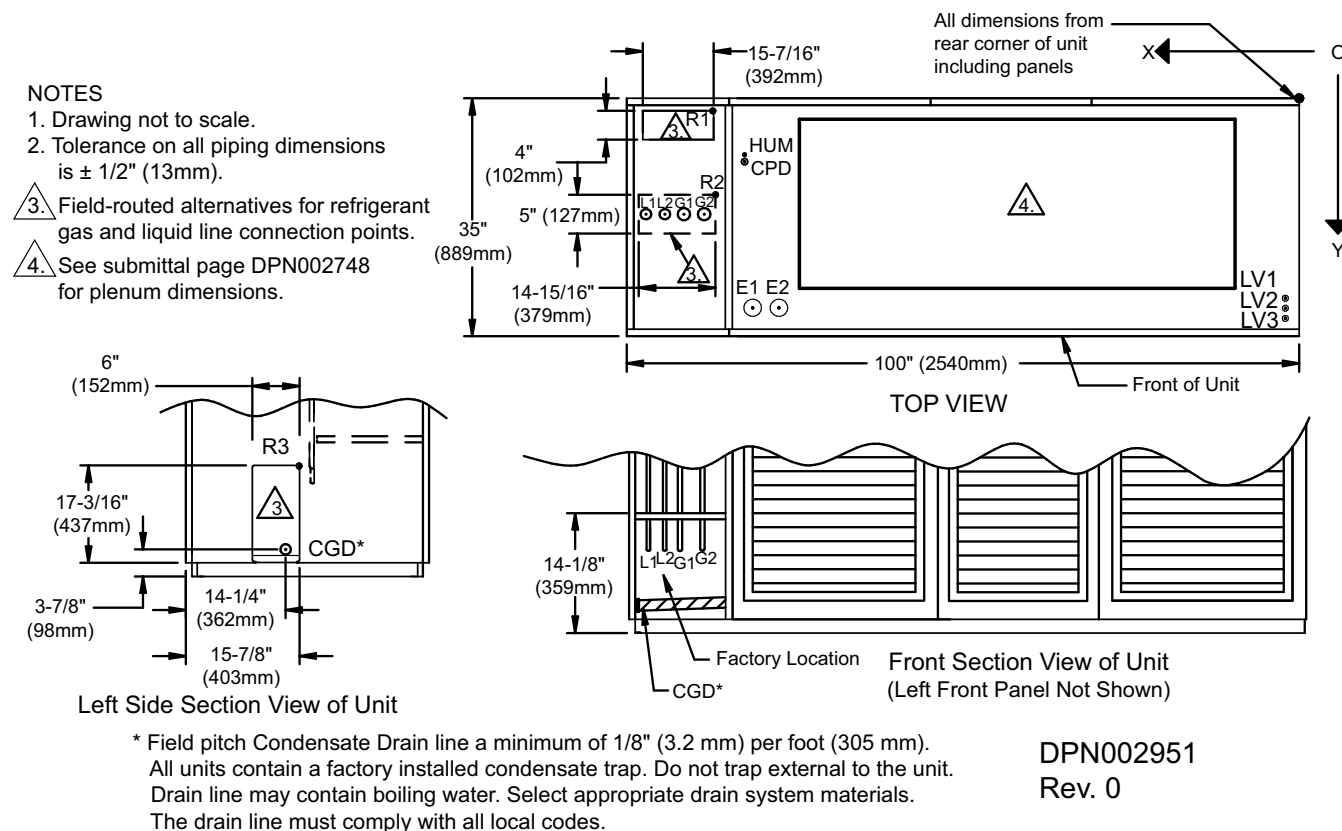
Figure 79 Primary connection locations—Upflow, air-cooled DA080U, DA085U scroll compressor models
