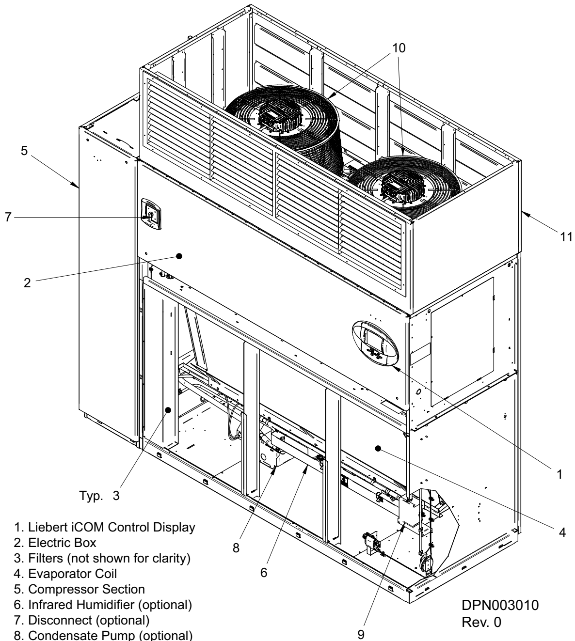
Figure 2 Upflow model component locations
