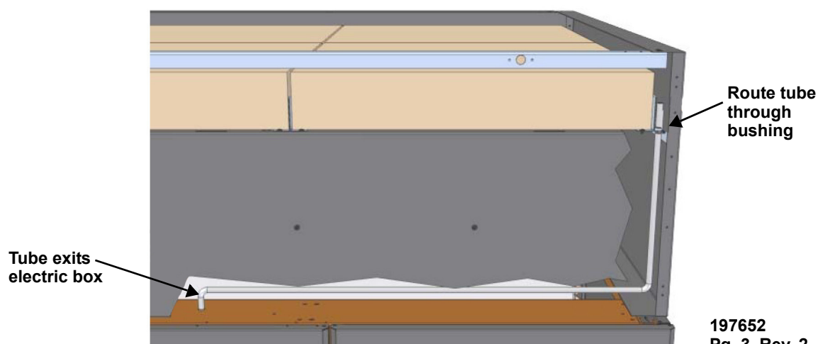
Figure 62 Route filter clog sensing tube
