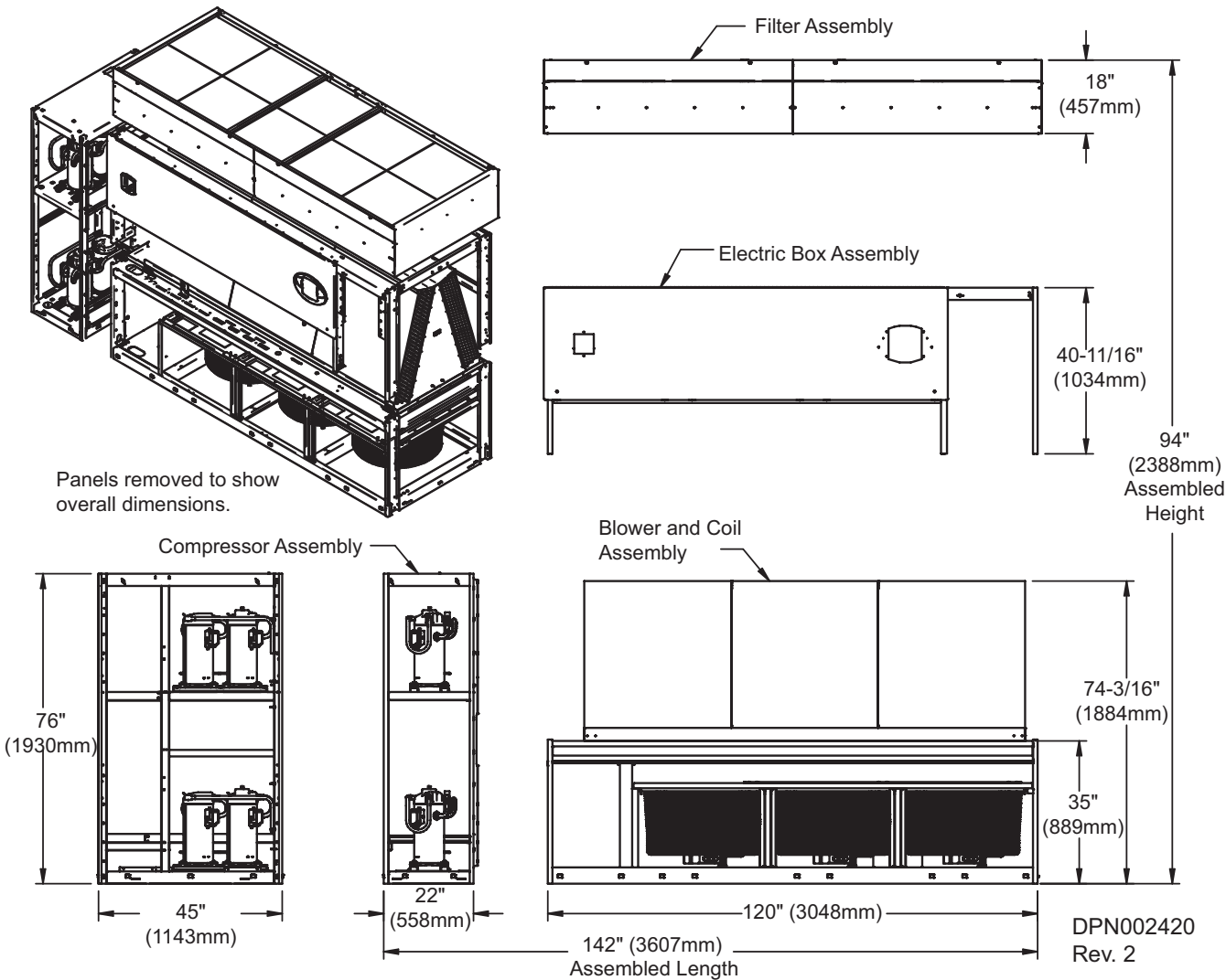
Figure 64 Component dimensions, Liebert DSE models DA125 and DA150 downflow units
