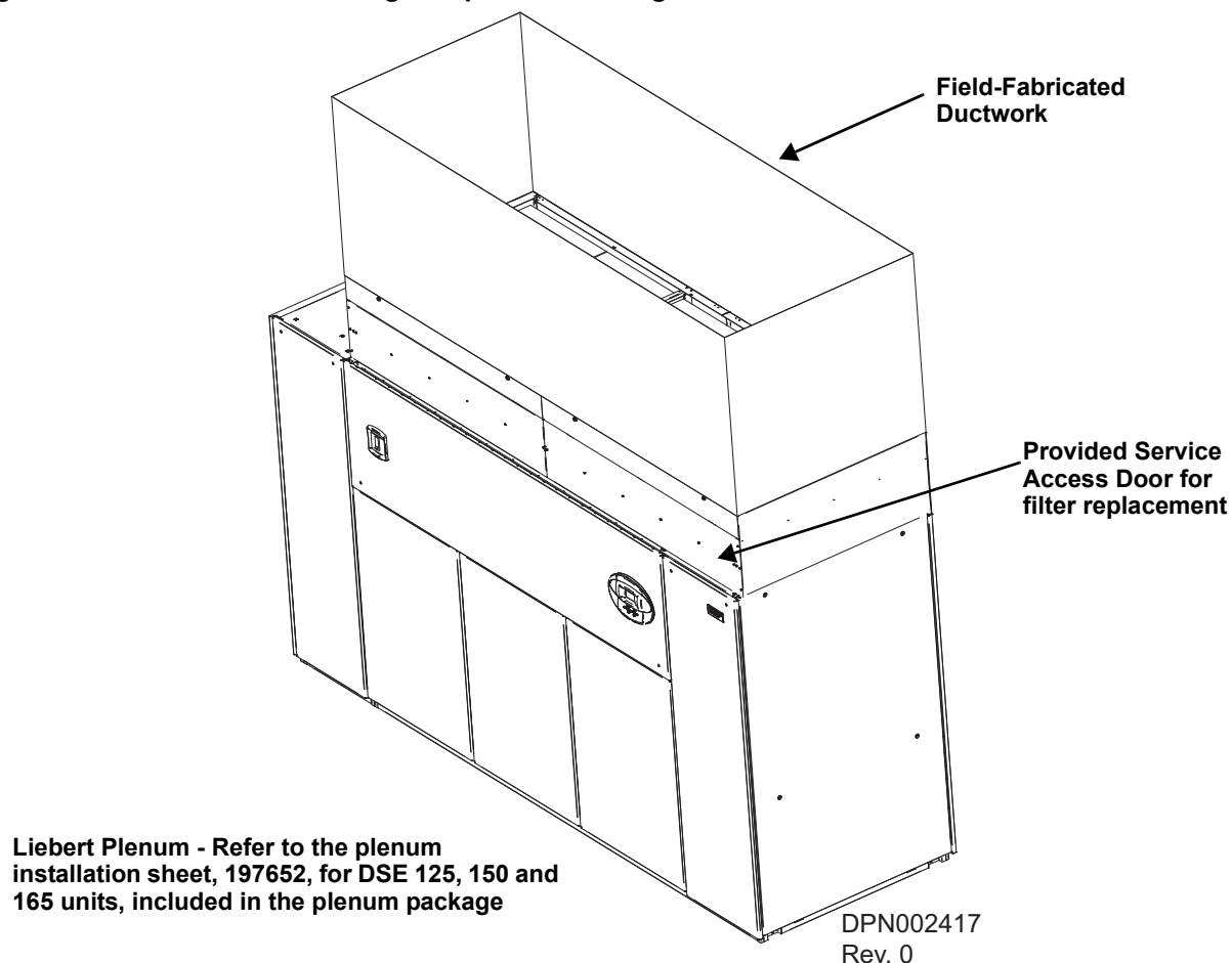
Figure 4 Downflow unit ducting and plenum ducting
