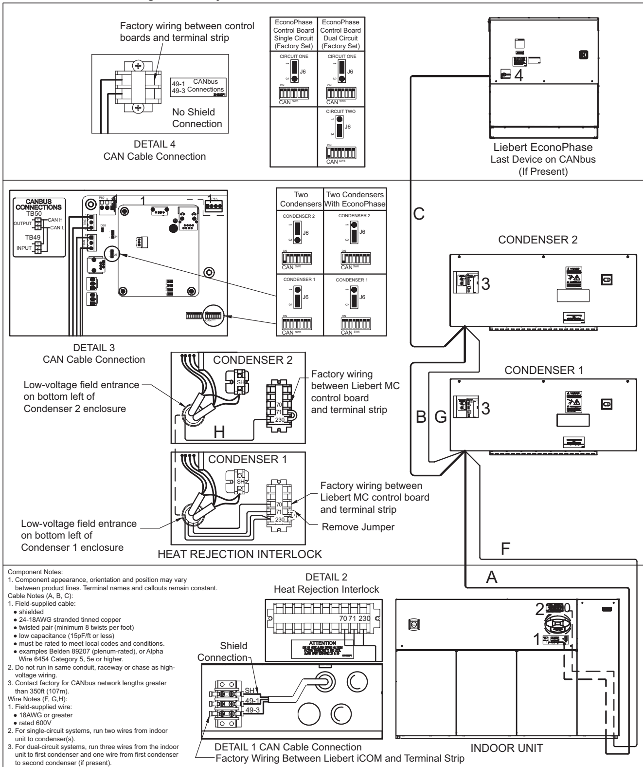
Figure 70 CANbus cable connections between indoor unit, Liebert MC™ condenser and optional Liebert EconoPhase™ pumping unit
