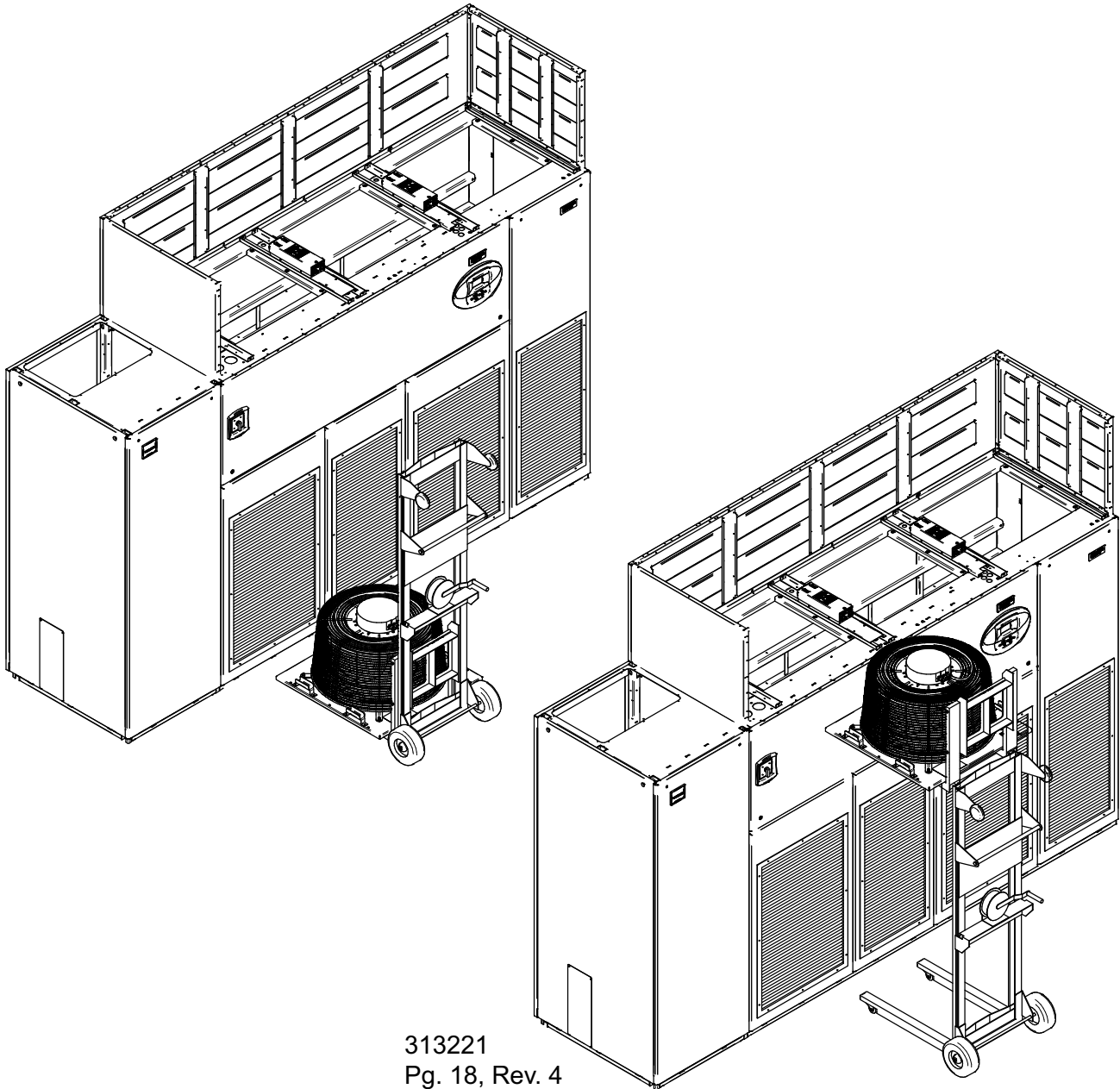
Figure 43 EC fan assembly alignment for placement on top of Liebert DSE
