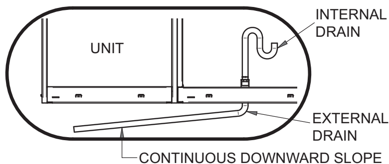
Figure 72 Gravity drain for downflow units
