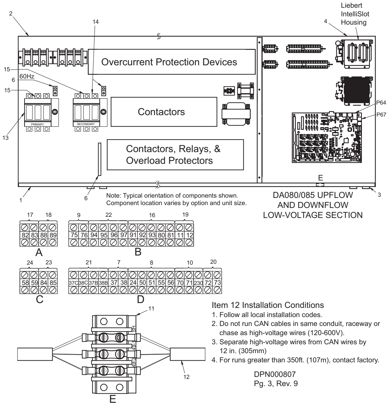
Figure 67 Electrical field connections, DA080 and DA085 upflow and downflow models, dual-fused disconnect switches
