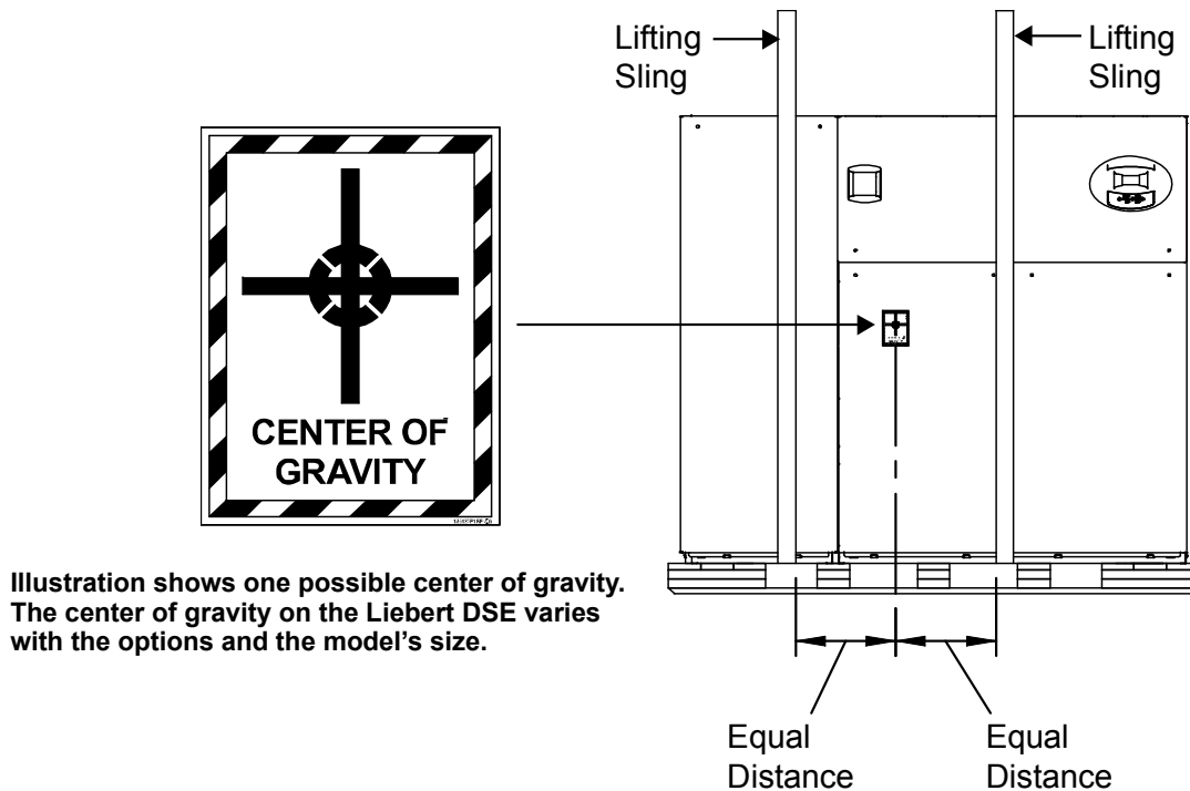
Figure 18 Locate center of gravity marker and place slings
