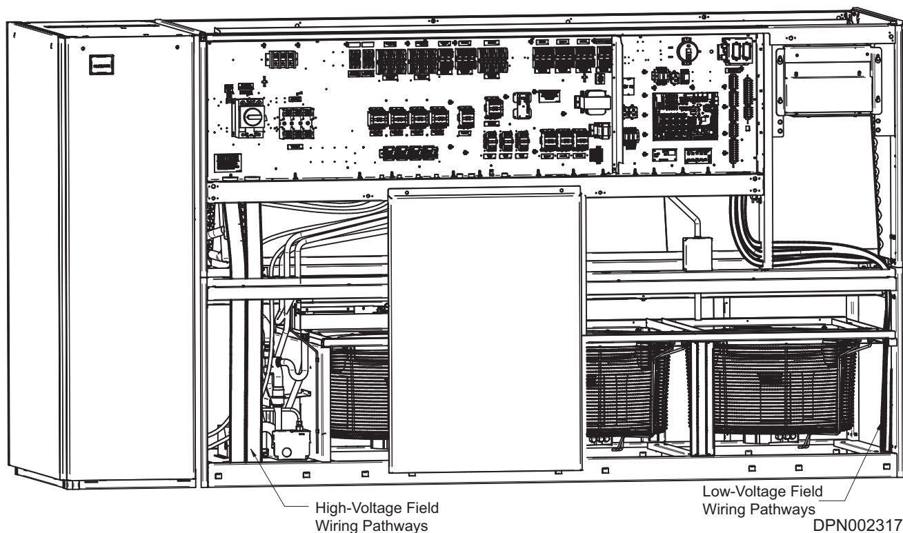
Figure 68 Electrical field connections for DA125 and DA150 downflow models
