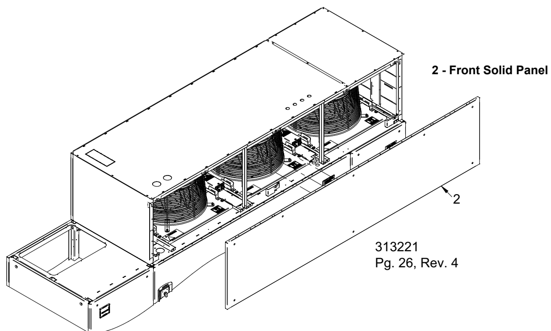
Figure 54 Rear-grilled plenum front panel attachment
