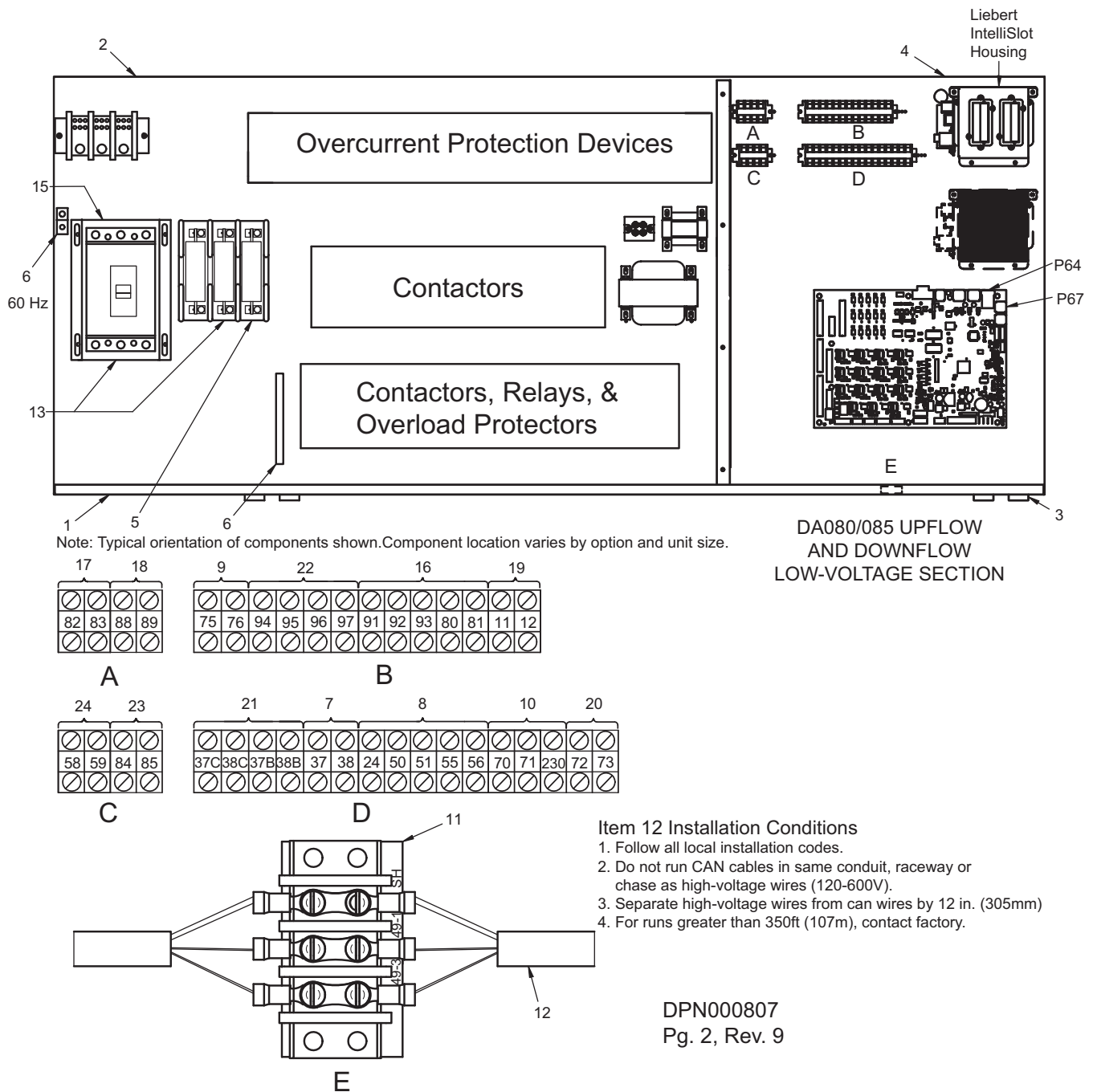
Figure 66 Electrical field connections DA080, and DA085 upflow and downflow models, single-molded case switch disconnect with main fuses
