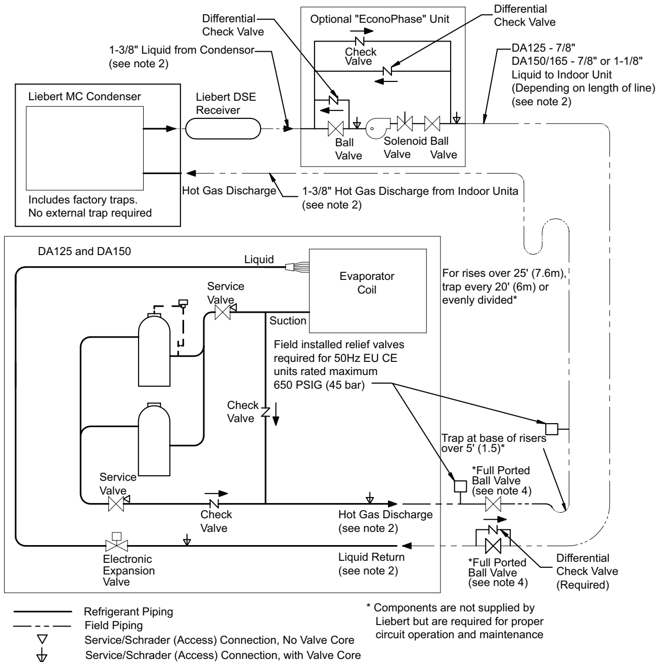
Figure 74 Piping schematic—Air-cooled DA125 and DA150 models
