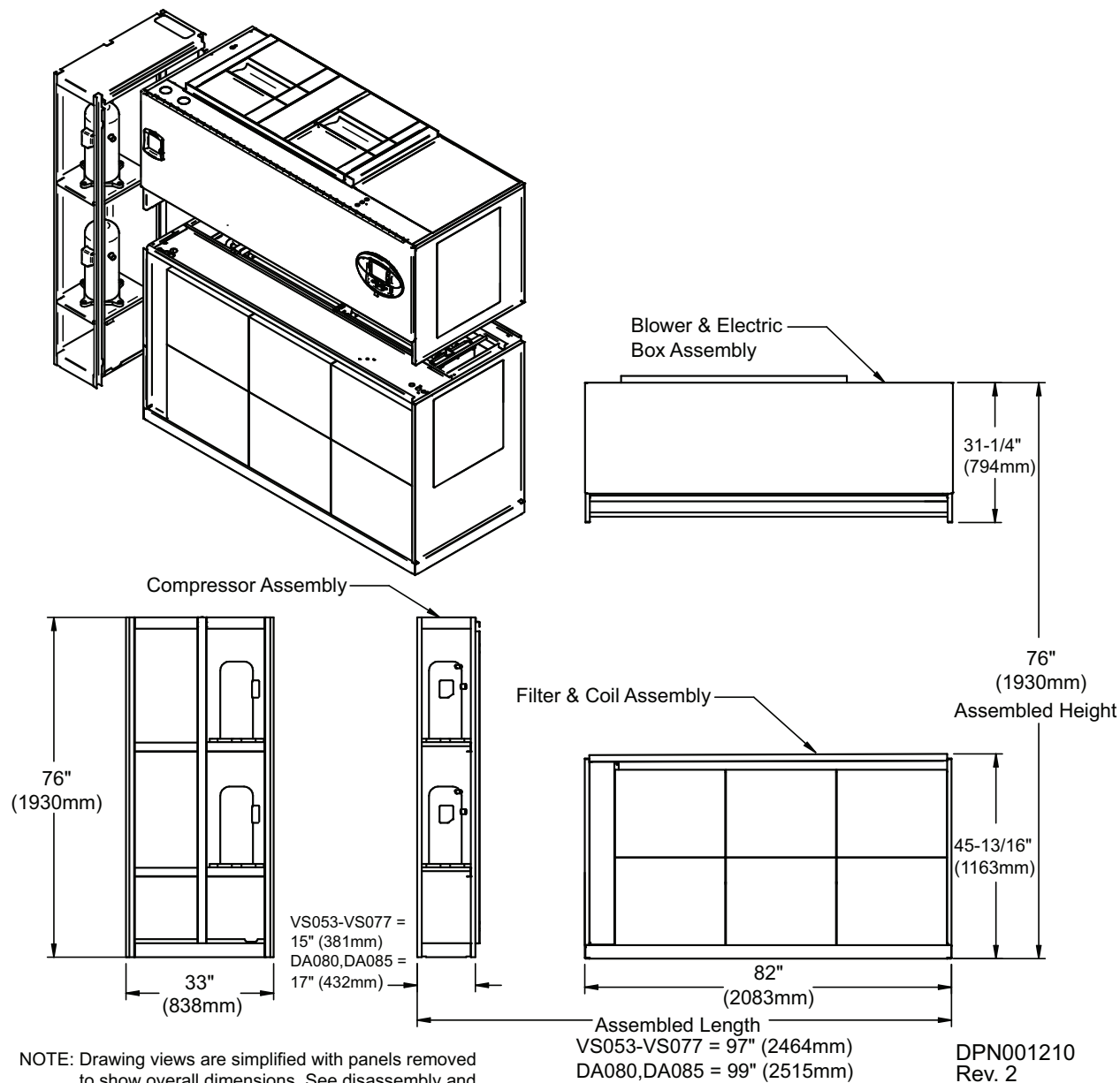
Figure 65 Component dimensions, Liebert DSE upflow models DA080U and DA085U
