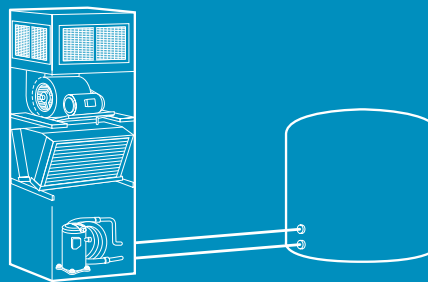
Split-System
