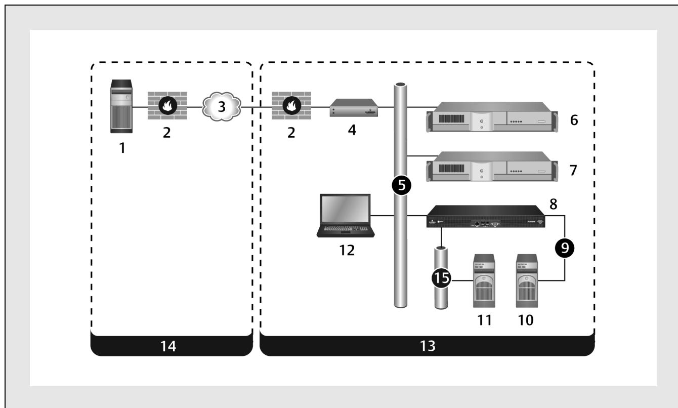
Figure 2.2 Installation on a Separate Private Network for Facility Equipment
