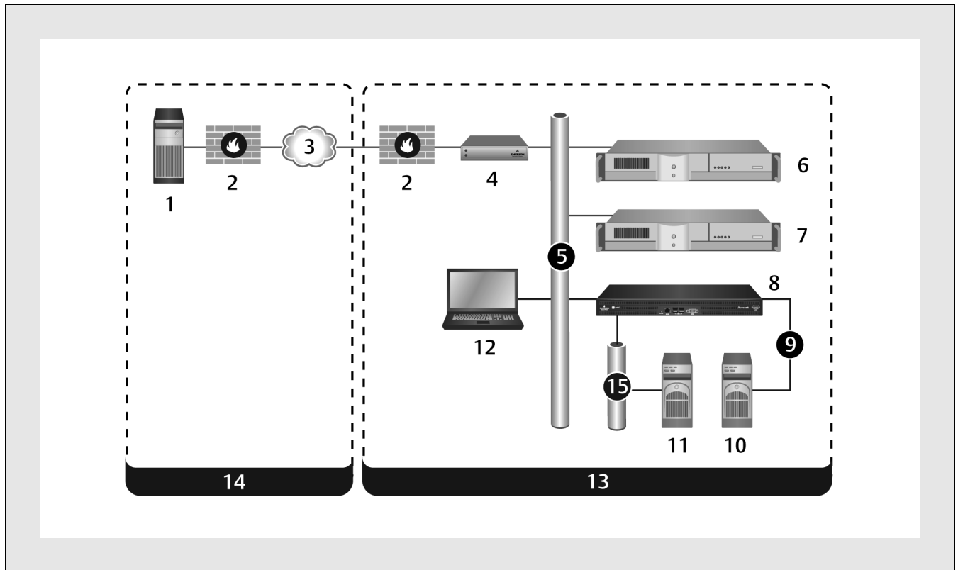
Figure 2.1 Installation on a Separate Private Network for Facility Equipment
