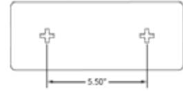
Wall Mounting Detail Rear View
