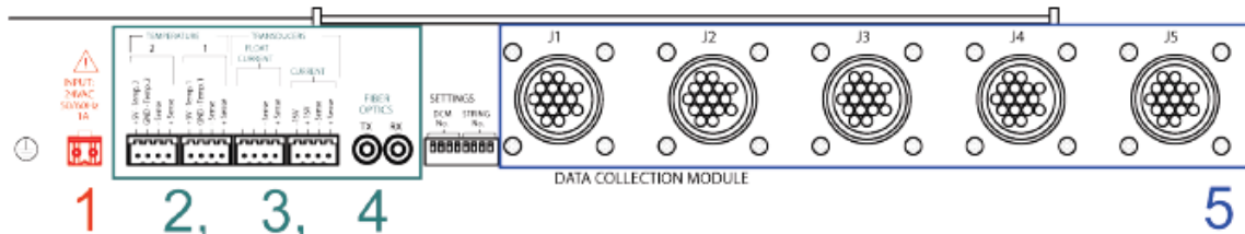
Figure 7. Base Unit DCM Rear Panel Connectors
