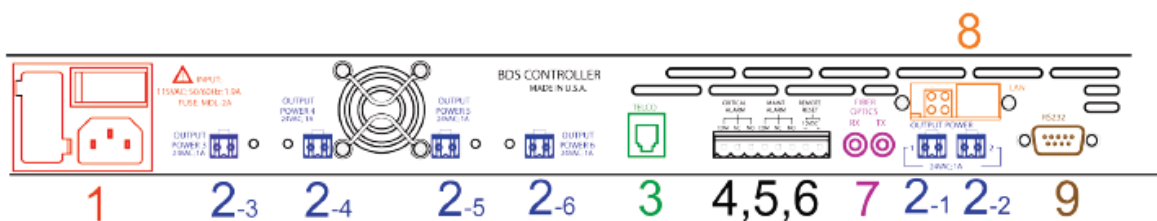
Figure 6. BDS-40 Base Unit Controller Rear Panel Connectors
