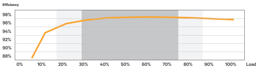
eSure™ 15kW High-Efficiency Rectifier
