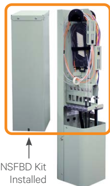
Vertiv™ BBE BD Series NSFBD Fiber Distribution Kit
