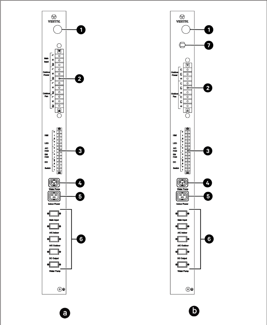
Figure 1 - PMB Appearance
