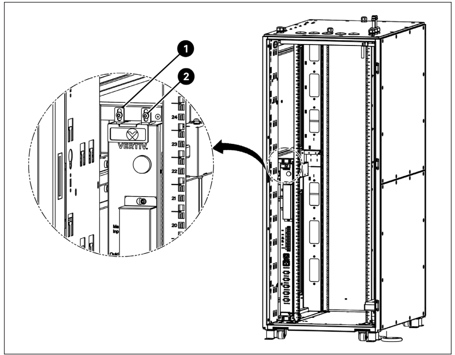
Figure 4 - Installation of Mounting Bracket to the Cabinet
