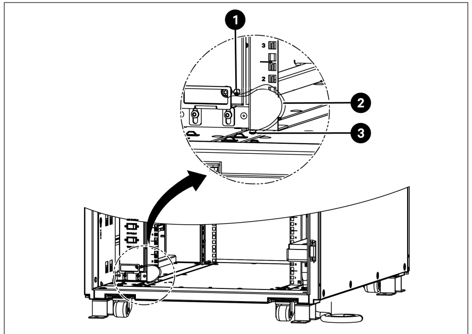
Figure 5 - Grounding Connection of the PMB
