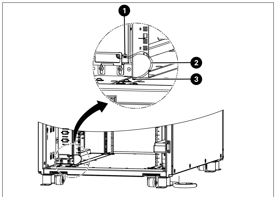
Figure 5 - Grounding Connection of the PMB
