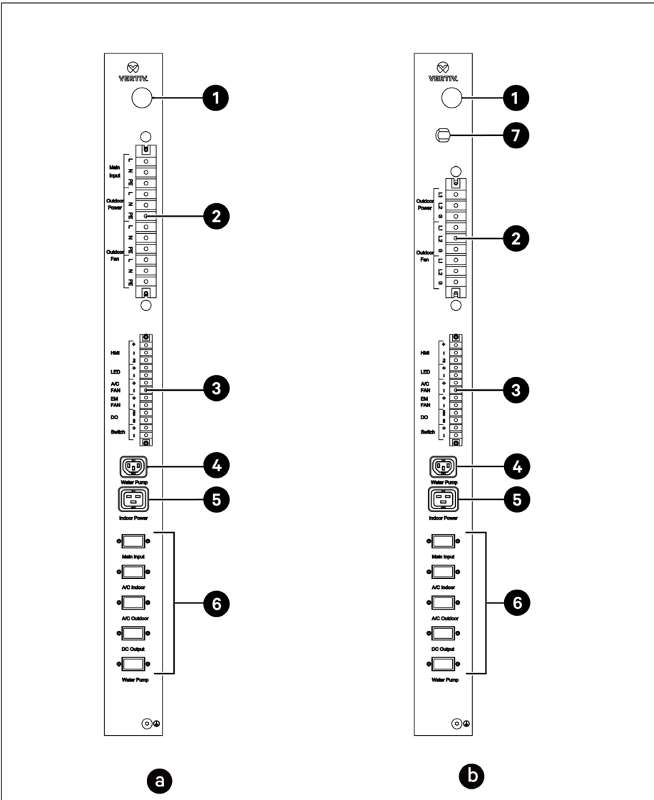
Figure 1 - PMB Appearance
