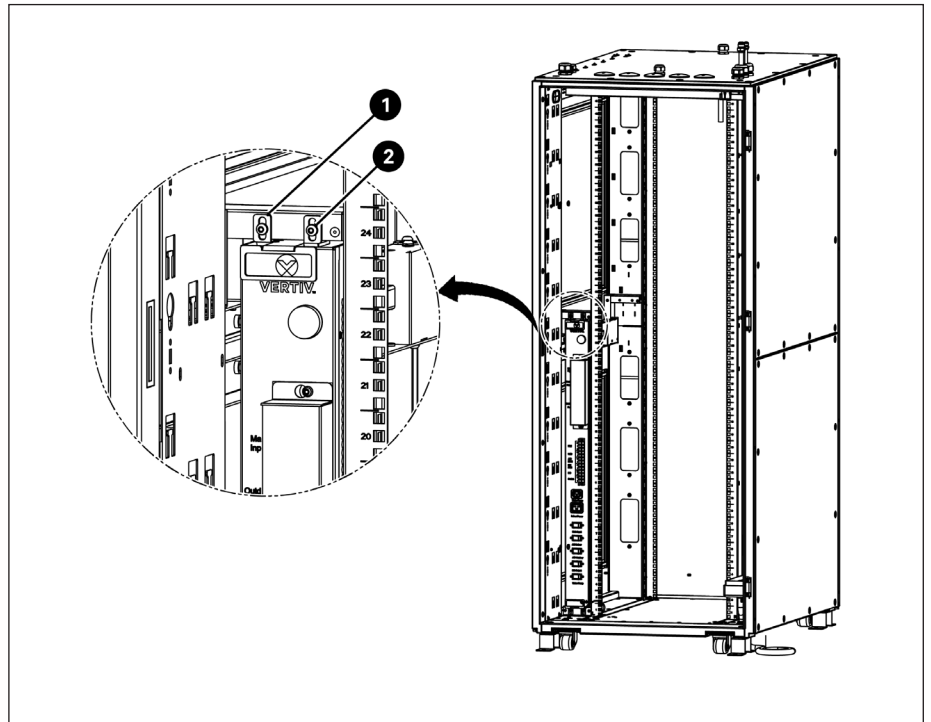
Figure 5 - Grounding Connection of the PMB
