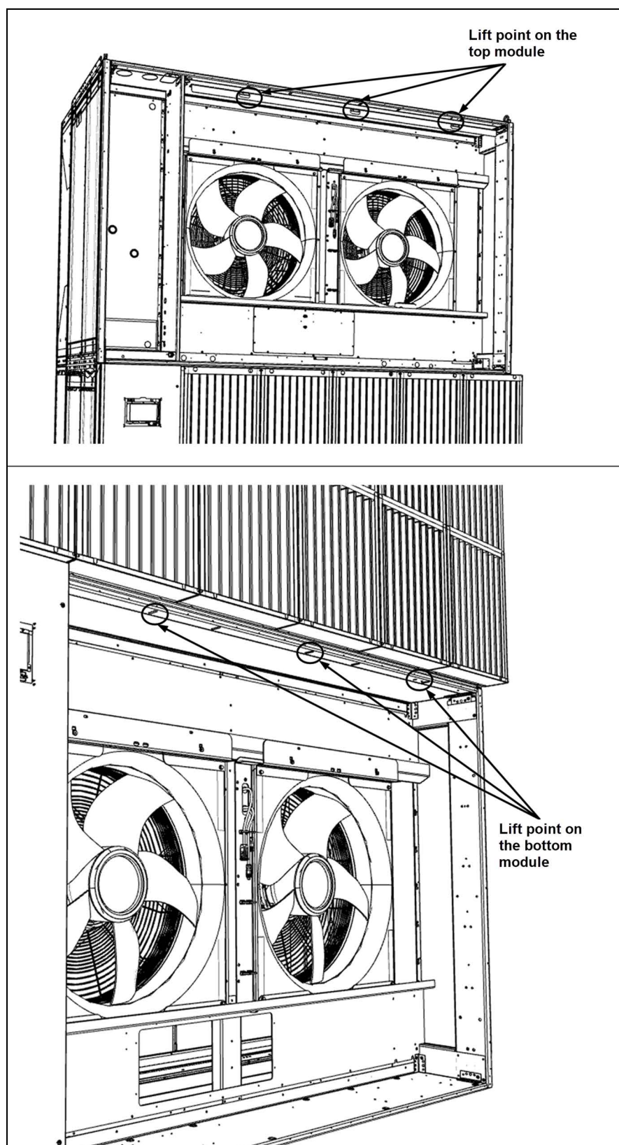
Figure 9.6 Lift Point for Top and Bottom Modules
