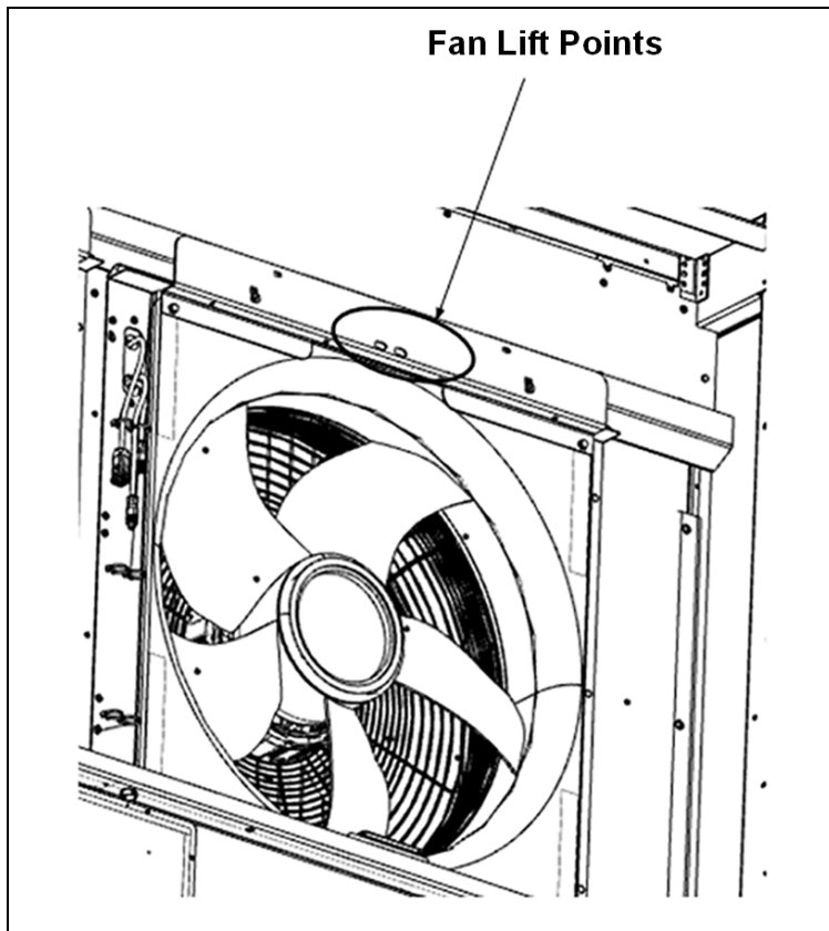
Figure 9.8 Axial Fan Lift Points
