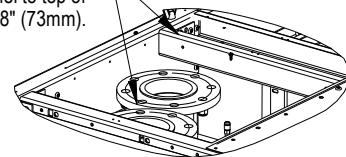
Detail B (Chilled Water Field Connection)
