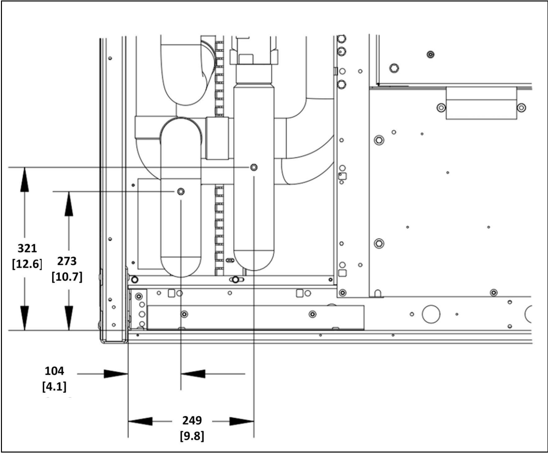
Figure 4.4 Bottom Module Supply and Return Pipe Detail
