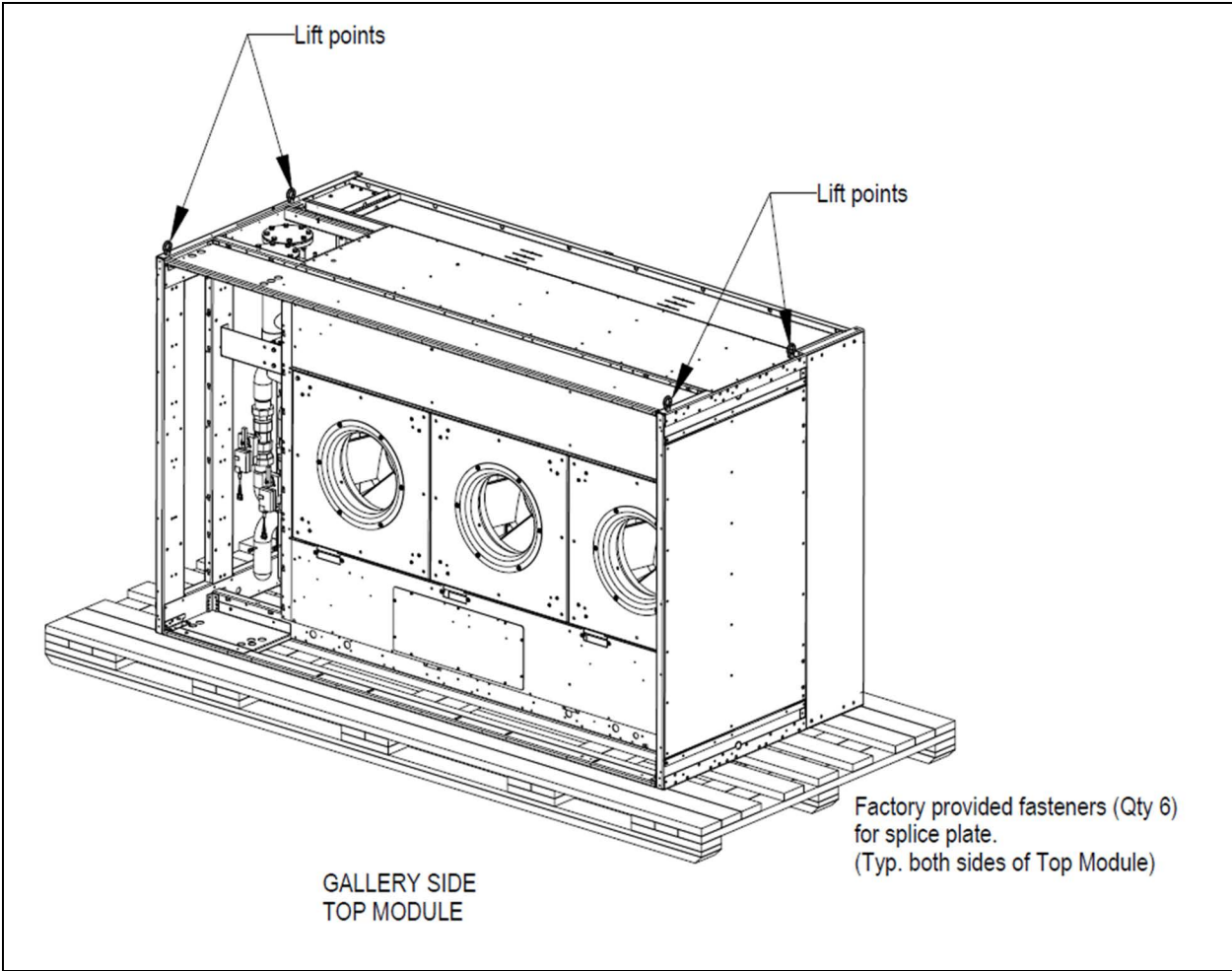
Figure 4.11 Lifting Points
