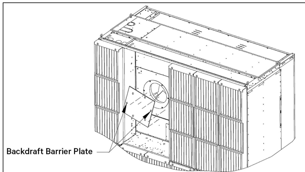
Figure 9.3 High Airflow, High Efficiency Fan Backdraft Barrier Plate Kit
