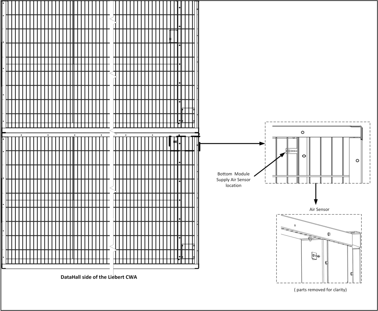
Figure 5.4 CWA Air Sensor Location
