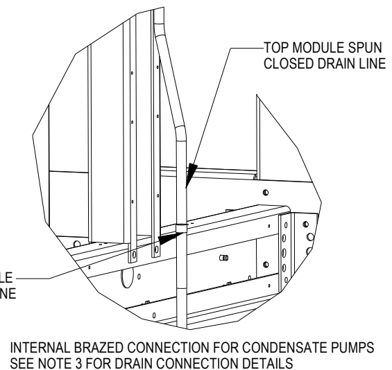
DRAIN LINE ROUTING FRAME SHOWN FOR REFERENCE. SOME MEMBERS HIDDEN FOR CLARITY
