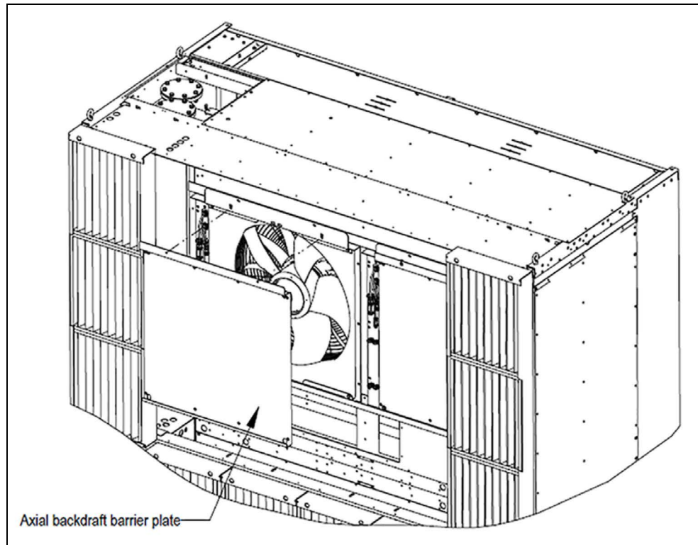
Figure 9.3 High Airflow, High Efficiency Fan Backdraft Barrier Plate Kit
