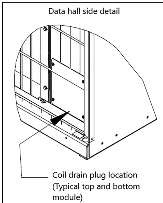
Figure 9.10 Coil Drain Plug Detail
