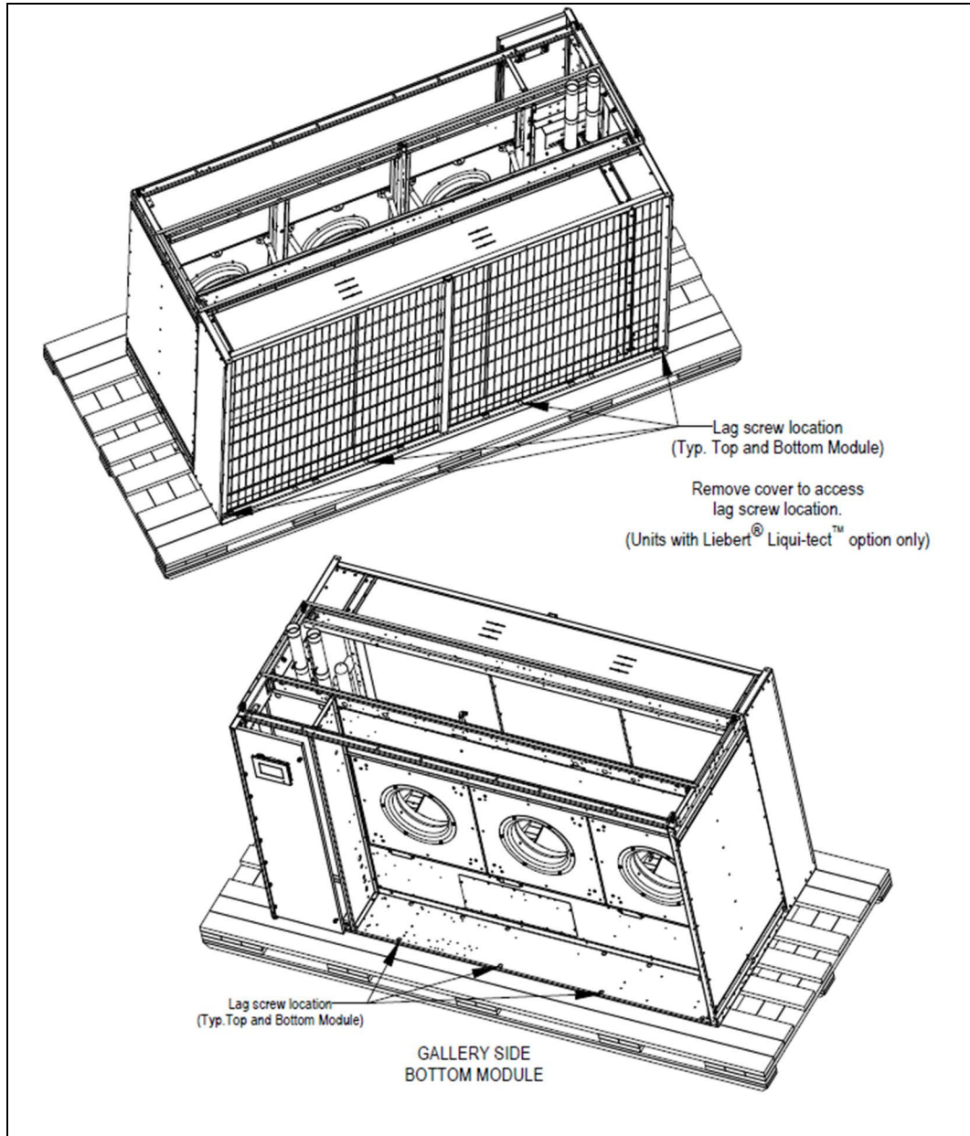
Figure 4.10 Lag Screw Removal
