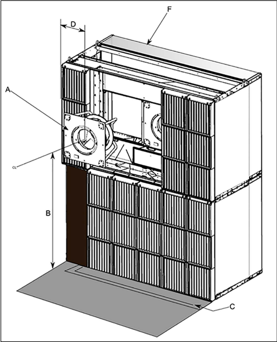
Figure 9.9 Clearance Dimensional Data
