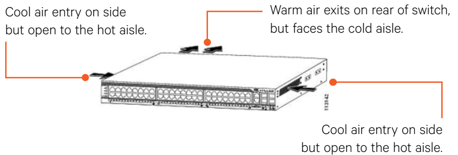
Cisco Catalyst 4948 1
