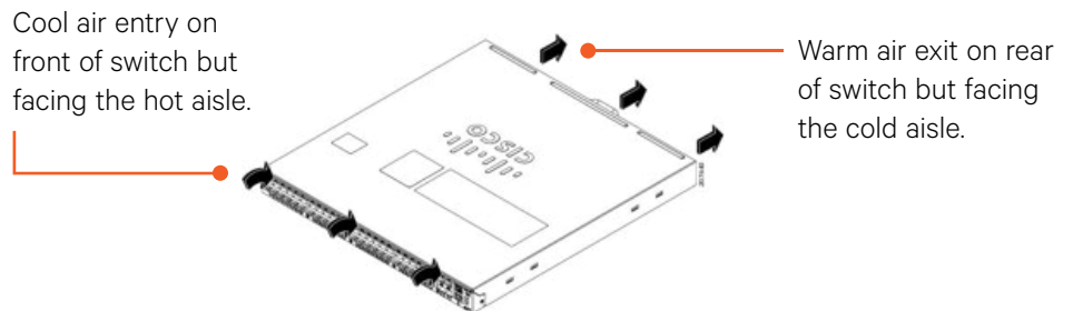
Cisco Catalyst 4948E 2
