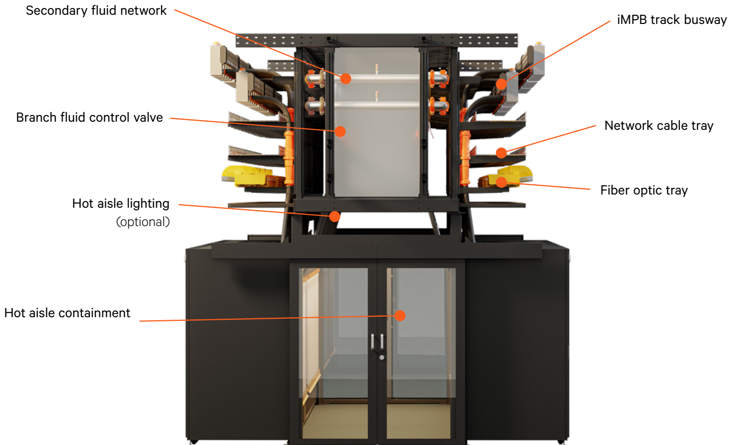
Frontal view of Vertiv™ SmartRun with racks
