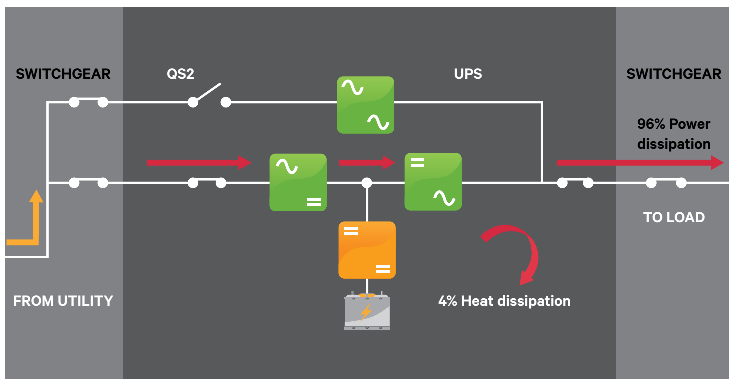
Figure 1: Traditional Load Bank Test
