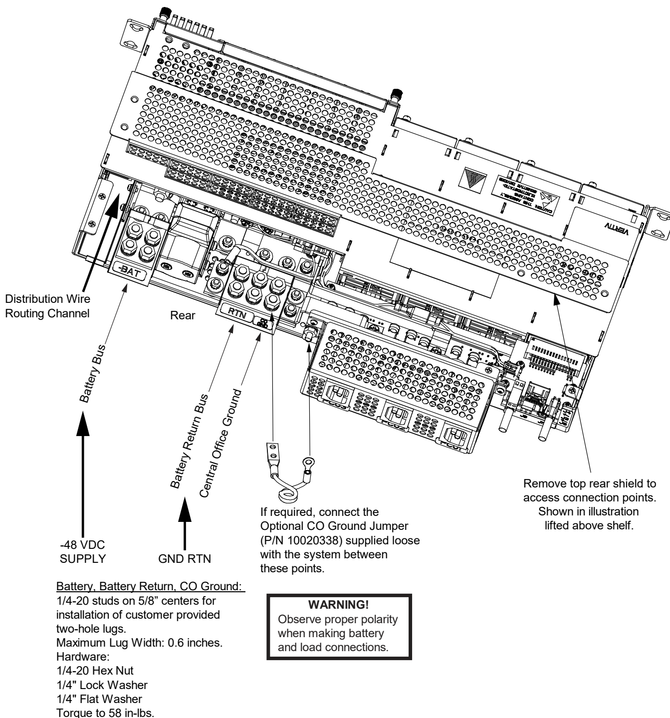
Figure 13 (cont'd on next page) Load Distribution Wiring, Input Battery Wiring, and CO Ground Wiring (List BA)
