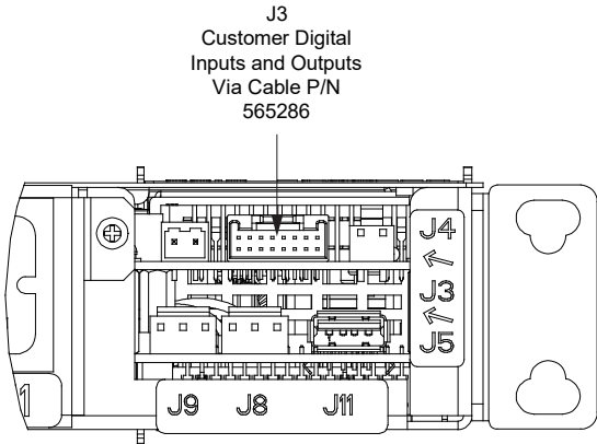
Figure 5 External Alarm, Reference, Monitoring, and Control Connections Locations (cont’d from previous page, cont’d on next page)
