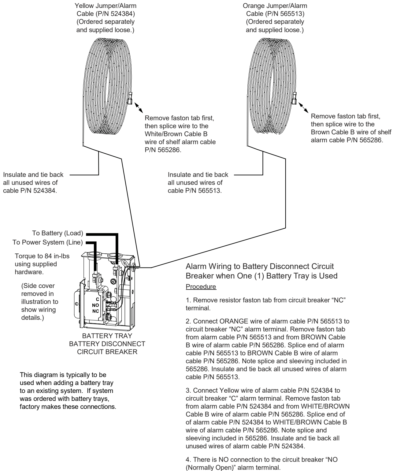
Figure 7 Alarm Wiring to Battery Disconnect Circuit Breaker when One (1) Battery Tray is Used (cont'd on next page)
