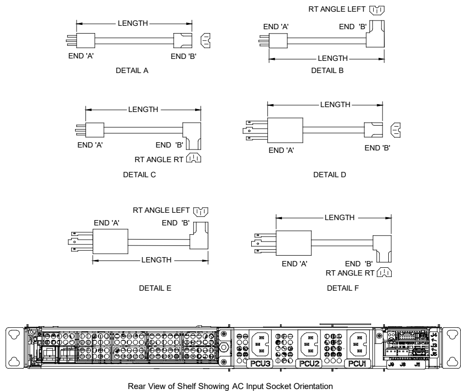
Figure 1 AC Input Kit Option P/N 564840 (One AC Feed per Rectifier Position)
