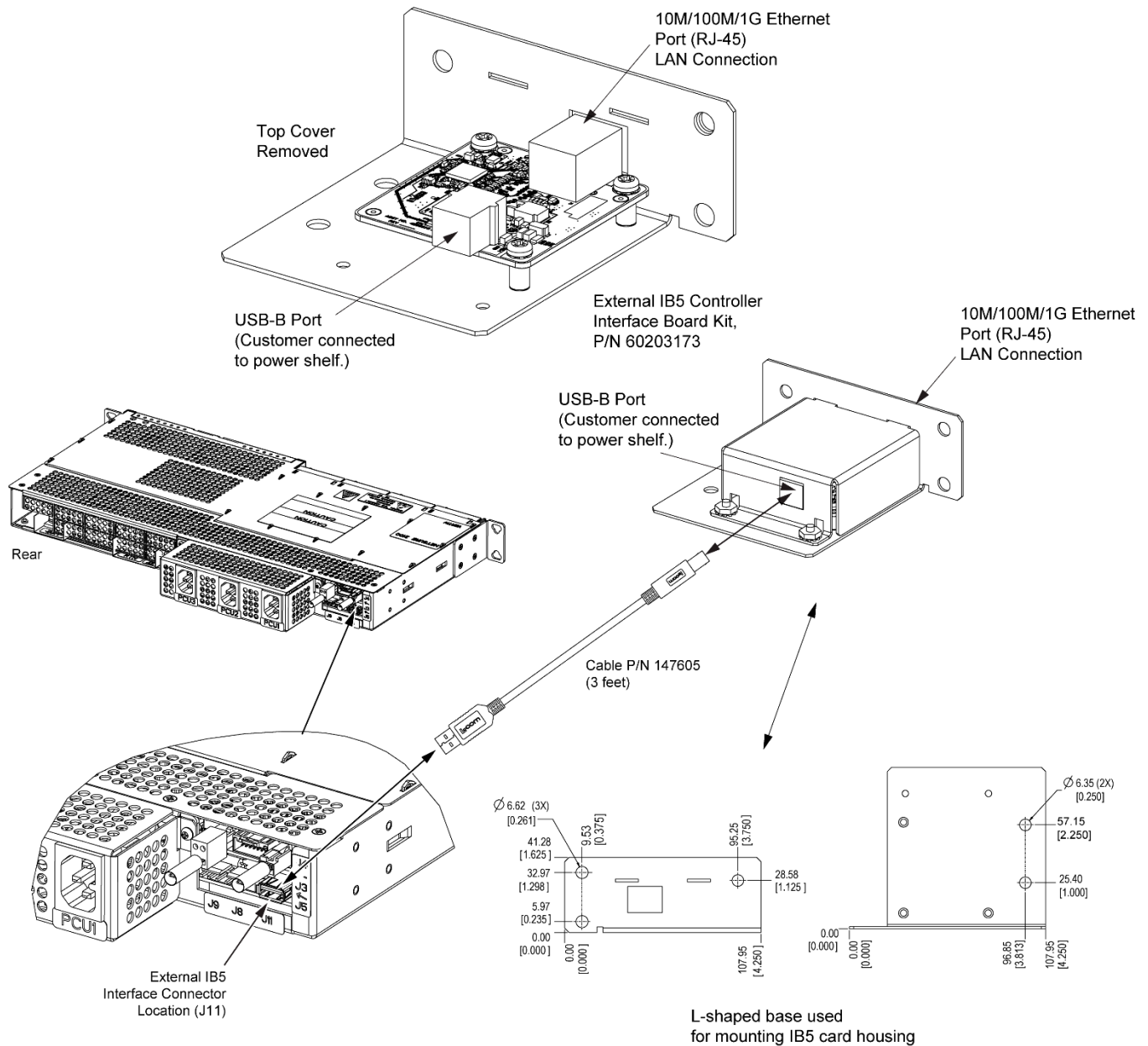
Figure 6 Optional External IB5 Connections Locations
