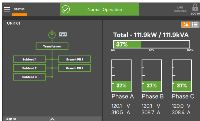
Figura 1: Pantalla principal de DPM Observer
