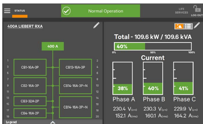
Figure 2. On left is a "single-line" electrical diagram of the Vertiv™ Liebert® RXA unit, displaying the input and output distribution of branch panel boards and sub-feed breakers. On right is the unit's total output load, with individual power levels for each phase in a 3-phase distribution, including voltage and amperage for each phase.
