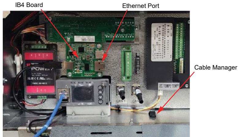
Figure 1.26 Connecting the Ethernet Cable
