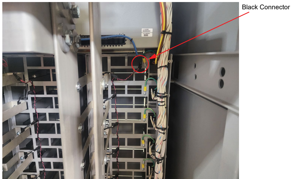
Figure 1.11 Removing the Black Connector to Disconnect the CAN Connection
