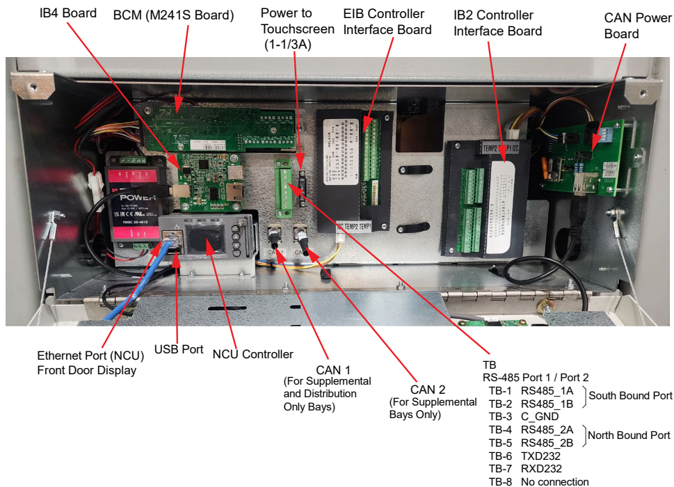
Figure 1.17 Component Layout
