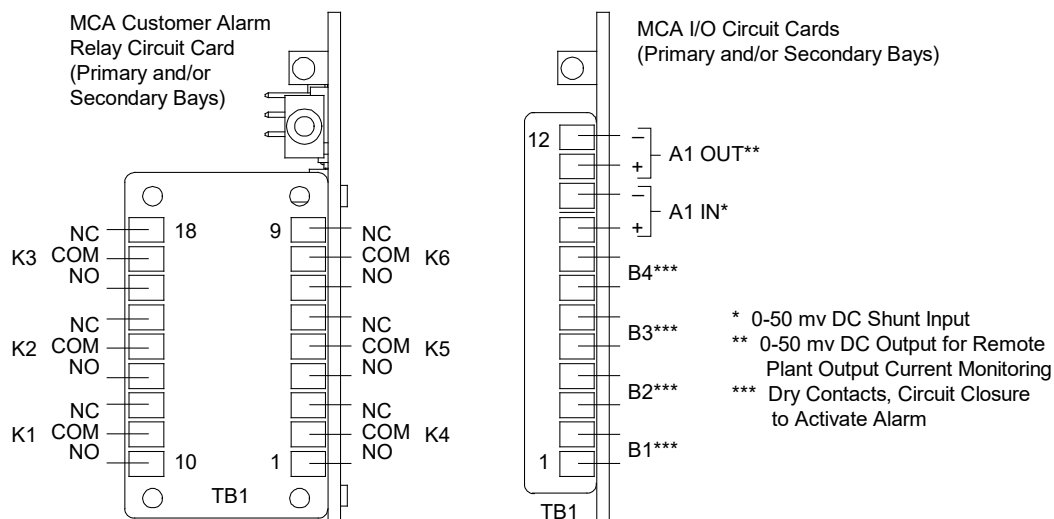
Detail MCA-C
