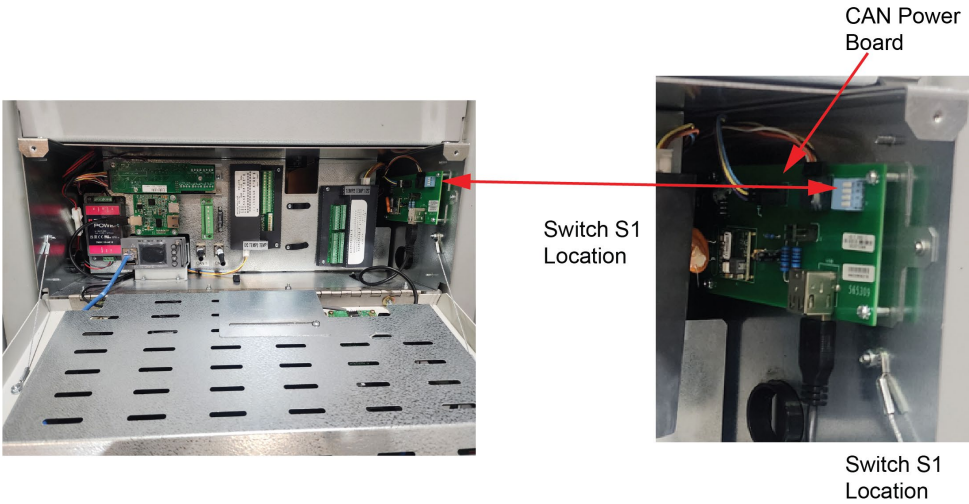
Figure 1.18 DIP Switch S1 (Bay Addressing)
