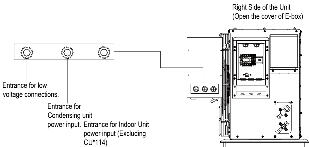
Electric control box layout and power supply system
