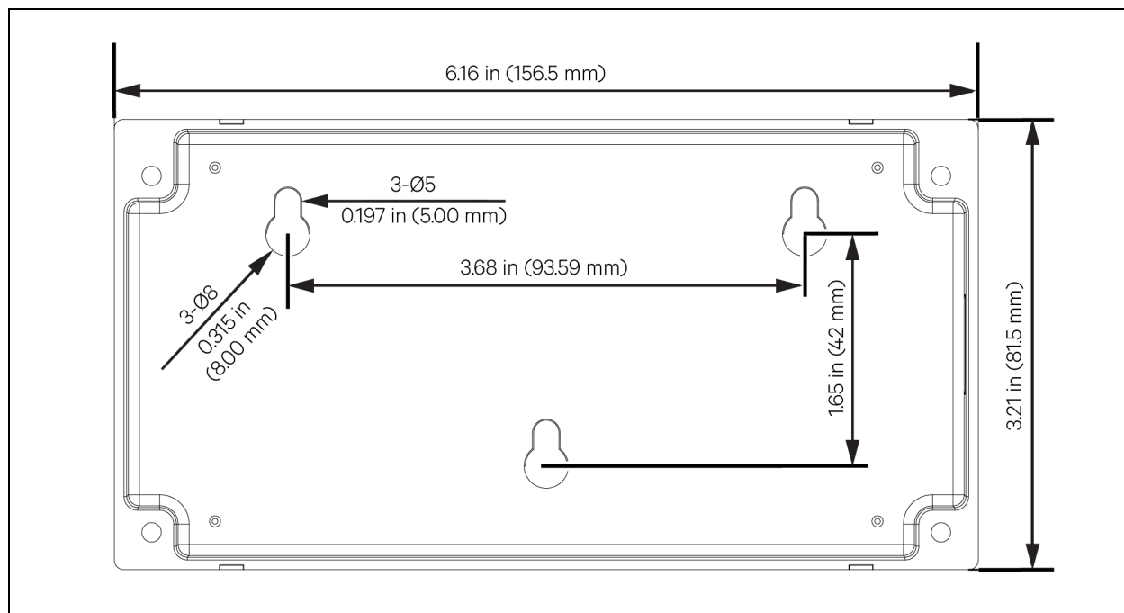
Figure 1.5 LCD Display Installation
