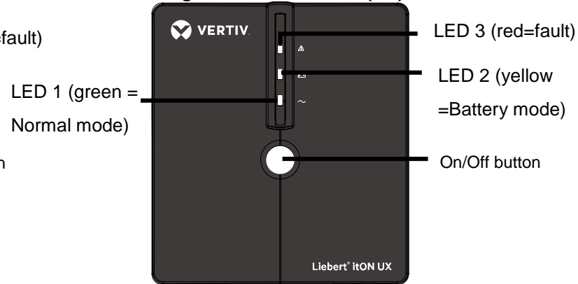
Figure 2 – Front Panel (UX)
