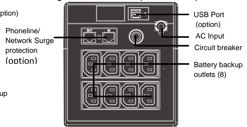
Figures 6 – Rear Panel (PSA1000-UX1)
