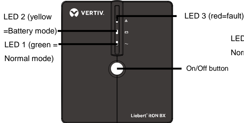
Figures 1 – Front Panel (BX)
