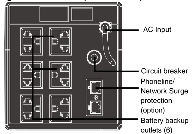
Figures 6 – Rear Panel (PSA1000-UX1)
