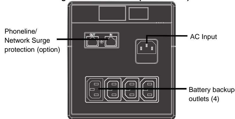
Figures 3 – Rear Panel (PSA1000-BX)
