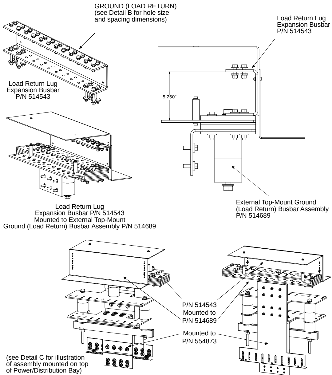
Load Return Lug Extension Busbar P/N 514543 (mounts to External Top-Mount Ground [Load Return] Busbar Assembly)
