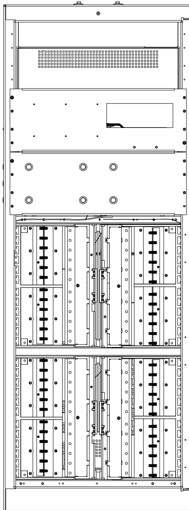
Front View
