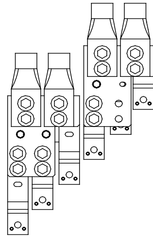
3-Position Lug Adapter Kit P/N 529131 (see Notes 2, 3, 4, 5)
