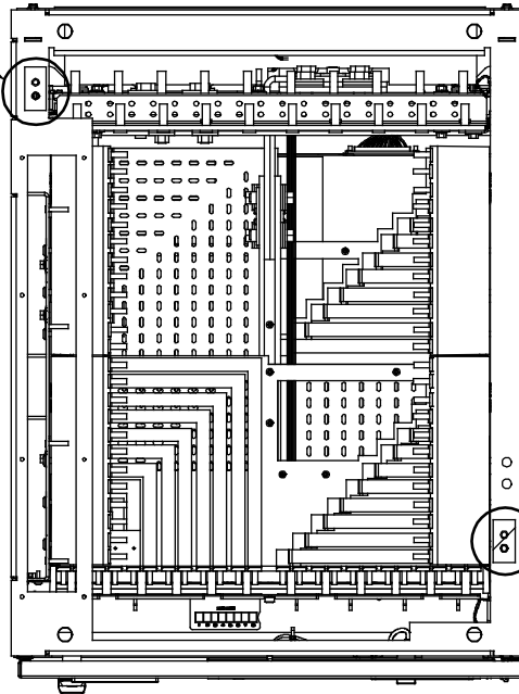
Top View Power/Distribution Bays (Power Only Bays Similar)
