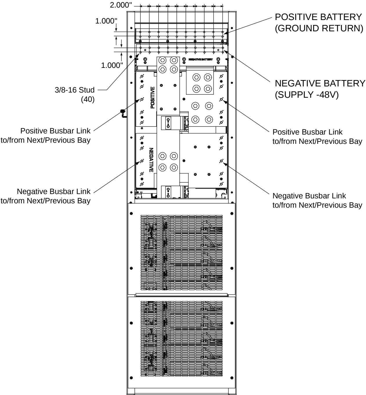
Rear View Power/Distribution Bays
