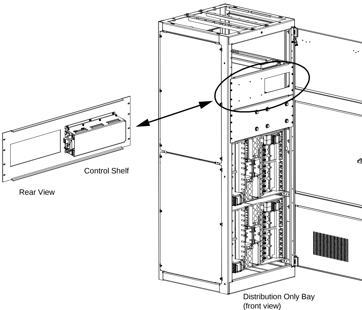
Figure 2 Older Style 582140000 List 16 Distribution Only Bay
