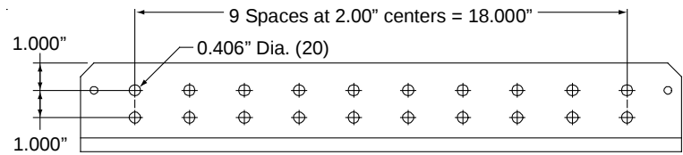
Detail B Negative Battery Busbar Hole Size and Spacing Dimensions (for installation of customer provided two-hole lugs with 3/8" clearance holes on 1" centers)
