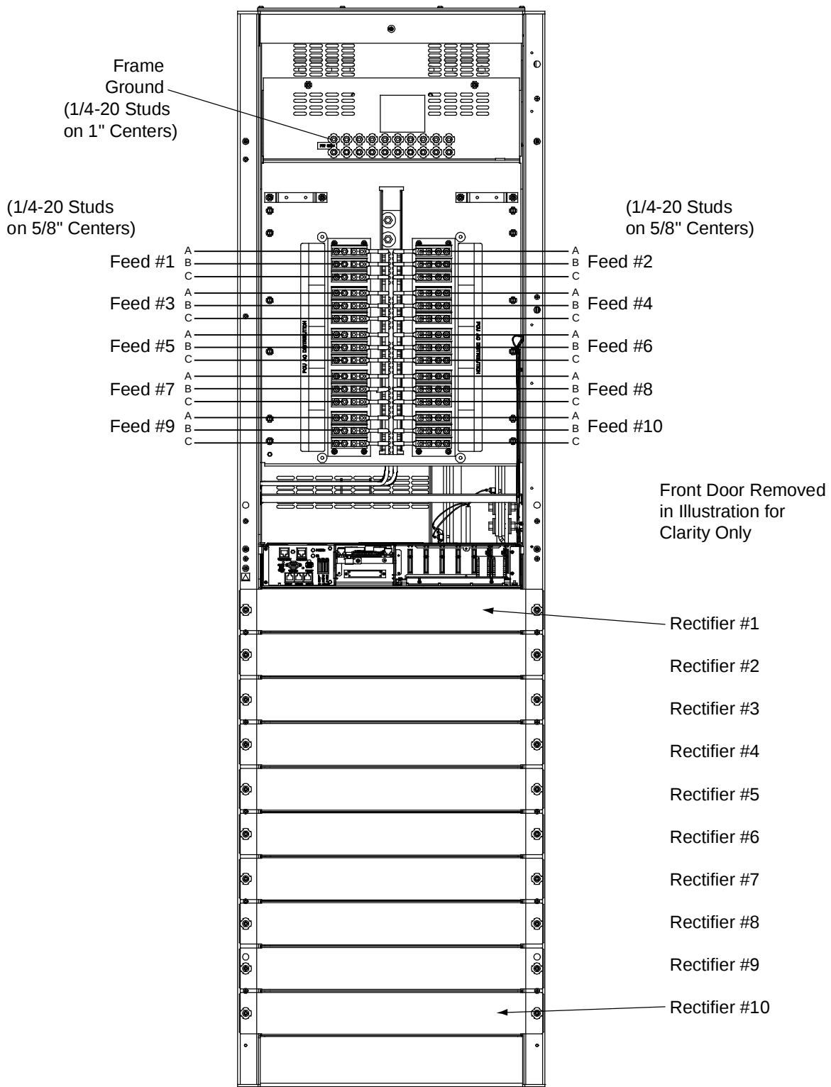
Front View
