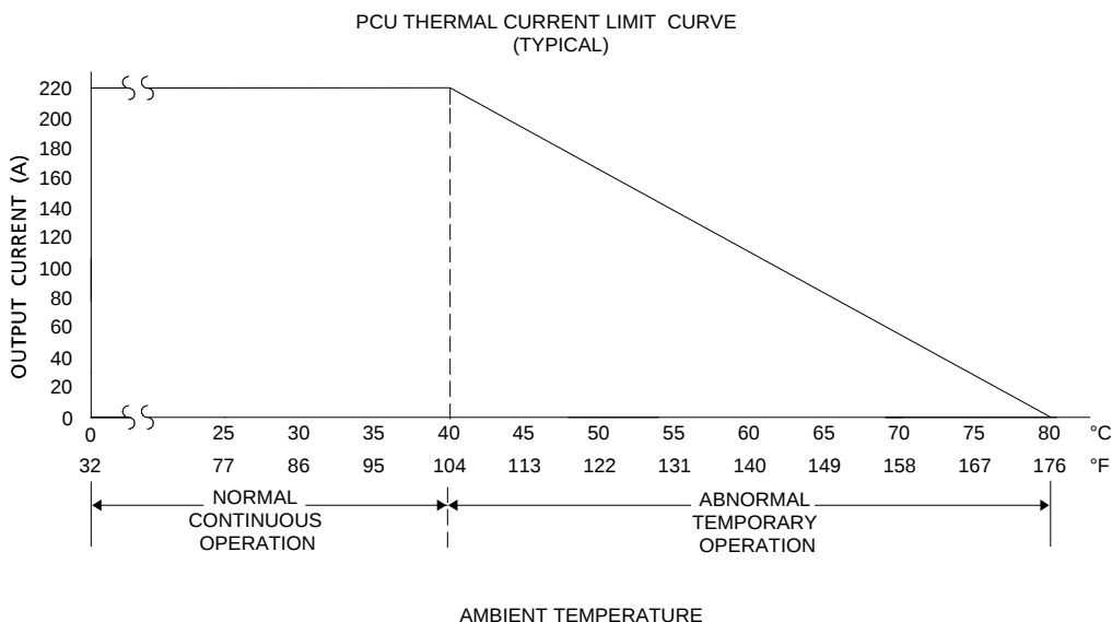
Typical Thermal Current Limit Curve
