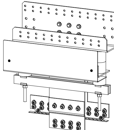
VIEW WITH BUSBAR SHIELD REMOVED
