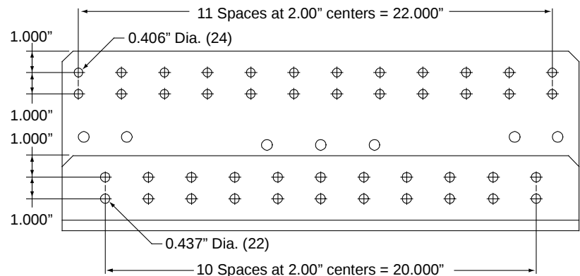
Detail A Positive Battery Busbar Hole Size and Spacing Dimensions (for installation of customer provided two-hole lugs with 3/8" clearance holes on 1" centers)
