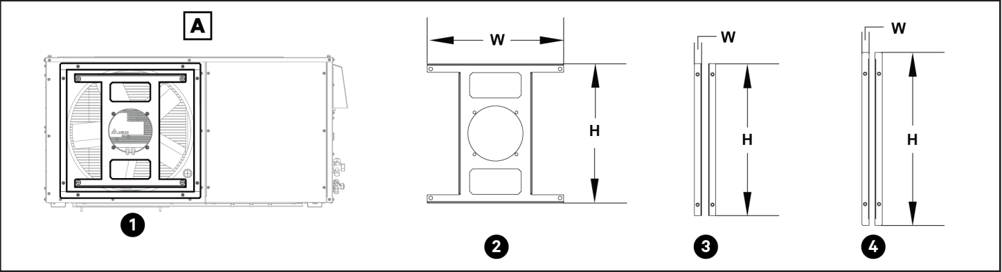
Figure 2. Duct Kit dimensions and location
