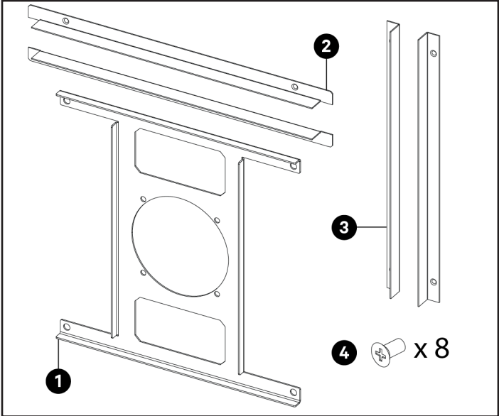
Figure 1. Duct Kit components
