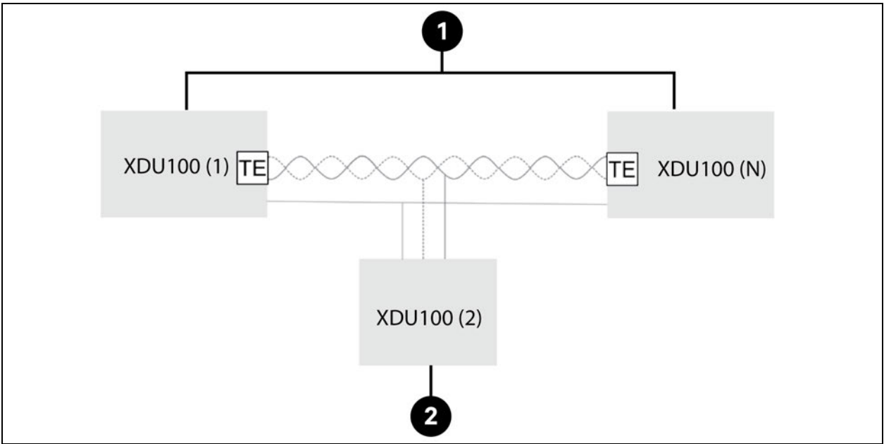
Figure 4.24 CANbus Network Termination Resistors
