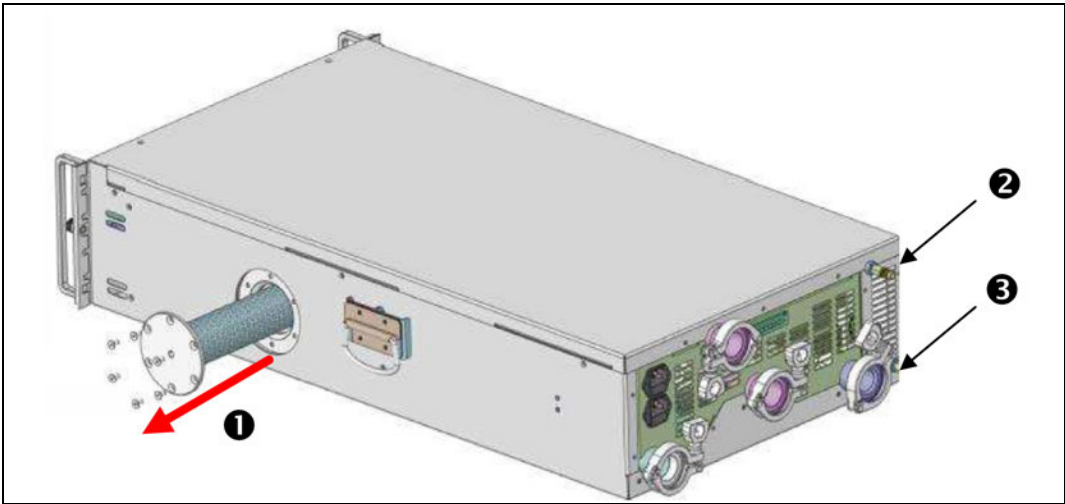
Figure 5.7 Removing the Filter
