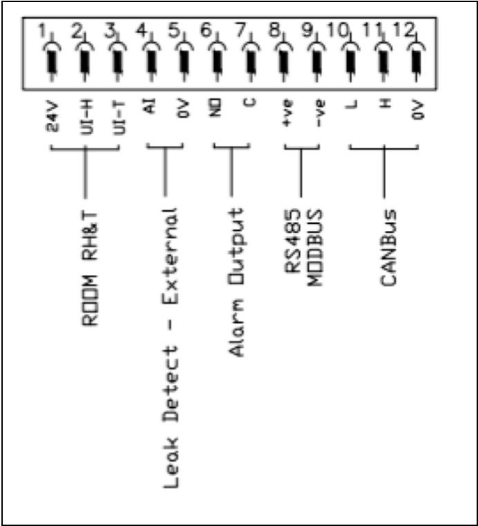
Figure 3.5 Controls Port Mapping (after July 2023)
