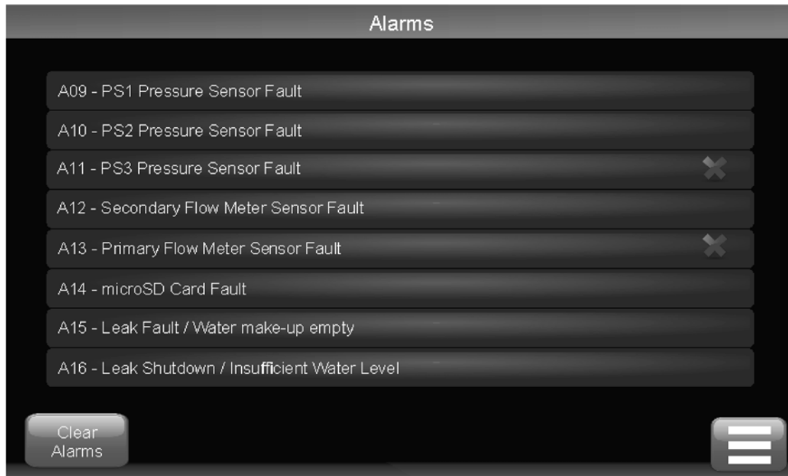
Figure 4.19 Control Screen Alarm identification
