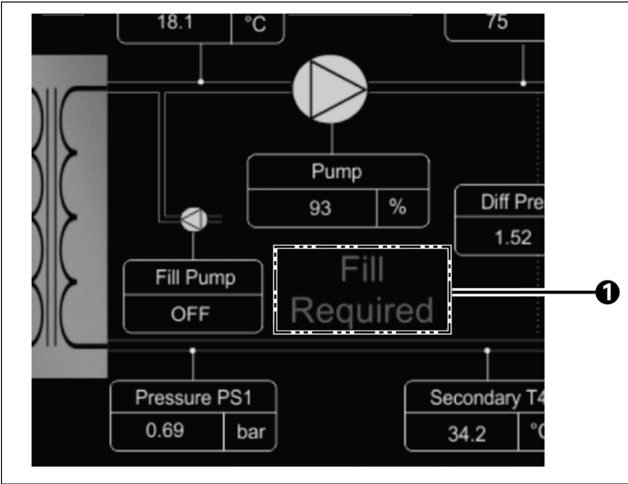
Figure 4.13 Fill Required Request
