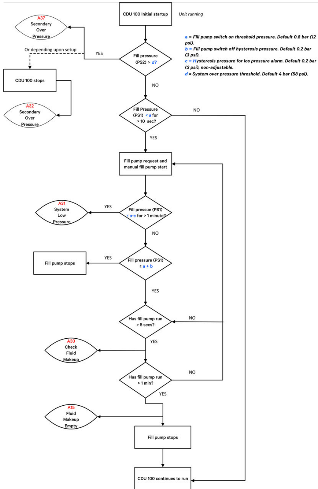
Figure 4.16 Fill Pressure and Level Flow Charge (When Running)
