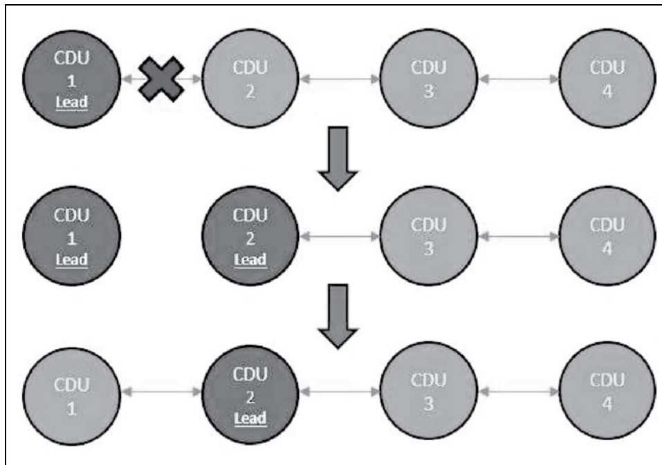
Figure 4.27 Lead Communication Failure
