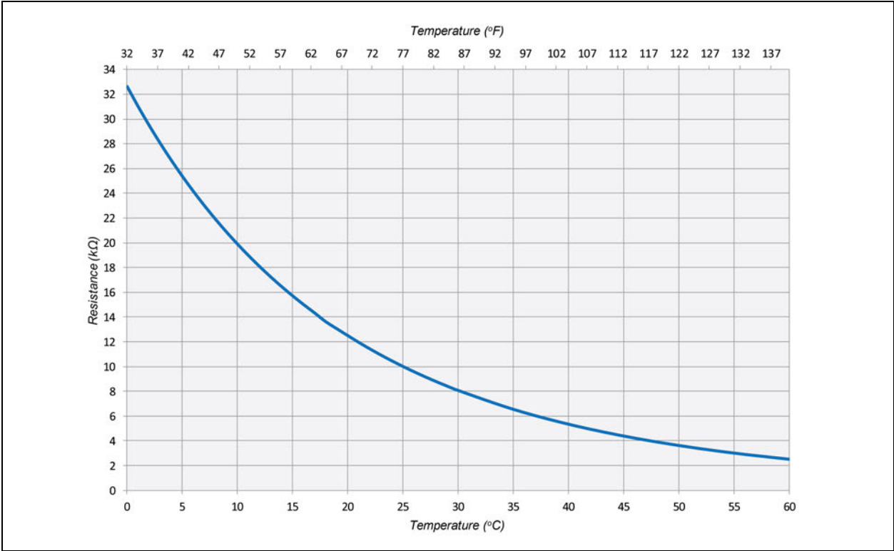
Figure 4.20 Temperature Sensor Resistance Graph
