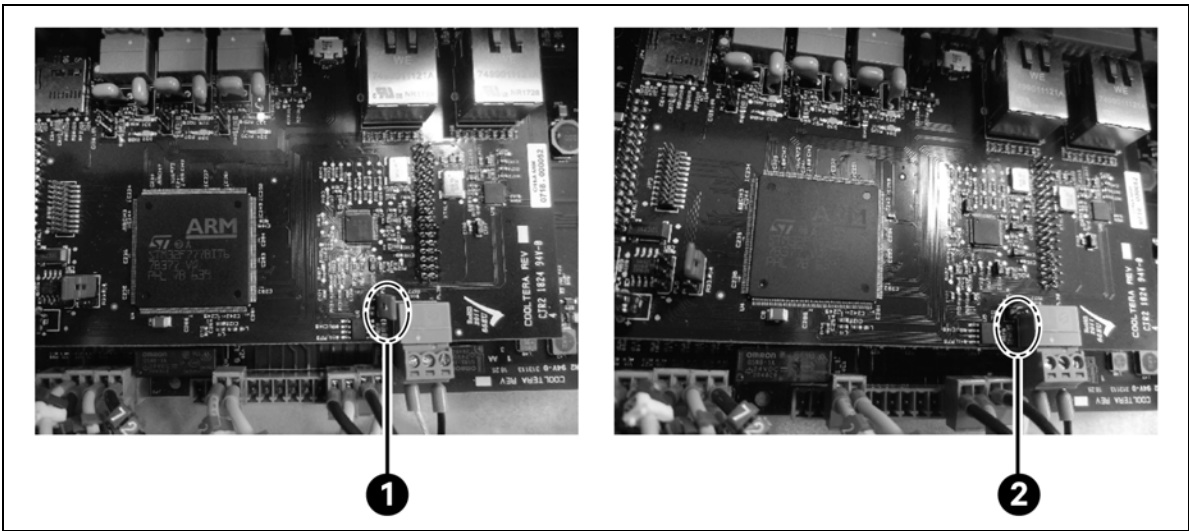
Figure 4.25 CANbus Network Termination Resistors
