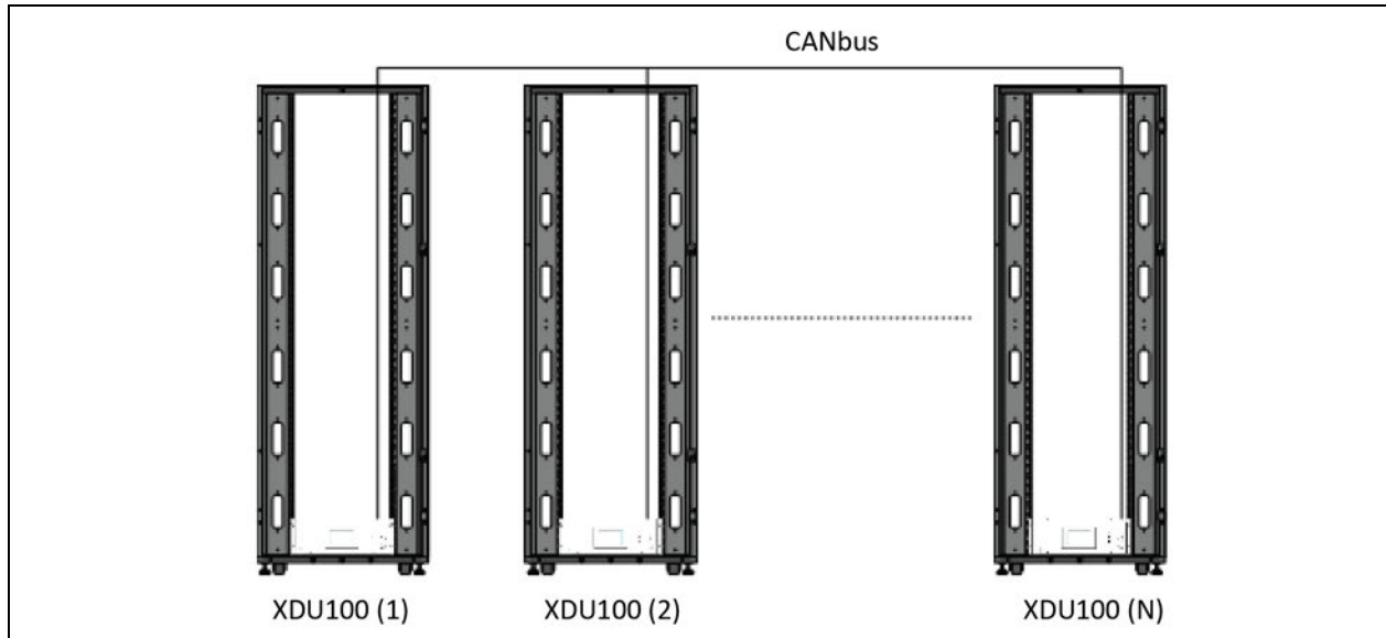
Figure 4.21 Vertiv™ CoolChip CDU 100 Group Control
