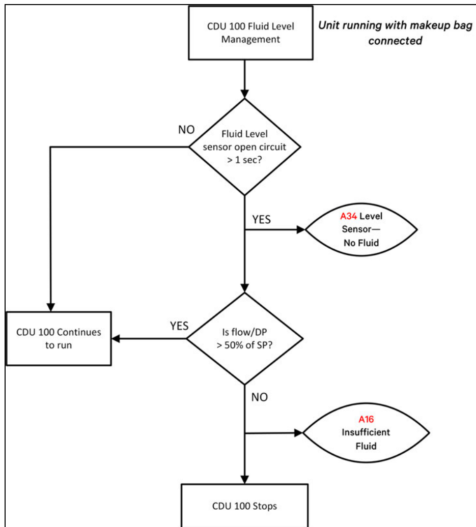
Figure 4.17 Water Level Management (When Running)
