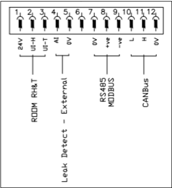
Figure 3.4 Controls Port Mapping (before July 2023)
