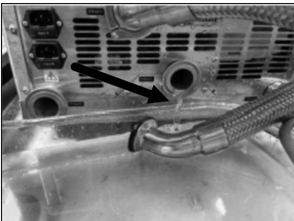
Figure 5.4 Fluid Draining, Removing Primary Hygienic Fitting
