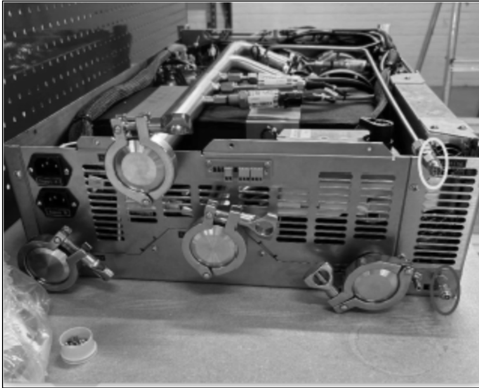
Figure 5.1 Schrader Valve Locations
