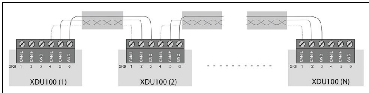
Figure 4.22 Group Control Wiring Configuration
