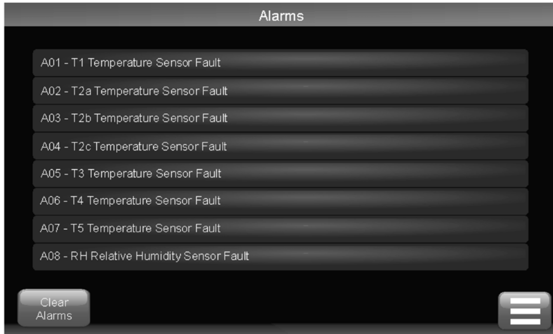
Figure 4.5 Control System Alarms Screen
