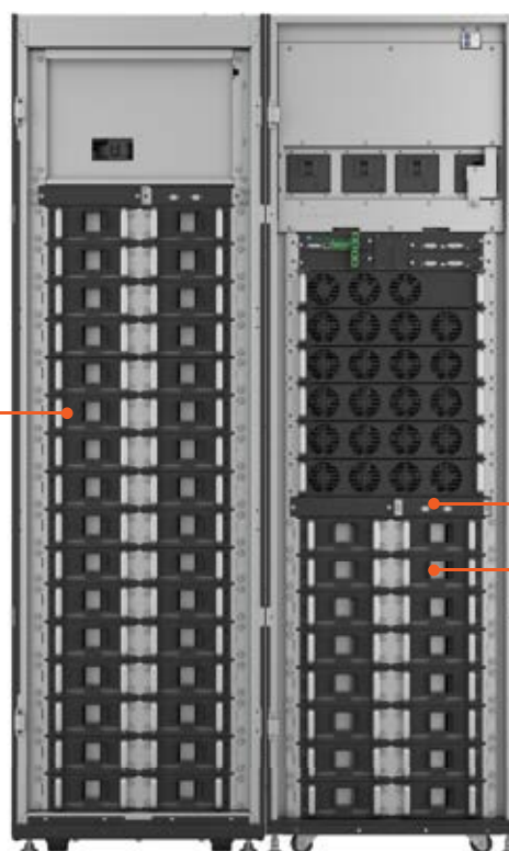
Vertiv™ Liebert® APM2 10-120kW with modular internal VRLA batteries and modular battery cabinet.
