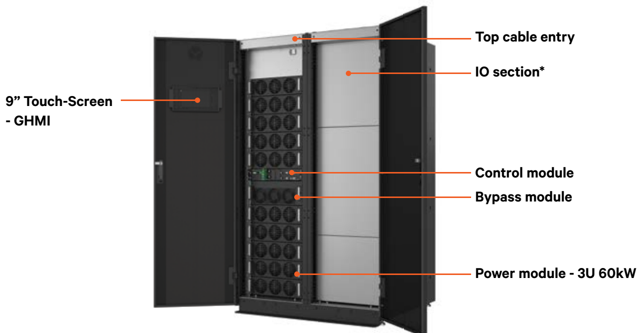
Vertiv™ Liebert® APM2 300-600 kW Compatible with External standard VRLA and Lithium-ion battery cabinets
