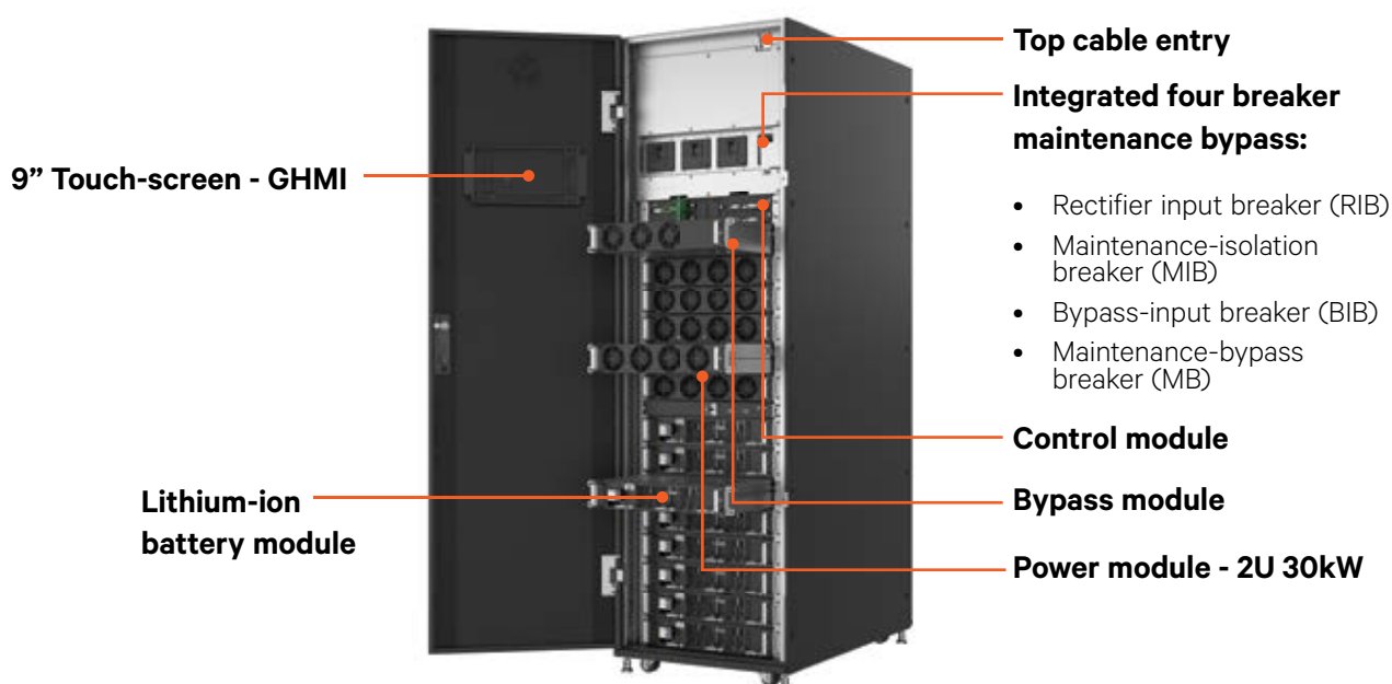
Vertiv™ Liebert® APM2 10-120 kW Compatible with Lithium-ion/VRLA internal modular batteries External modular VRLA, Standard VRLA, and Lithium-ion battery cabinets.
