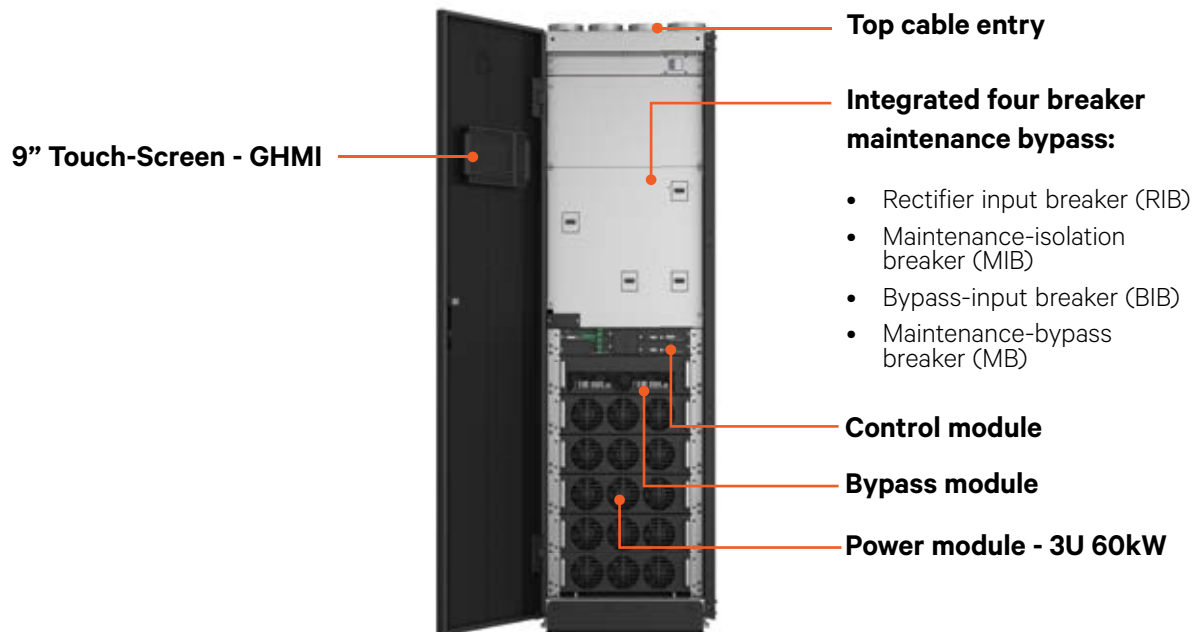
Vertiv™ Liebert® APM2 60-300 kW Compatible with External standard VRLA and Lithium-ion battery cabinets
