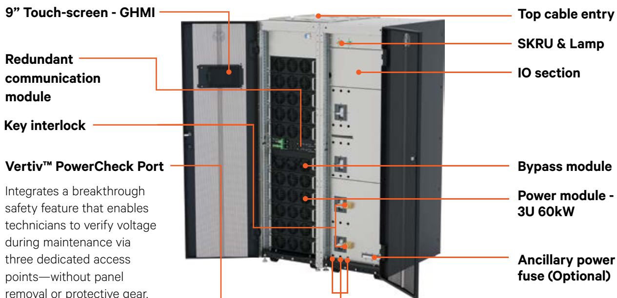
Vertiv™ Liebert® APM2 300-600 kW With Integrated maintenance bypass
