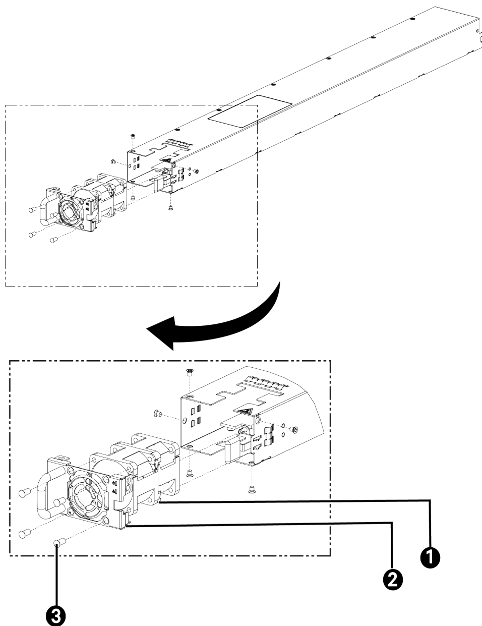
Figure 3.1 Fan Replacement
