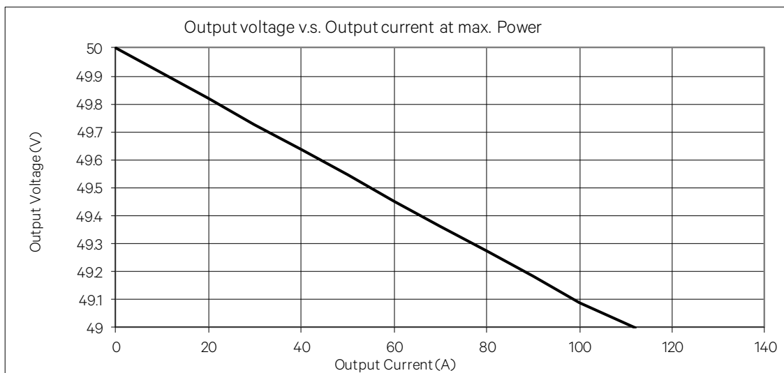
Figure 1.1 Output Voltage vs. Output Current
