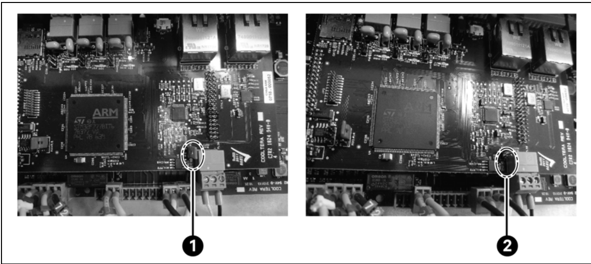
Figure 4.25 CANbus Network Termination Resistors
