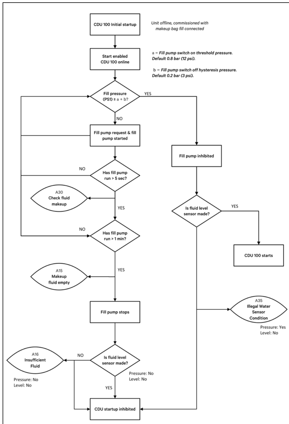
Figure 4.15 Pressure and Level Flow Chart (Initial Startup)
