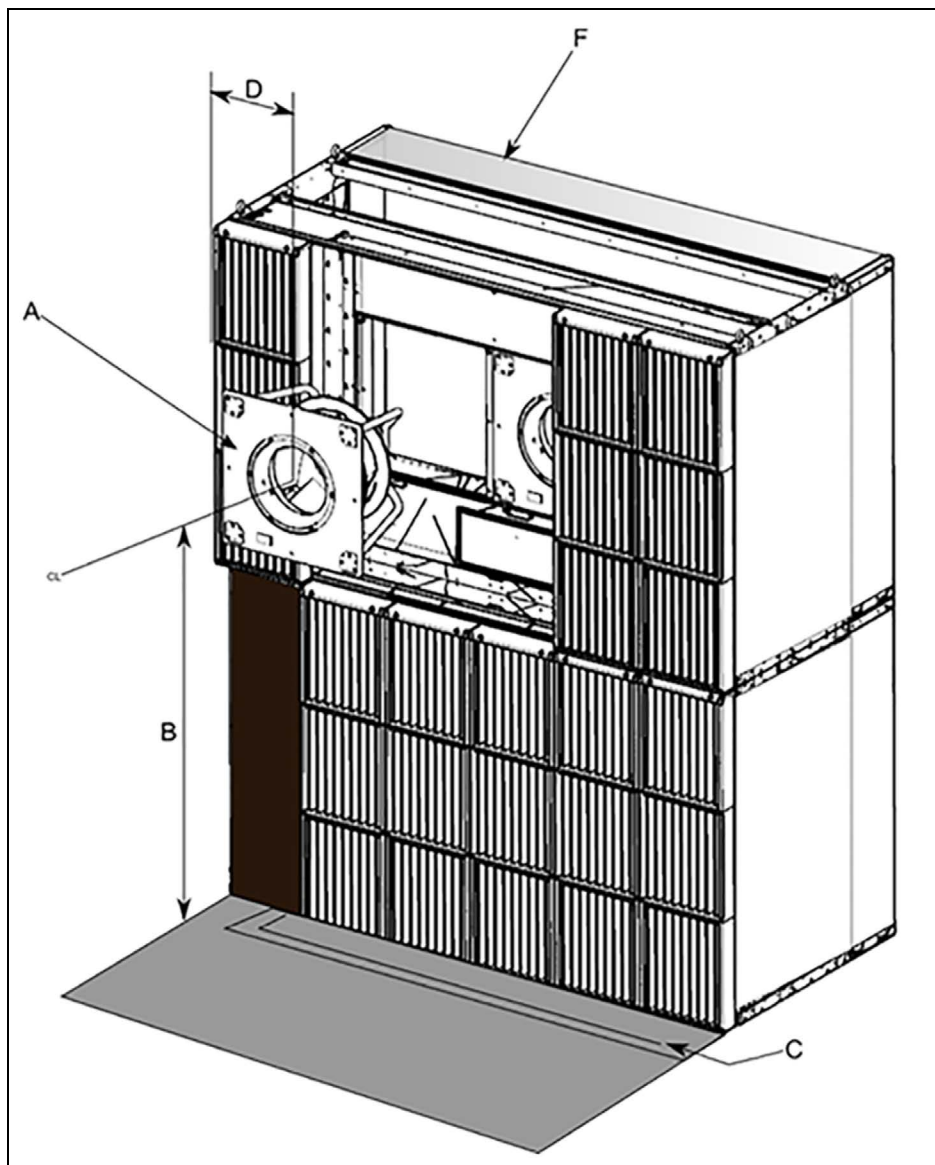
Figure 9.7 Clearance Dimensional Data
