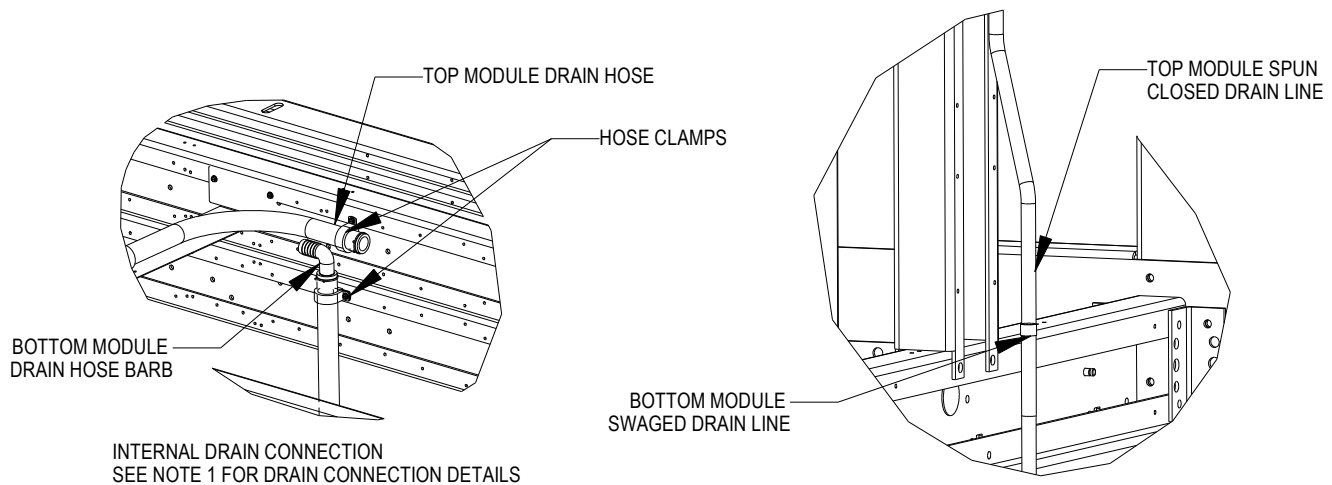
DRAIN LINE ROUTING FRAME SHOWN FOR REFERENCE. SOME MEMBERS HIDDEN FOR CLARITY
