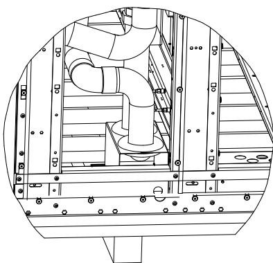
DETAIL B TOP MODULE PIPING BRACKET
