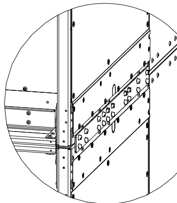
DETAIL C Splice Plate Detail
