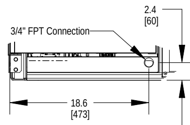
DETAIL B (Field Gravity Condensate Drain Connection)
