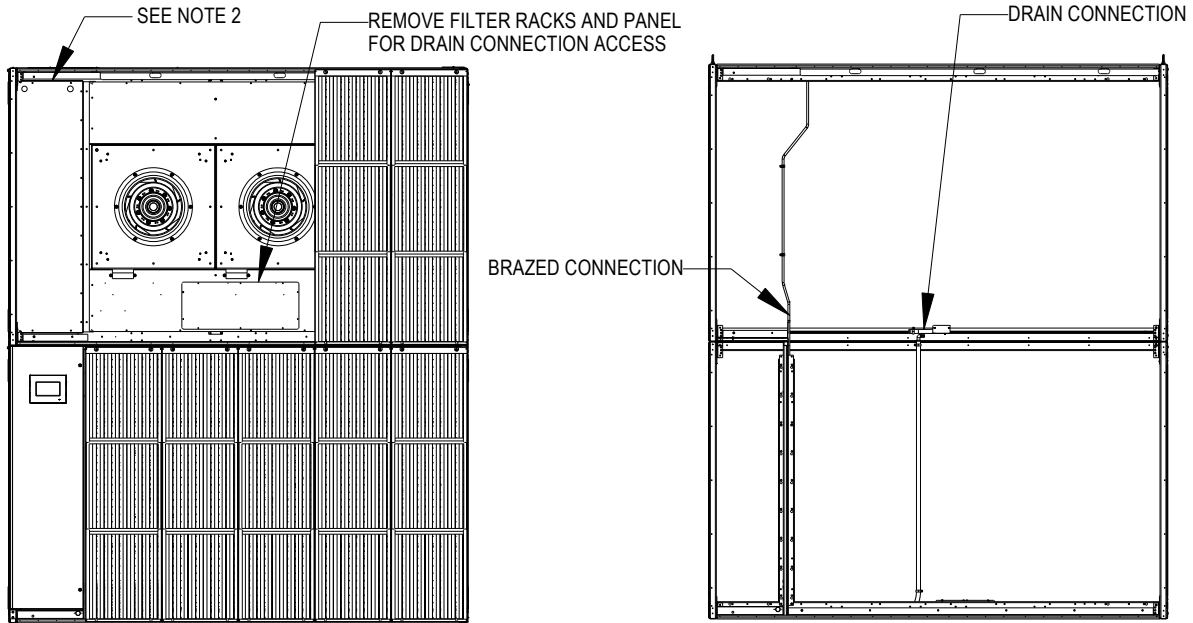
DRAIN LINE ROUTING FRAME SHOWN FOR REFERENCE. SOME MEMBERS HIDDEN FOR CLARITY
