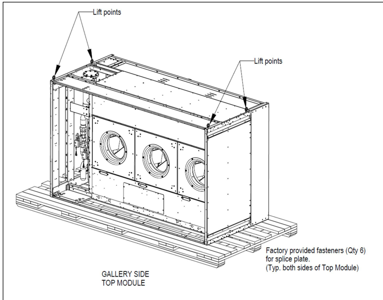
Figure 4.11 Lifting Points
