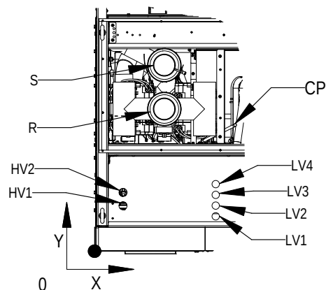
DETAIL A (Chilled Water Field Connection)
