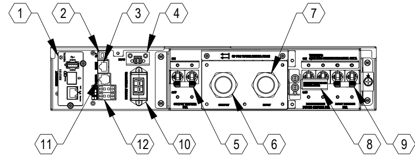
REAR VIEW
