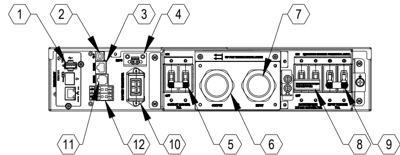
REAR VIEW
