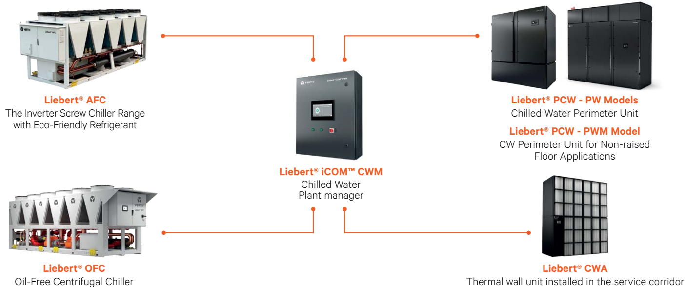
Figure 1. Vertiv's Enlarged Portfolio for a State-of-the-Art Chilled Water System
