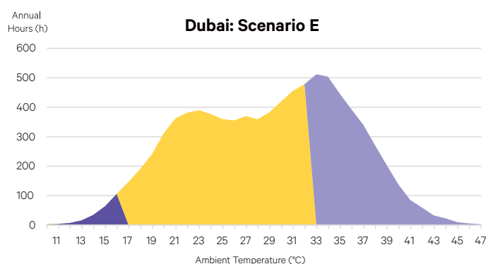
Figure 12. Dubai profile: Including the adiabatic system
