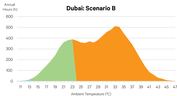
Figure 10. Dubai profile: With increased air and water temperatures
