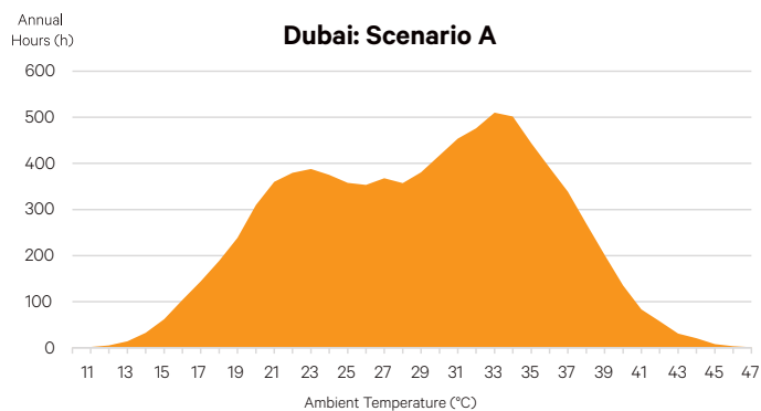
Figure 9. Dubai profile: Traditional Chilled Water System
