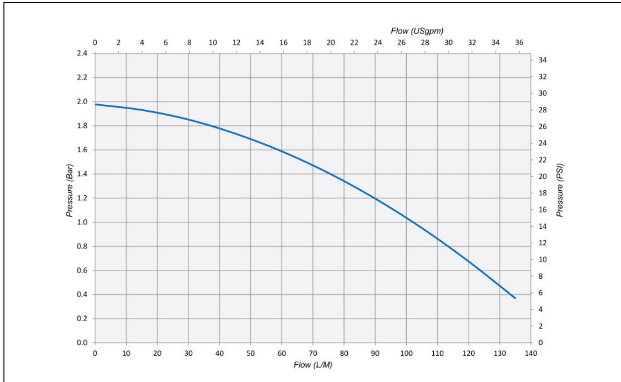
Figure 4.5 Available Secondary External Differential Pressure
