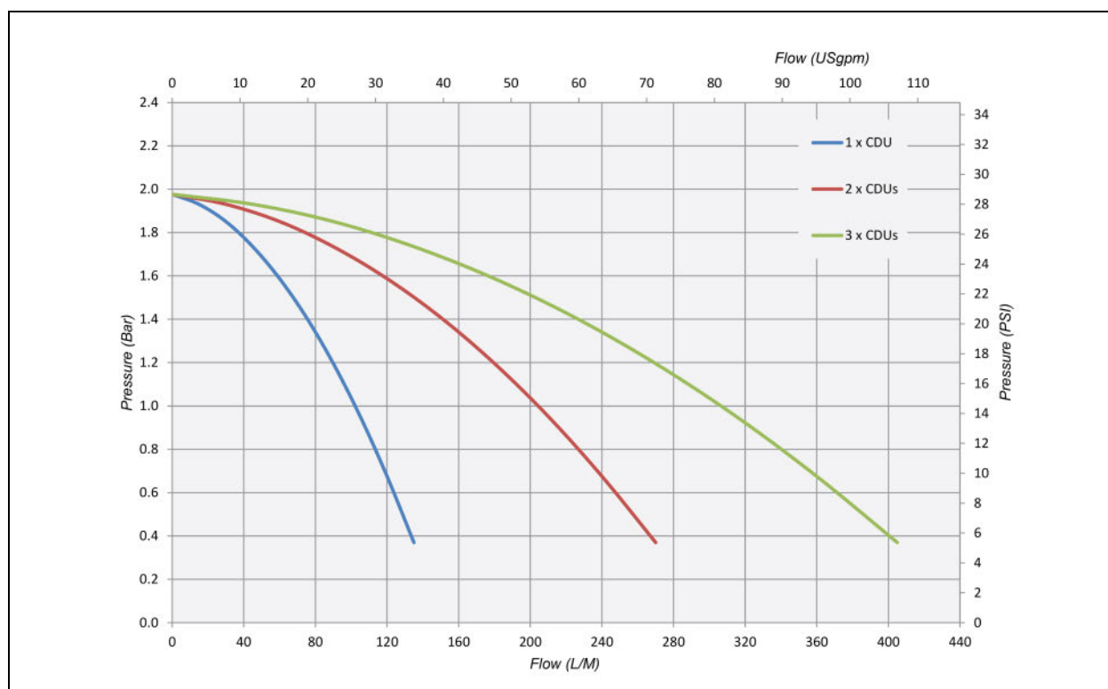
Figure 4.6 Flow and Pressure Graphs for Multiple Units in Parallel
