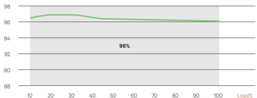
S48-2000e3 Efficiency Curve at 420 VDC Nominal
