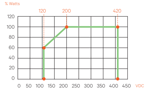
Figure 1: Output Power vs. Input Voltage at Temperature < 55°C
