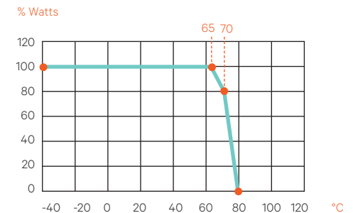
Figure 3: Output Power vs. Temperature at 420VDC > Vin > 200VDC
