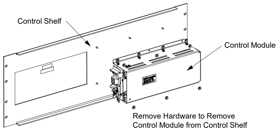
Figure 1.3 Temporarily Removing Control Module
