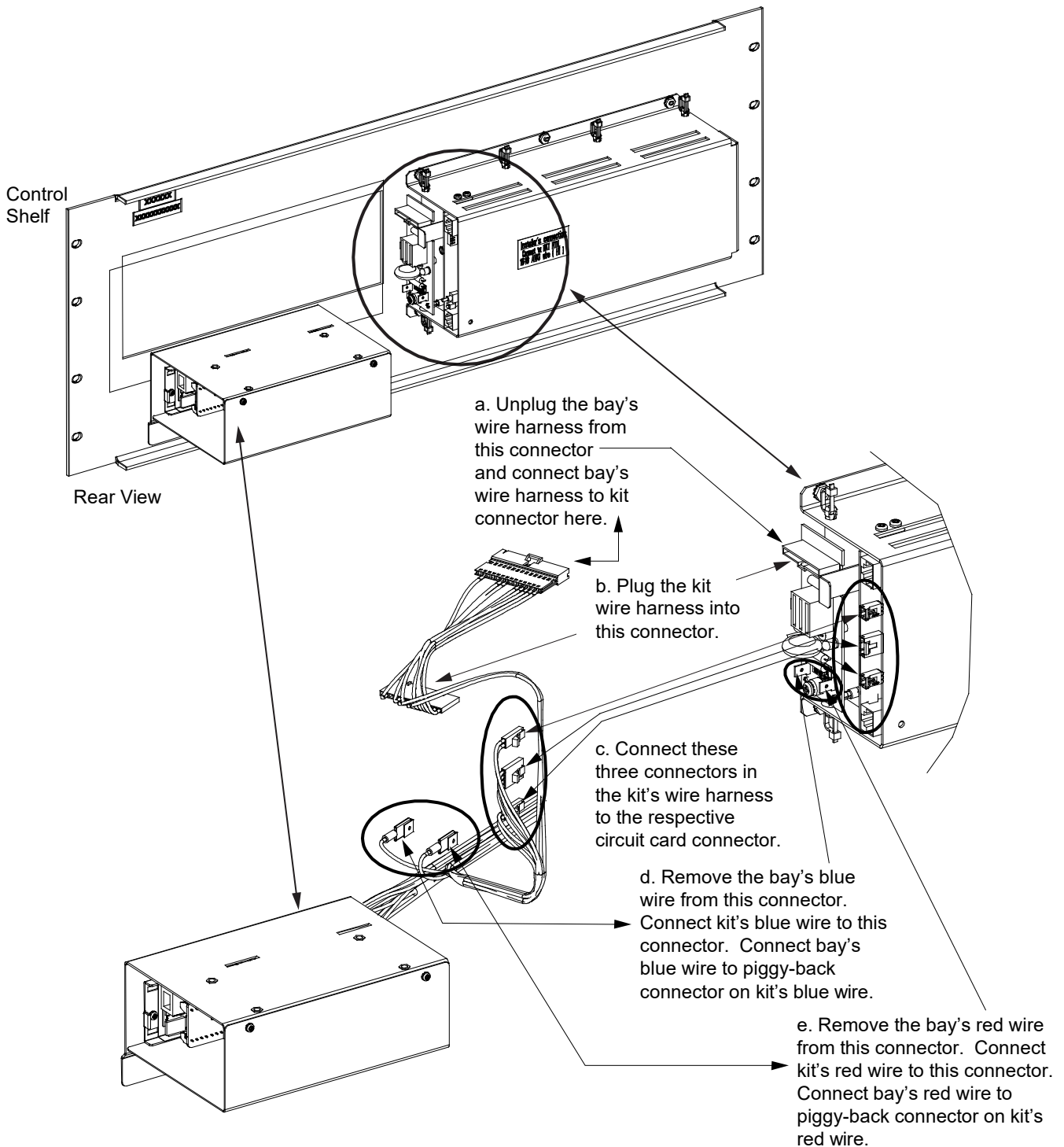
Figure 1.10 Connect Wire Harness Cables
