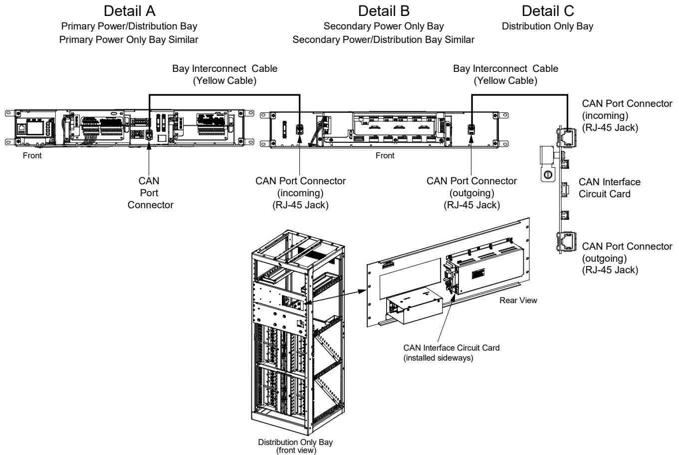
Figure 1.11 Connect Network Cable(s)
