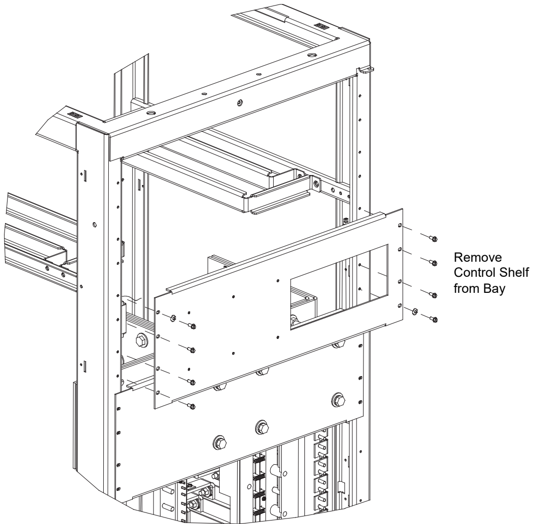
Figure 1.4 Removing Control Shelf
