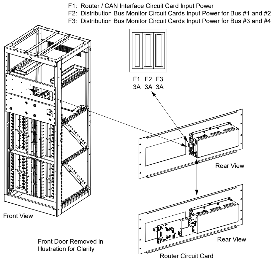
Figure 1.9 Distribution Only Bay Router Circuit Card Replacement and Fuse Location
