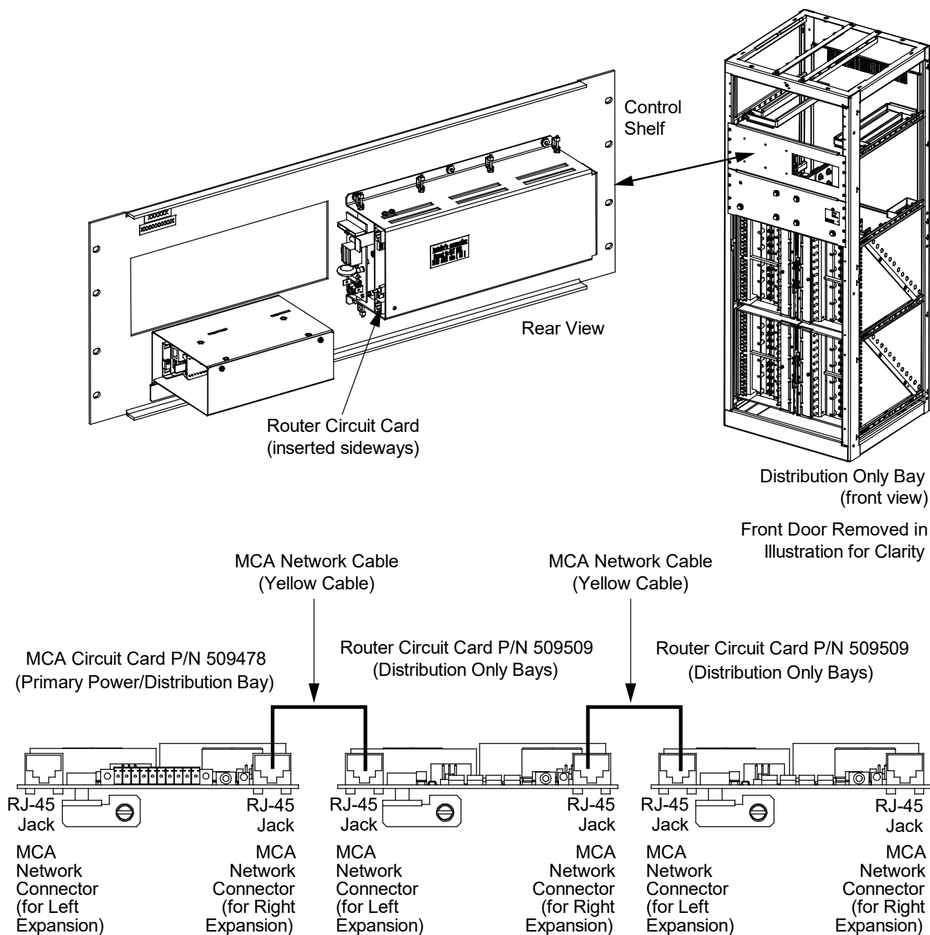
Figure 1.8 Disconnect MCA Network Cable(s)
