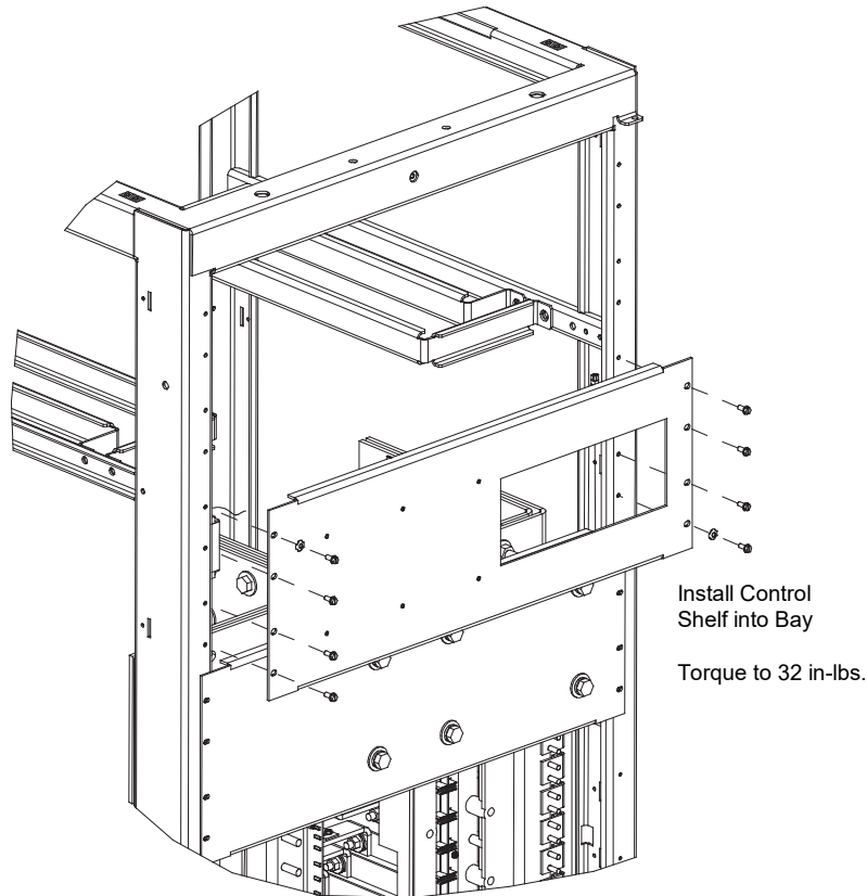
Figure 1.6 Installing the Kit Furnished Control Shelf
