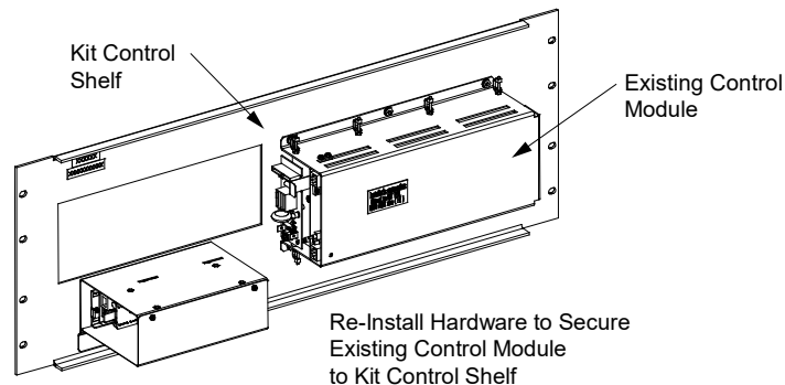
Figure 1.7 Installing Existing Control Module to Kit Control Shelf
