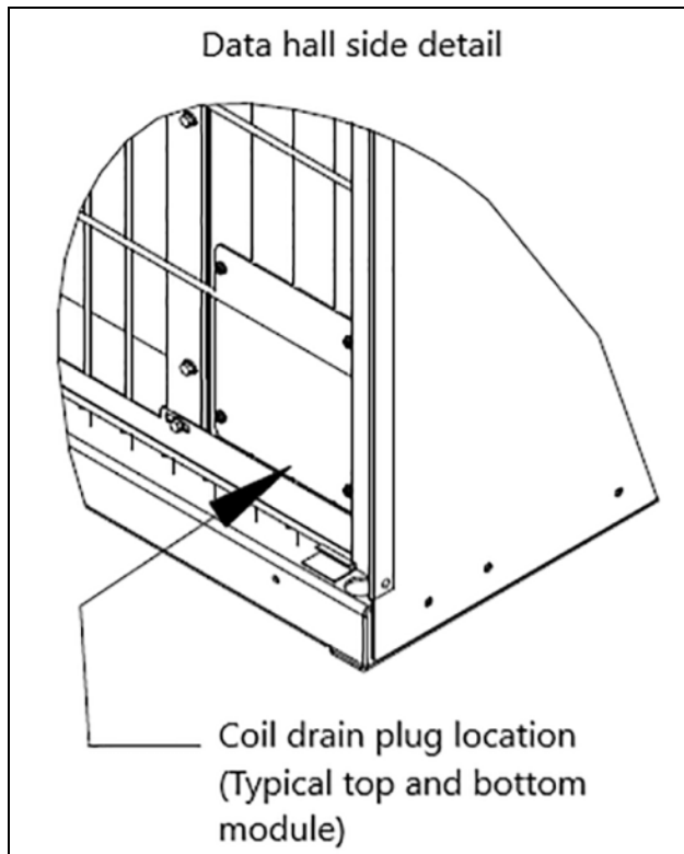
Figure 9.10 Coil Drain Plug Detail
