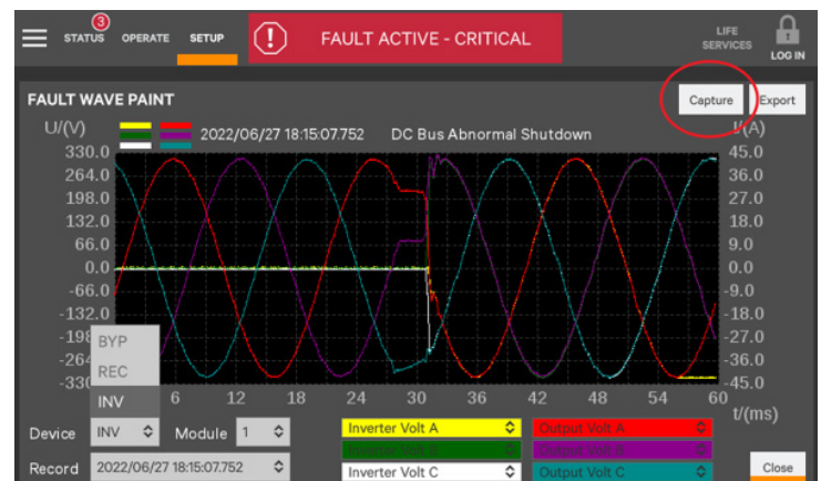
Fault wave recorder feature on PowerUPS 9000 HMI
