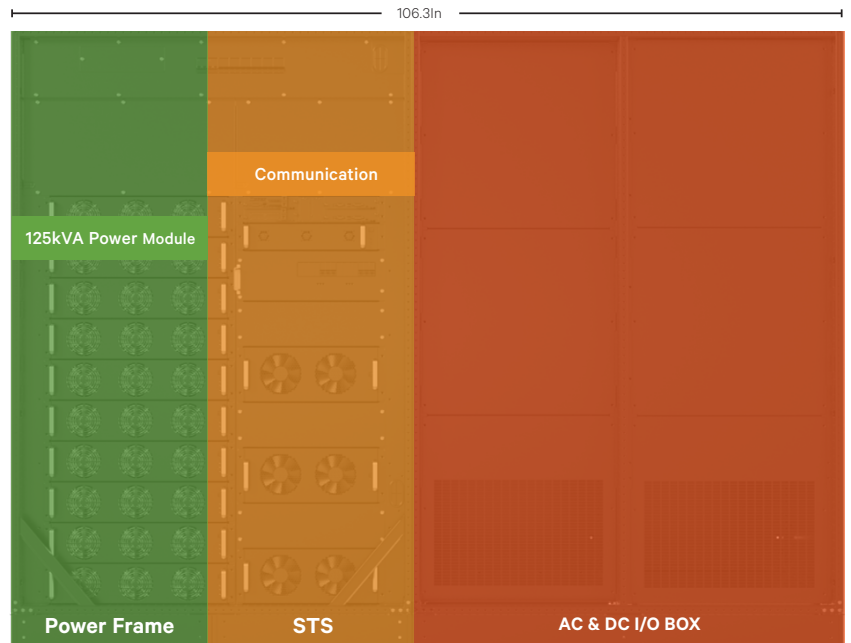
1.25MW 415Vac 4W UL Vertiv™ PowerUPS 9000
