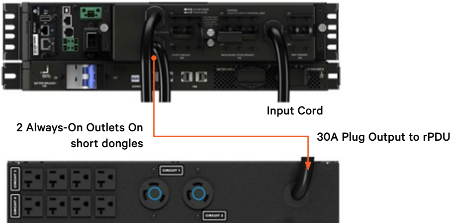
VP0N3202 rPDU
