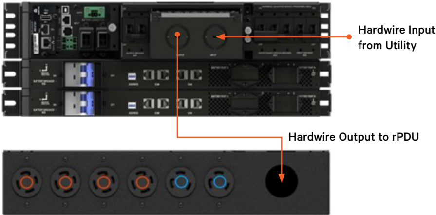
VP0N6202 rPDU
