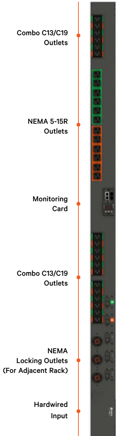
Vertiv™ Liebert® VP4N6003 Vertical rPDU
