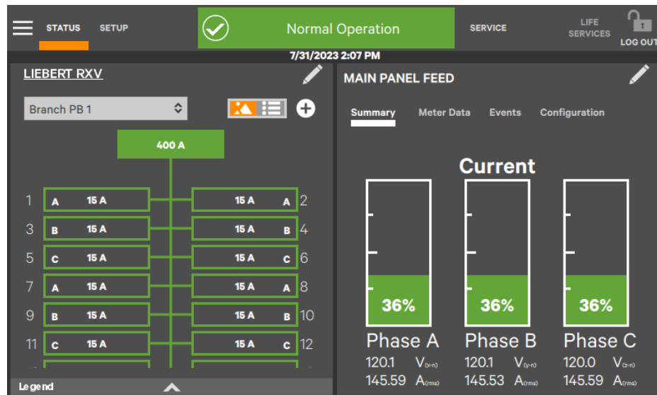
Figure 2. The Vertiv™ Liebert® RXV unit's One-line electrical diagram displays the current status of the main and branch panel breakers. The Summary panel displays the unit's total load and individual phase currents.
