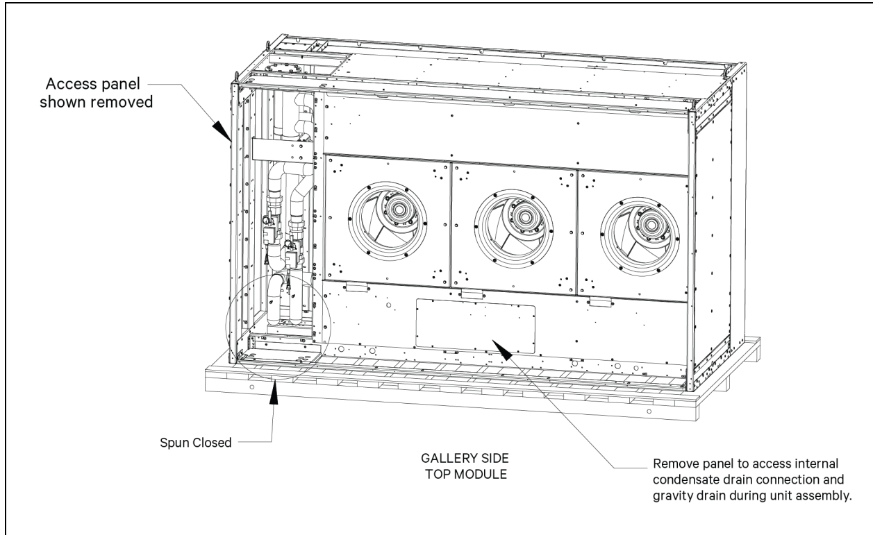
Figure 4.7 Gallery Side Top Module
