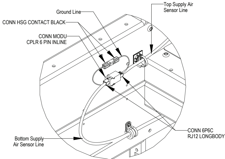
DETAIL D Supply Air Sensors Interconnection (Bottom and Top)
