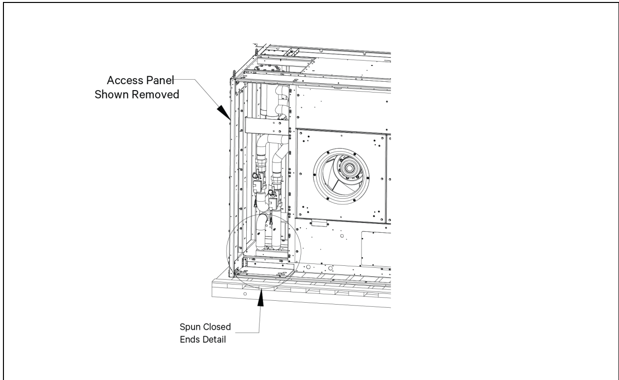
Figure 4.2 Gallery Side, Top Module Piping Access to Internal Supply and Return Piping Connections
