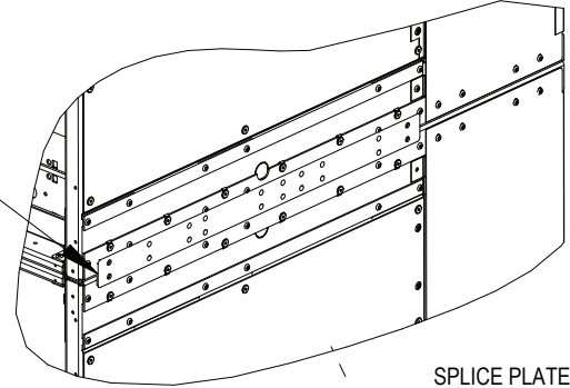
SPLICE PLATE DETAIL
