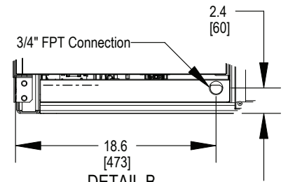
DETAIL B (Field Gravity Condensate Drain Connection)
