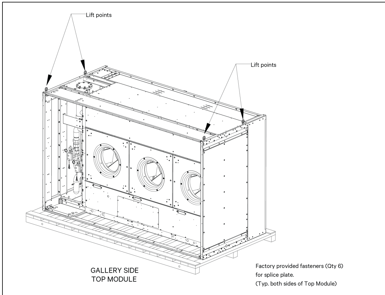
Figure 4.11 Lifting Points
