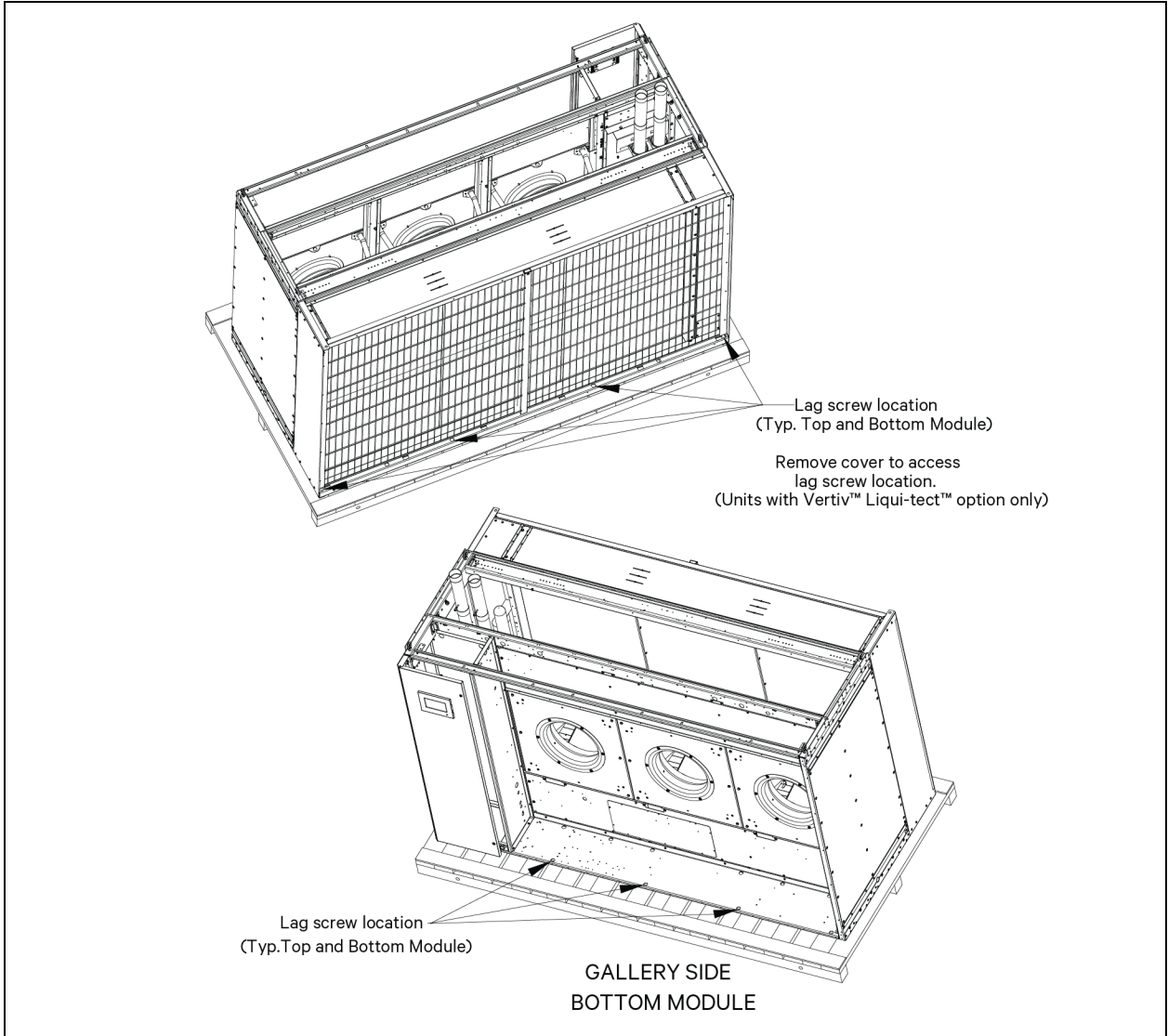
Figure 4.10 Lag Screw Removal
