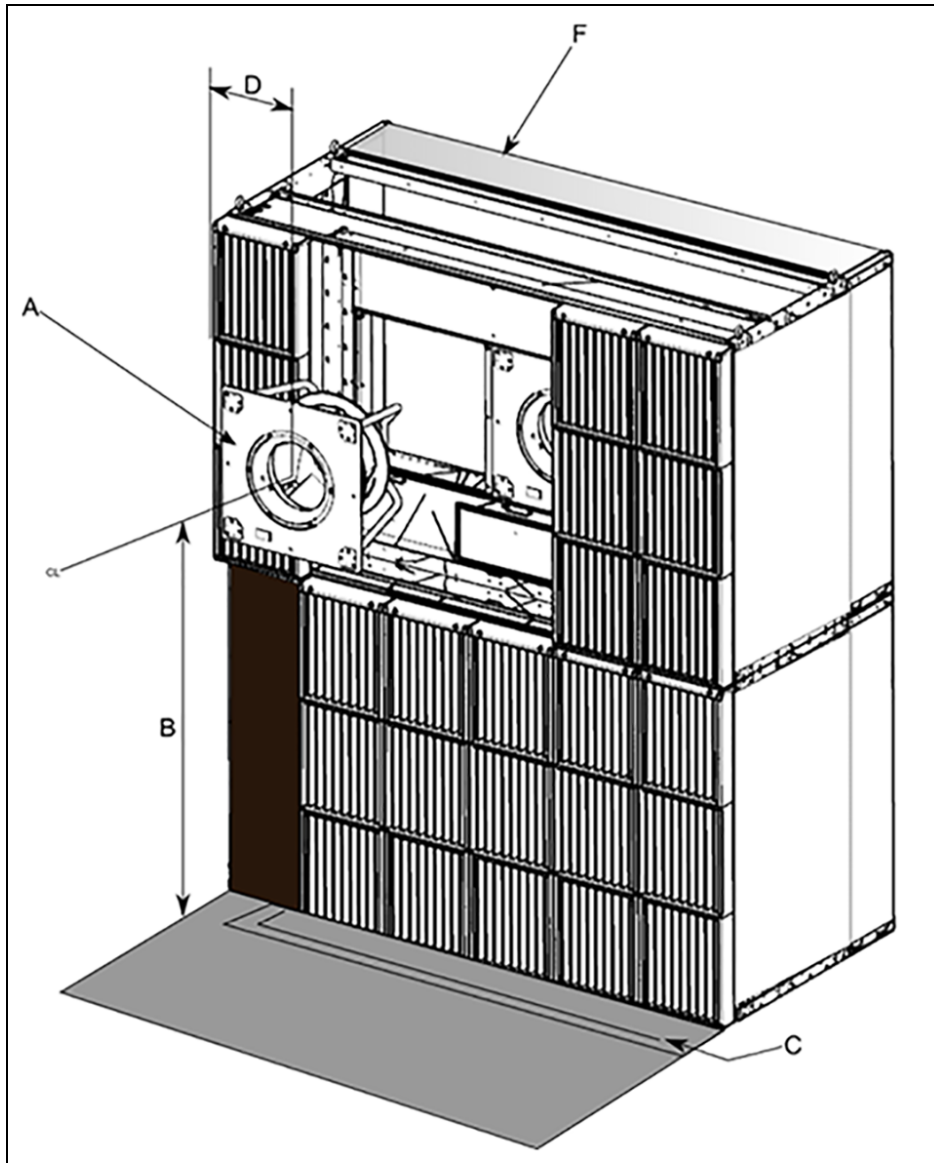
Figure 9.7 Clearance Dimensional Data
