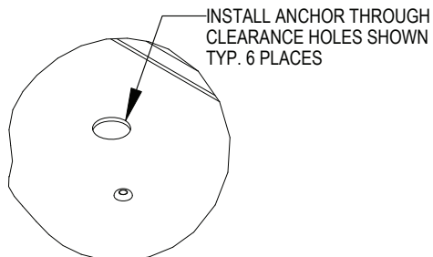
DETAIL A CLEARANCE HOLES FOR SEISMIC BOLTS TYP. 6 PLACES
