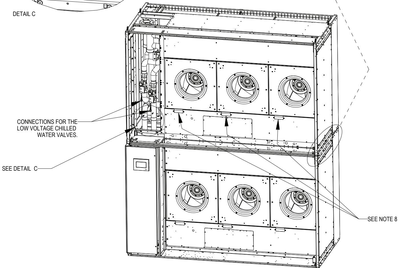
SPLICE PLATE DETAIL
