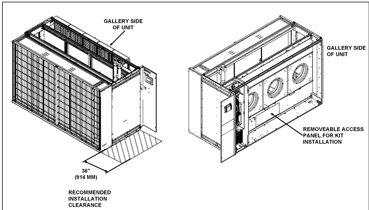
Figure 4.9 Installation Clearance
