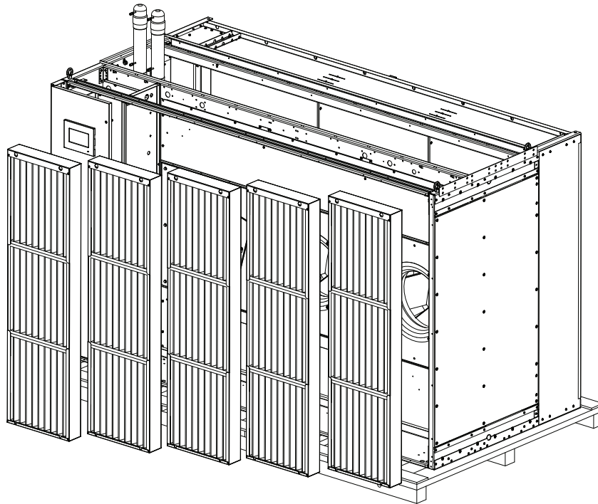
GALLERY SIDE BOTTOM MODULE
