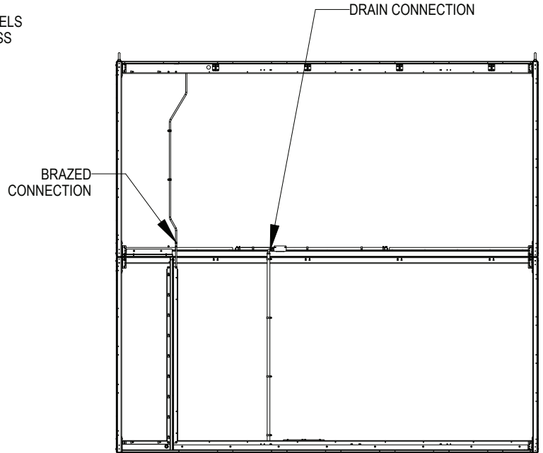
DRAIN LINE ROUTING FRAME SHOWN FOR REFERENCE. SOME MEMBERS HIDDEN FOR CLARITY
