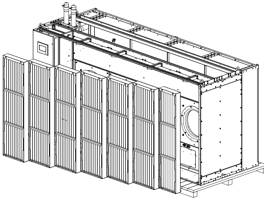
GALLERY SIDE BOTTOM MODULE
