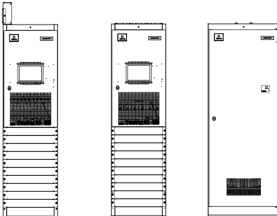
Primary Power/Distribution Bay Secondary Bay Similar
