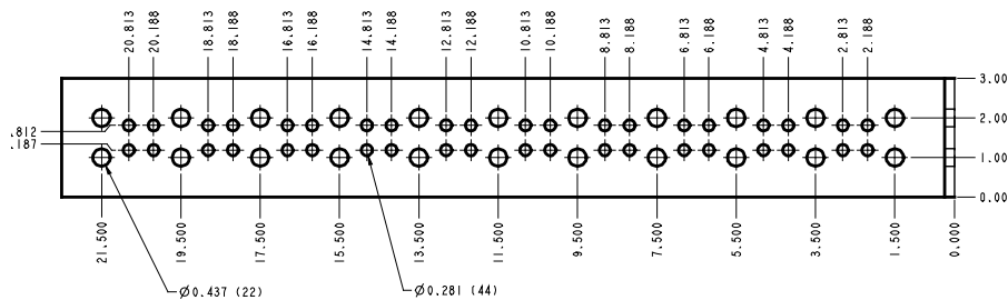
Internal Ground Busbar Assembly P/N 555214
