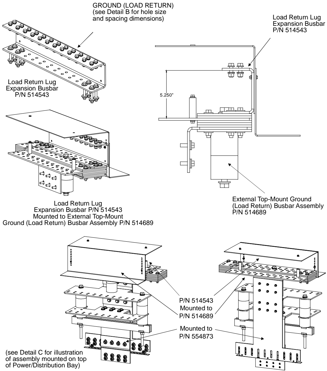
Load Return Lug Extension Busbar P/N 514543 (mounts to External Top-Mount Ground [Load Return] Busbar Assembly)
