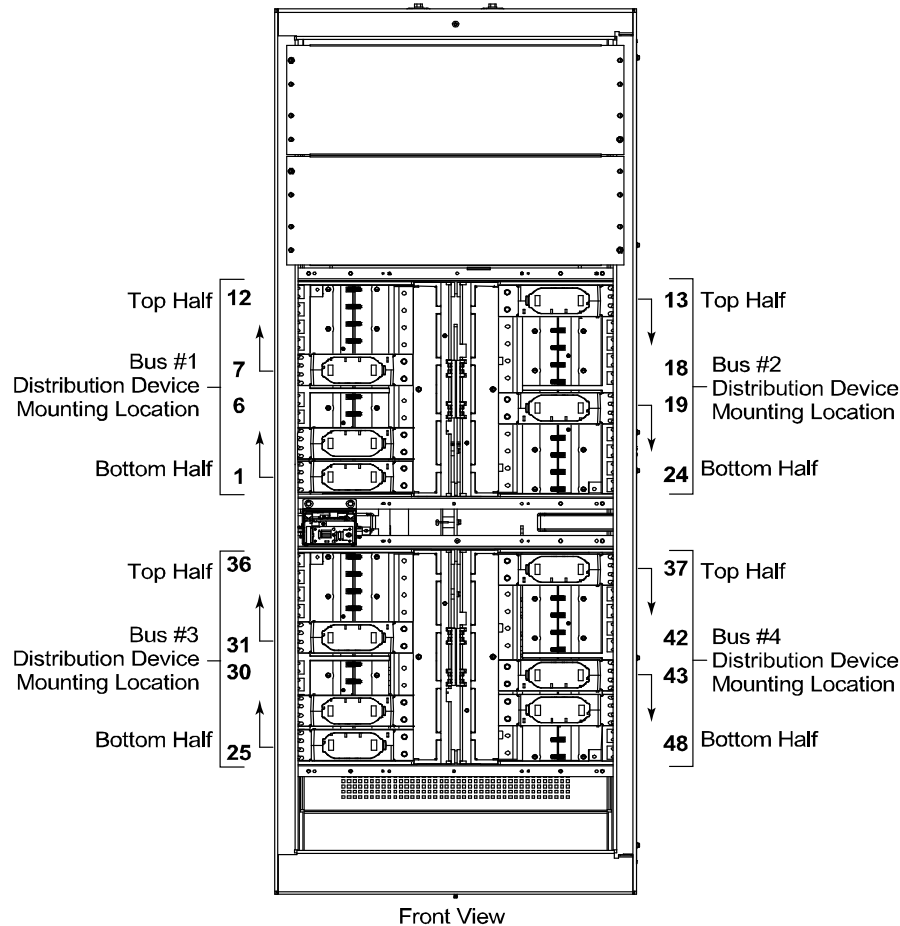
Front View Door removed in illustration for clarity.
