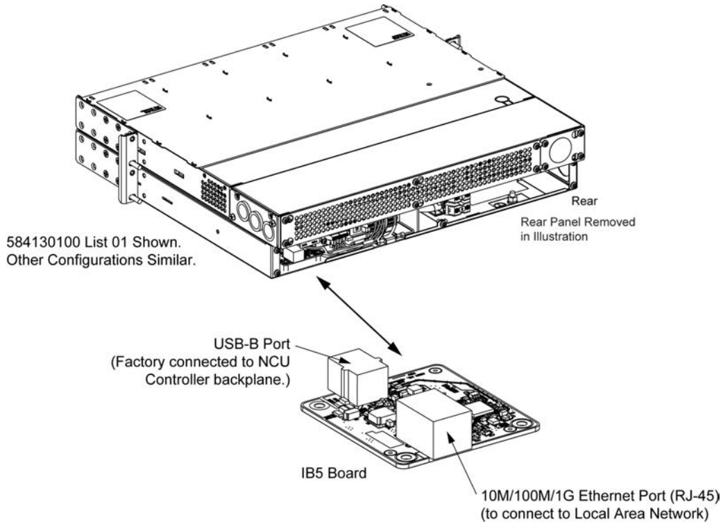
Figure 10 IB5 Board Ethernet Port (for connection into a customer's network)
