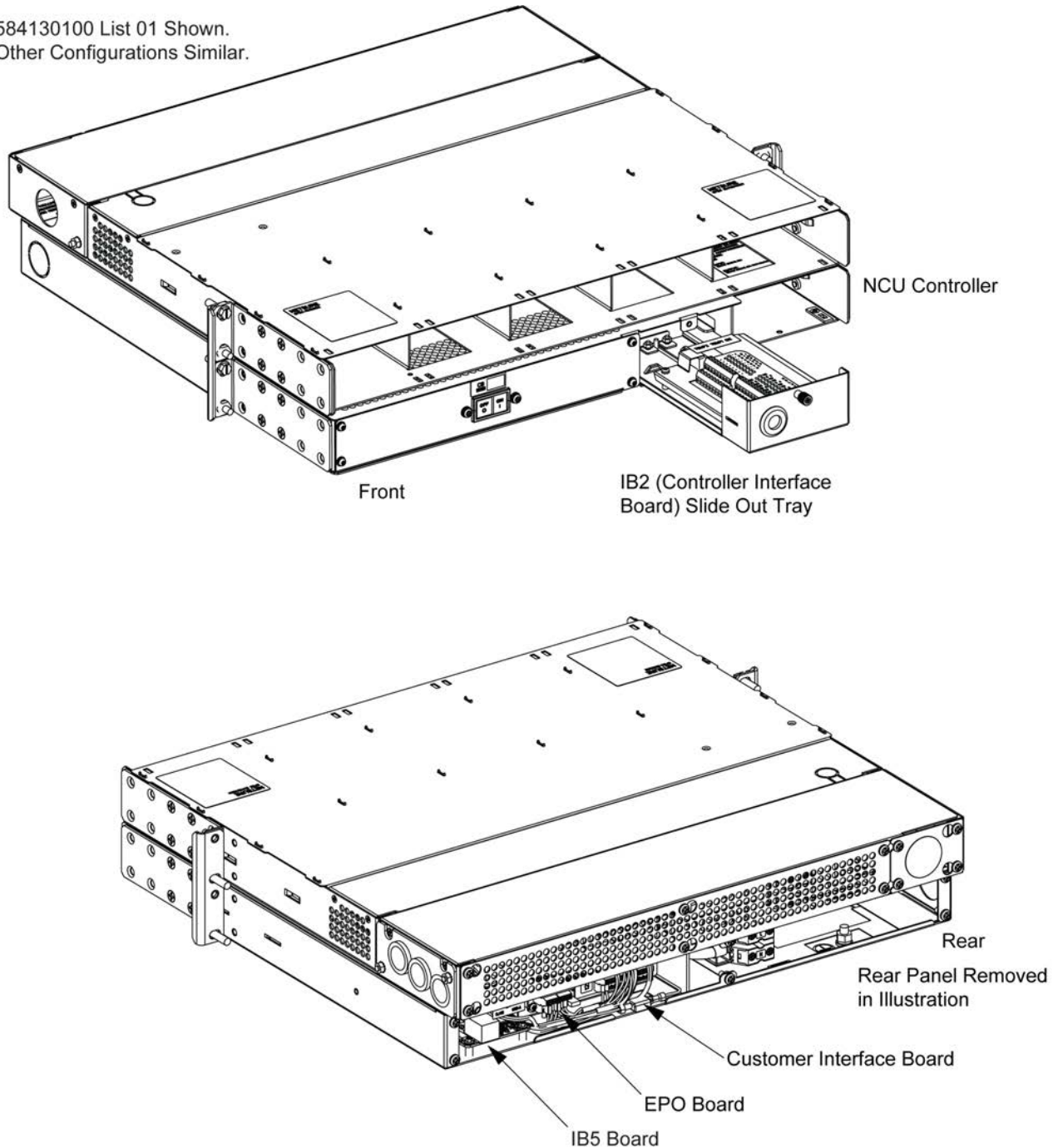
Figure 6 External Alarm, Reference, Monitoring, and Control Connections Locations
