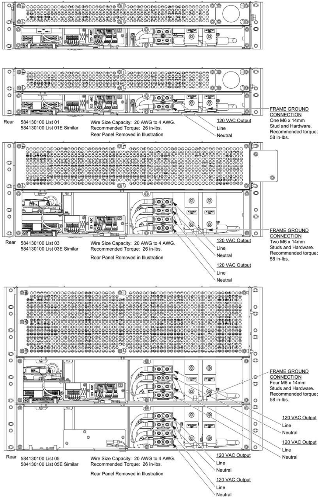
Figure 4 AC Output Connections (List 01, 01E, 03, 03E, 05 and 05E)
