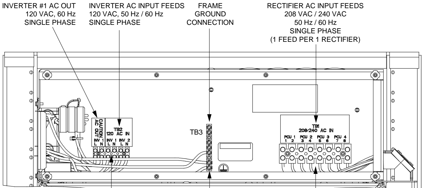
Front (front cover removed)
