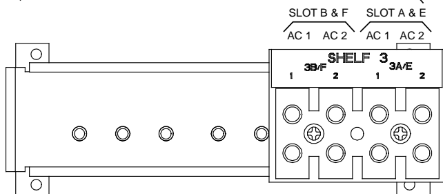
DUAL RECTIFIER (PCU) AC INPUT FEEDS 208-240VAC, 50/60Hz, SINGLE PHASE
