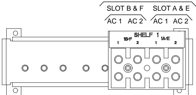
DUAL RECTIFIER (PCU) AC INPUT FEEDS 208-240VAC, 50/60Hz, SINGLE PHASE
