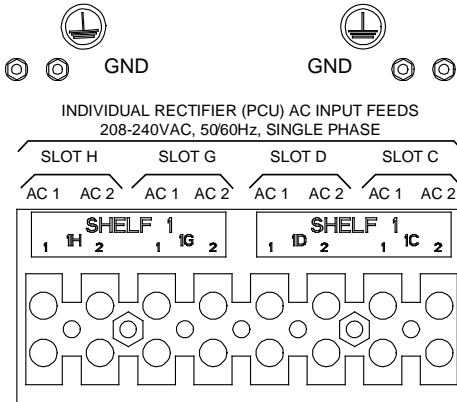
Inside View Right Side
