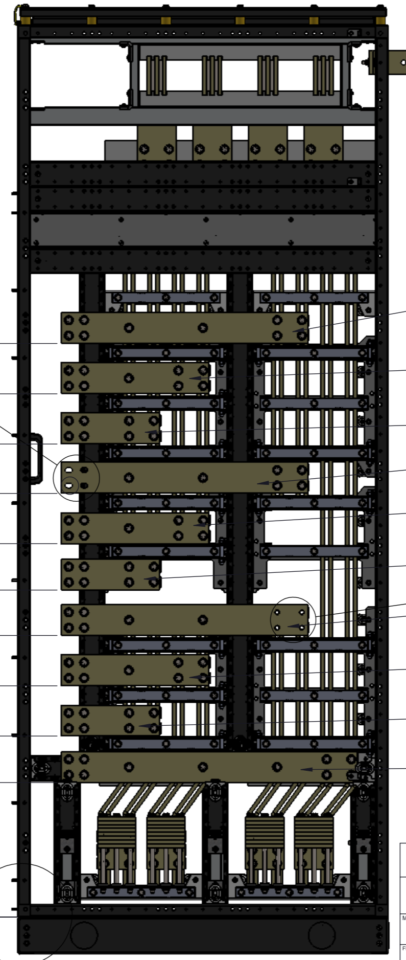
FRONT VIEW
