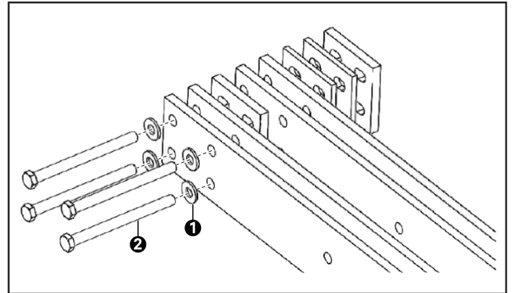
Figure 9 Exploded View of Busbar/Packer/Bolt Arrangement
