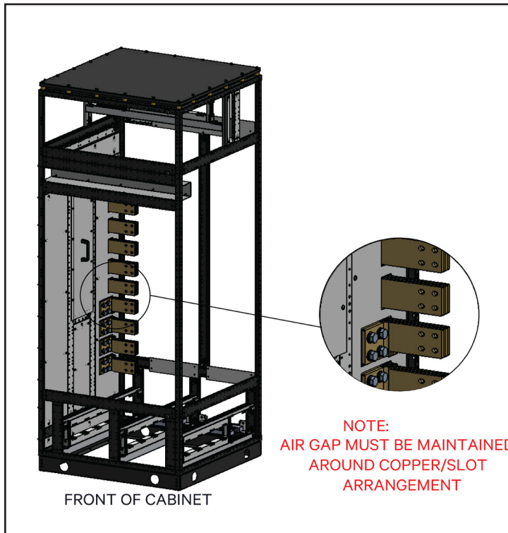
Figure 11 L-shaped Copper Busbar in Segregation Slots
