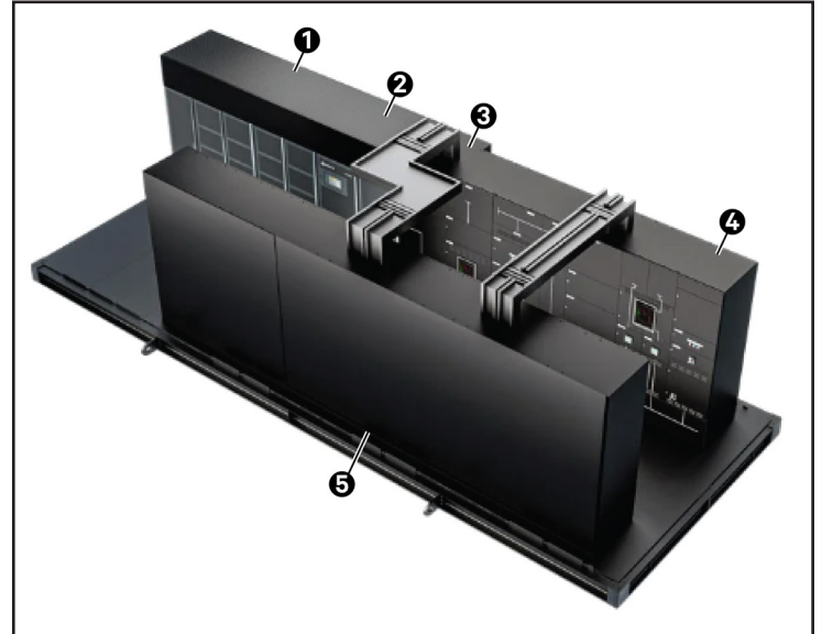
Figure 2 Example of Front-to-Front Layout
