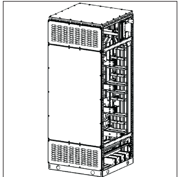
Figure 3 I/O Box - Back-to-Back
