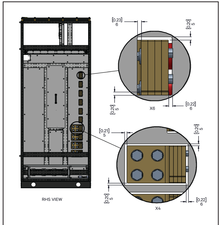
Figure 12 Clearance of Segregation Slots
