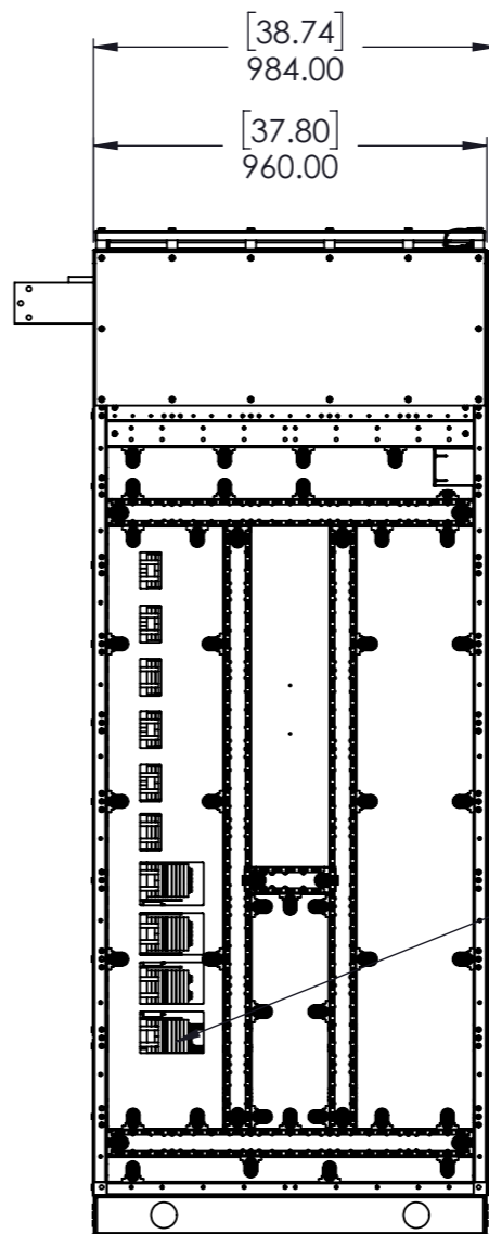
LHS VIEW
