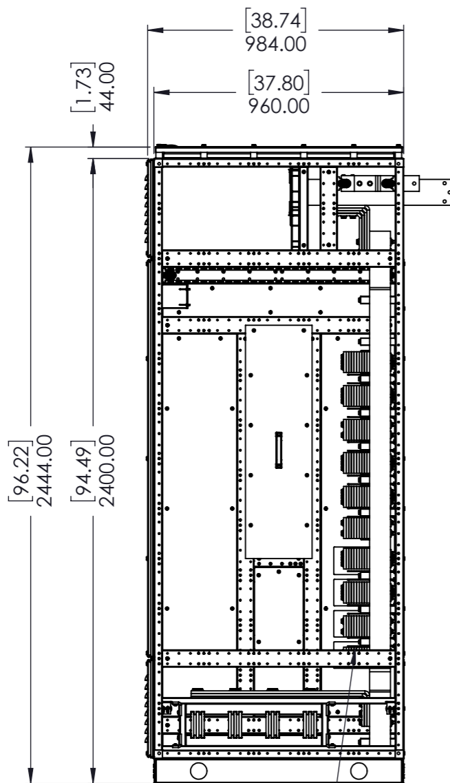
RHS VIEW
