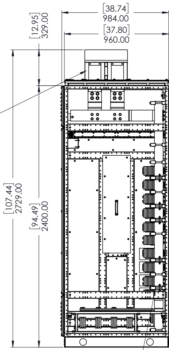
RHS VIEW
