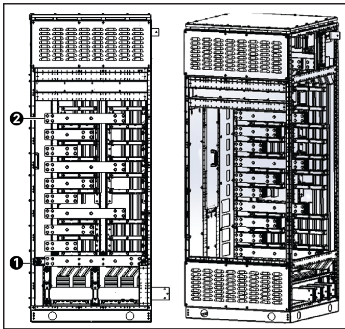
Figure 7 I/O Box Interface Connections
