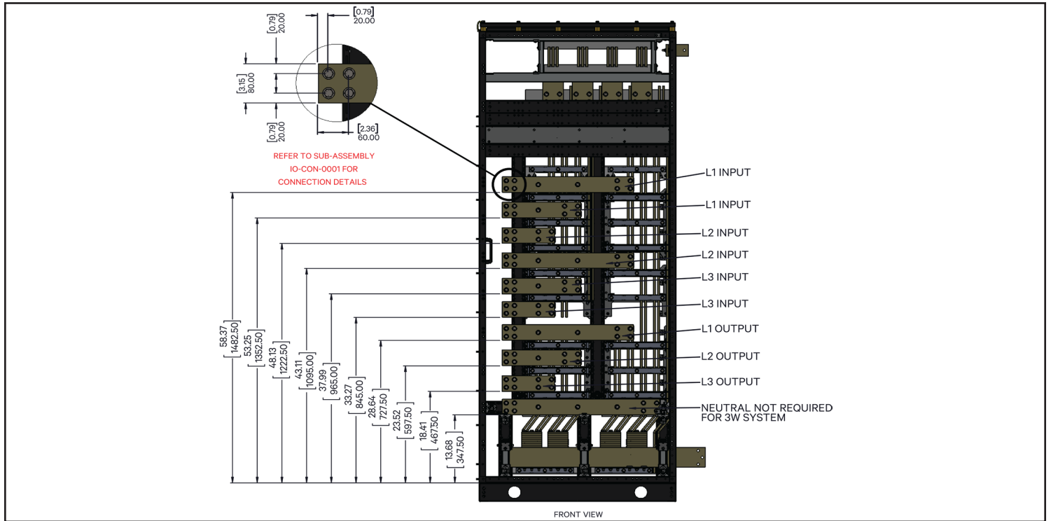
Figure 10 Height of Connecting Busbar from Datum Points
