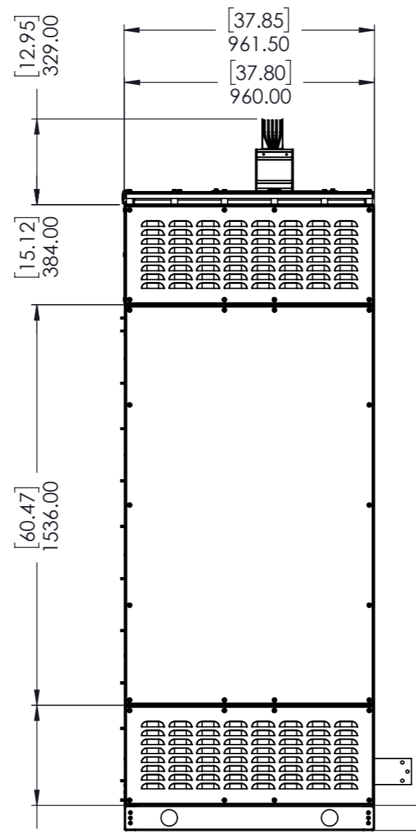
FRONT VIEW
