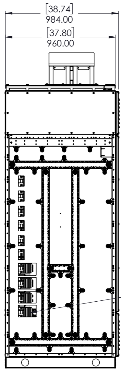
LHS VIEW
