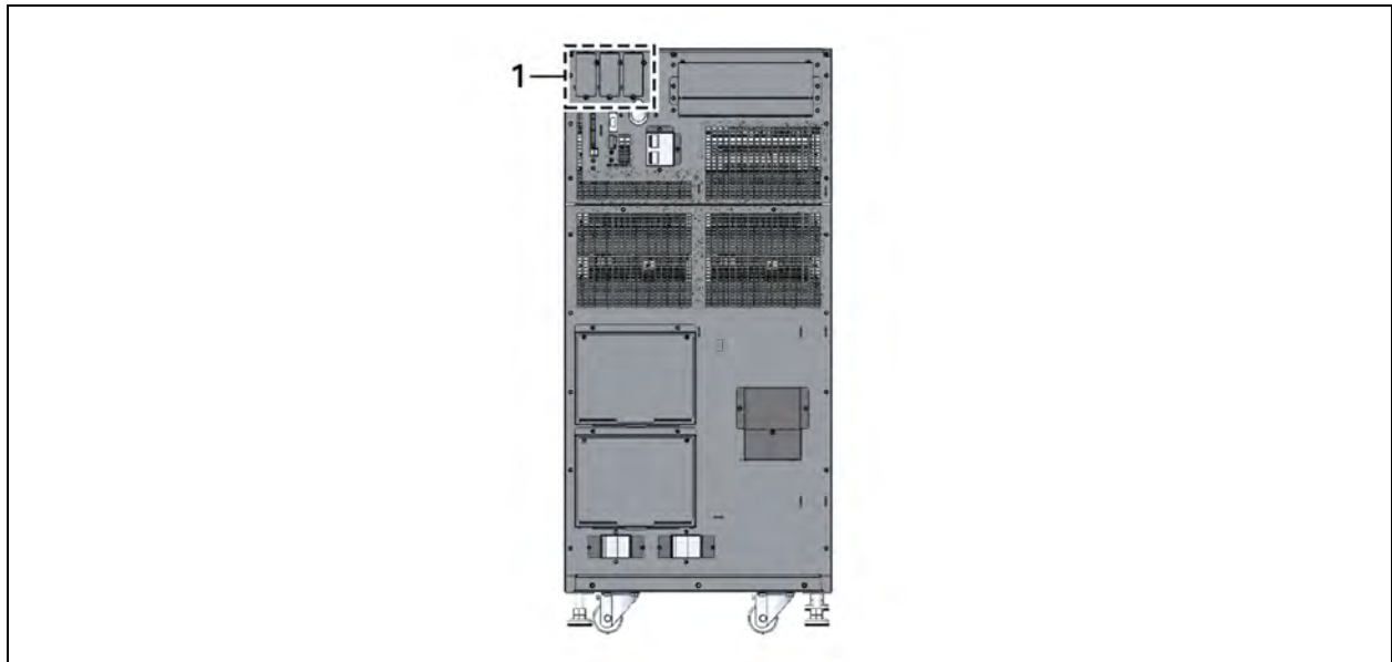
Figure 4.1 Liebert IntelliSlot communication port location
