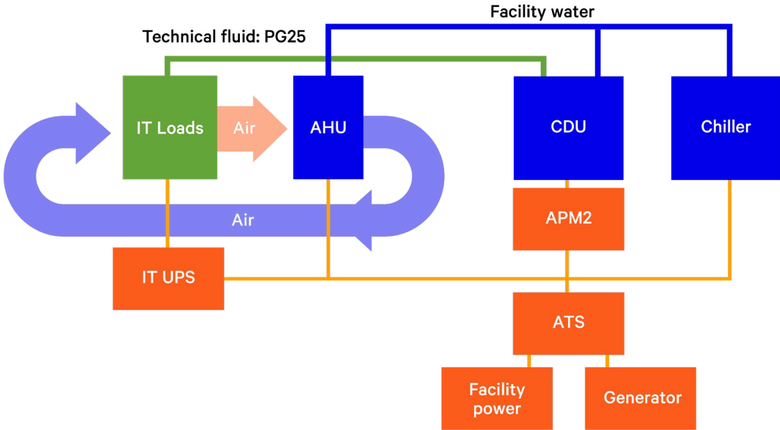
Figure 7. Schematic during laboratory testing. © 2026 Vertiv Group Corp.
