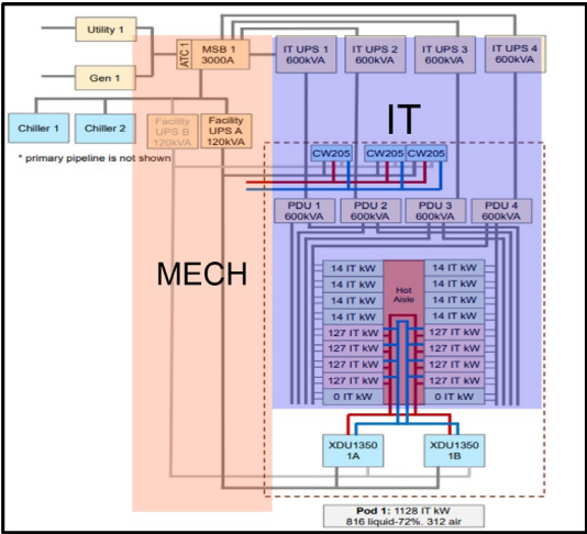
Figure 5. Vertiv™ 360AI Reference Design RD021. Source: Vertiv © 2026 Vertiv Group Corp.
