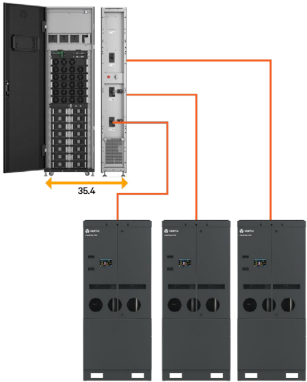
Figure 6. Reference design A: 4MW cooling system. Source: Vertiv © 2026 Vertiv Group Corp.
