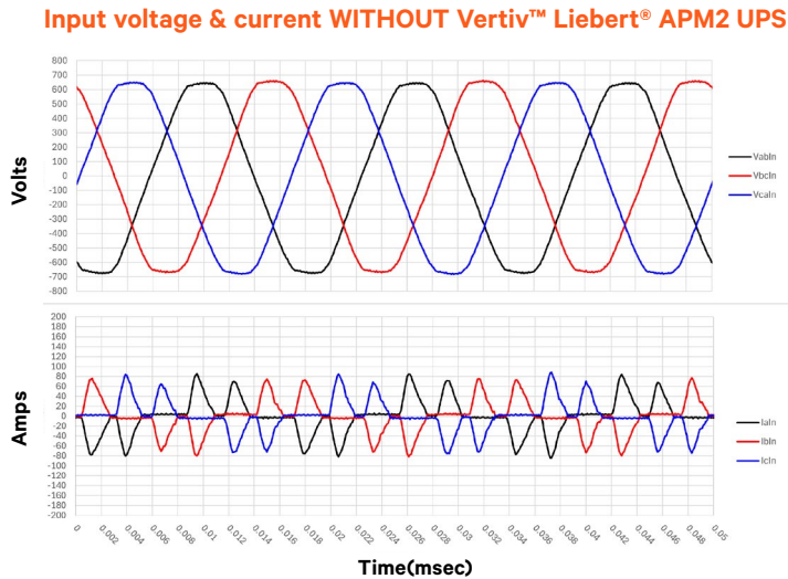
Figure 1. Input voltage and current waveforms WITHOUT Vertiv™ Liebert® APM2 UPS. Source: Vertiv © 2026 Vertiv Group Corp.
