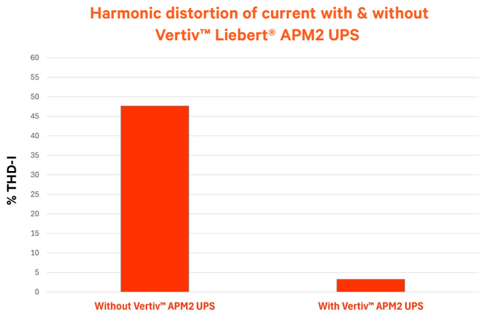
Figure 3. Harmonic distortion - THDi % with and without Vertiv™ Liebert® APM2 UPS. Source: Vertiv © 2026 Vertiv Group Corp.
