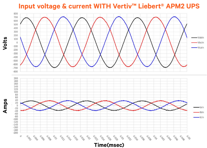
Figure 2. Input voltage and current waveforms WITH Vertiv™ Liebert® APM2 UPS. © 2026 Vertiv Group Corp.
