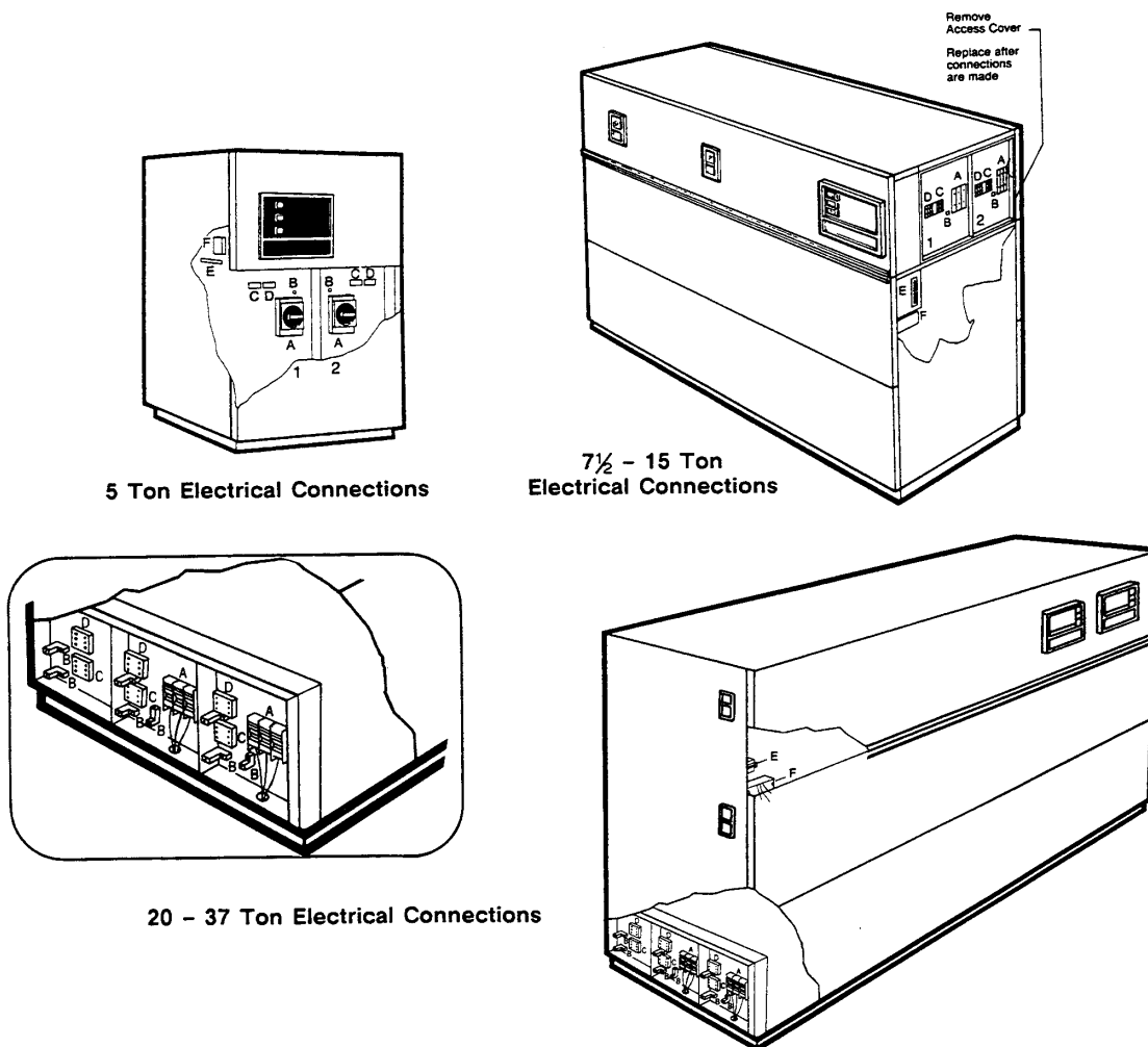
Figure 4 Electrical Connections
