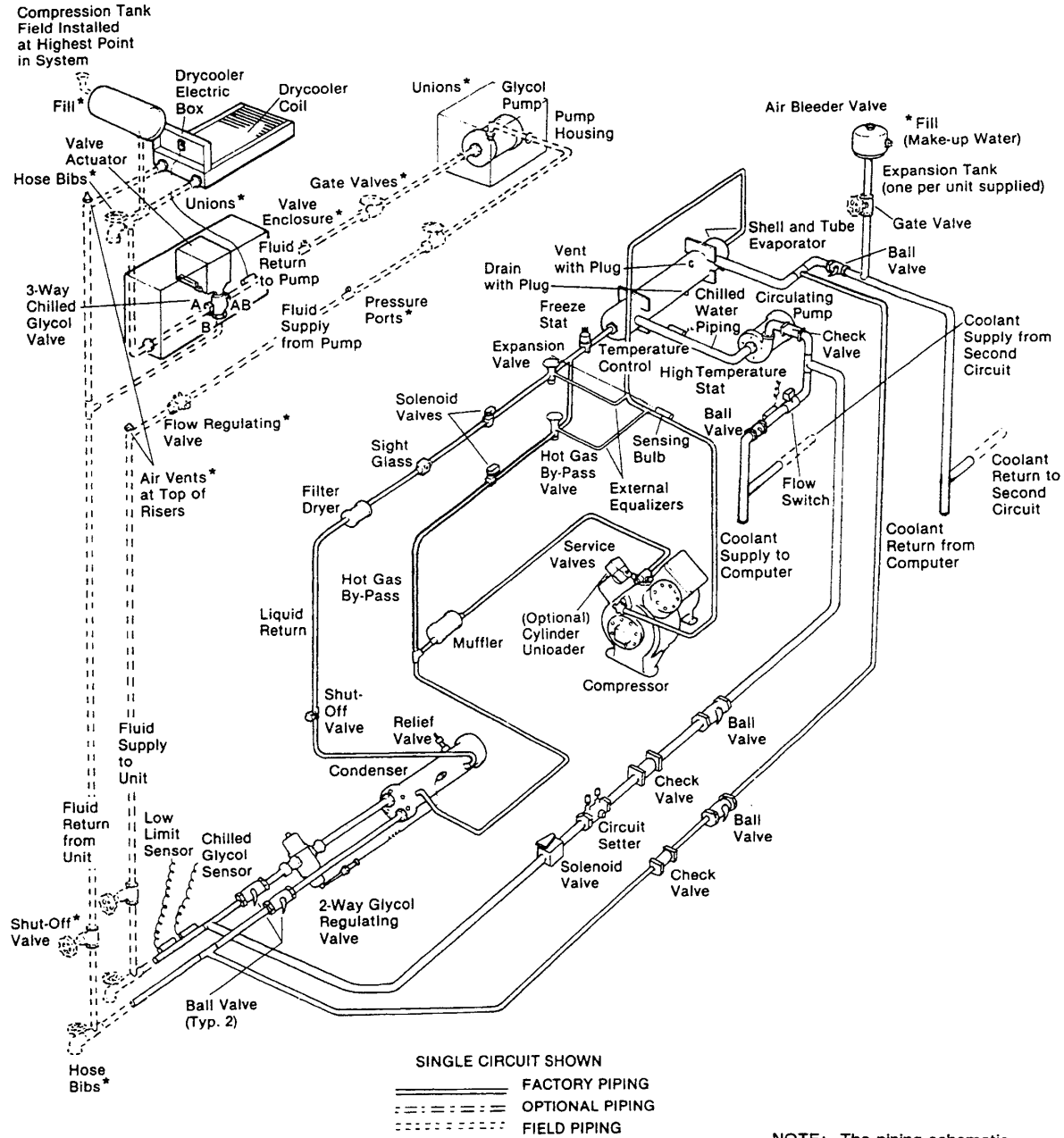
Figure 12 Glycool General Arrangement Diagram
