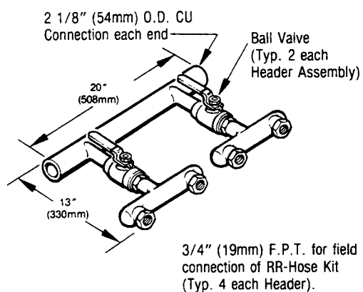
Figure 21 Optional RR830 Underfloor Header Kit
