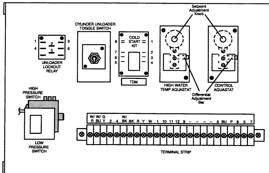
Figure 15 Control Box (with Optional Unloader Components)
