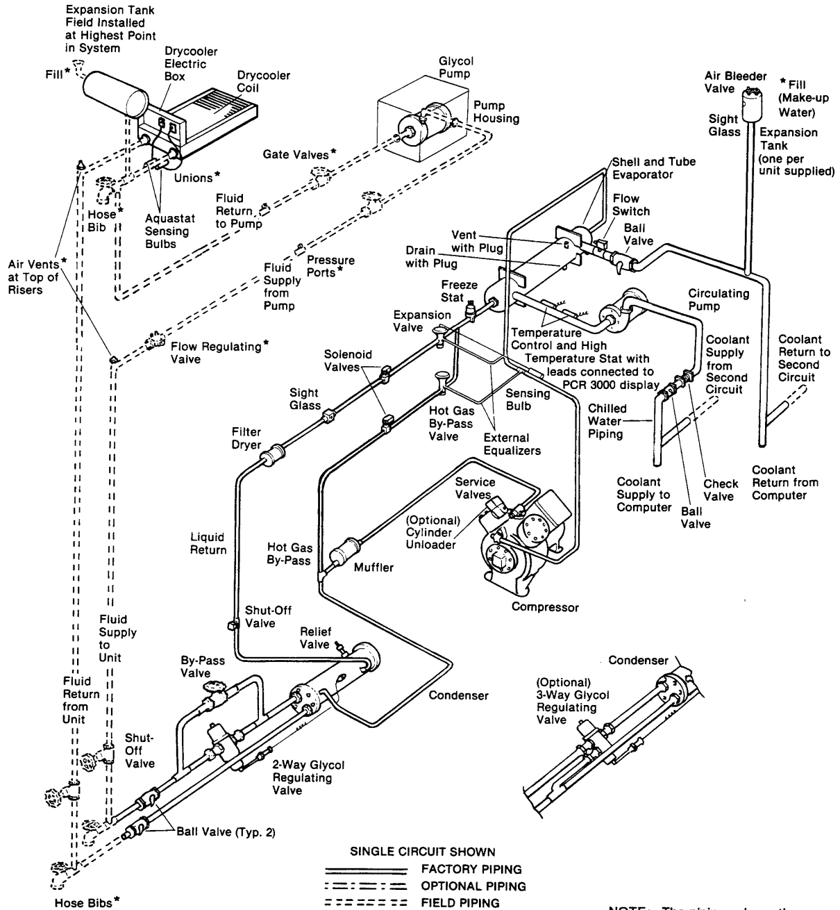
Figure 11 Glycol General Arrangement Drawing
