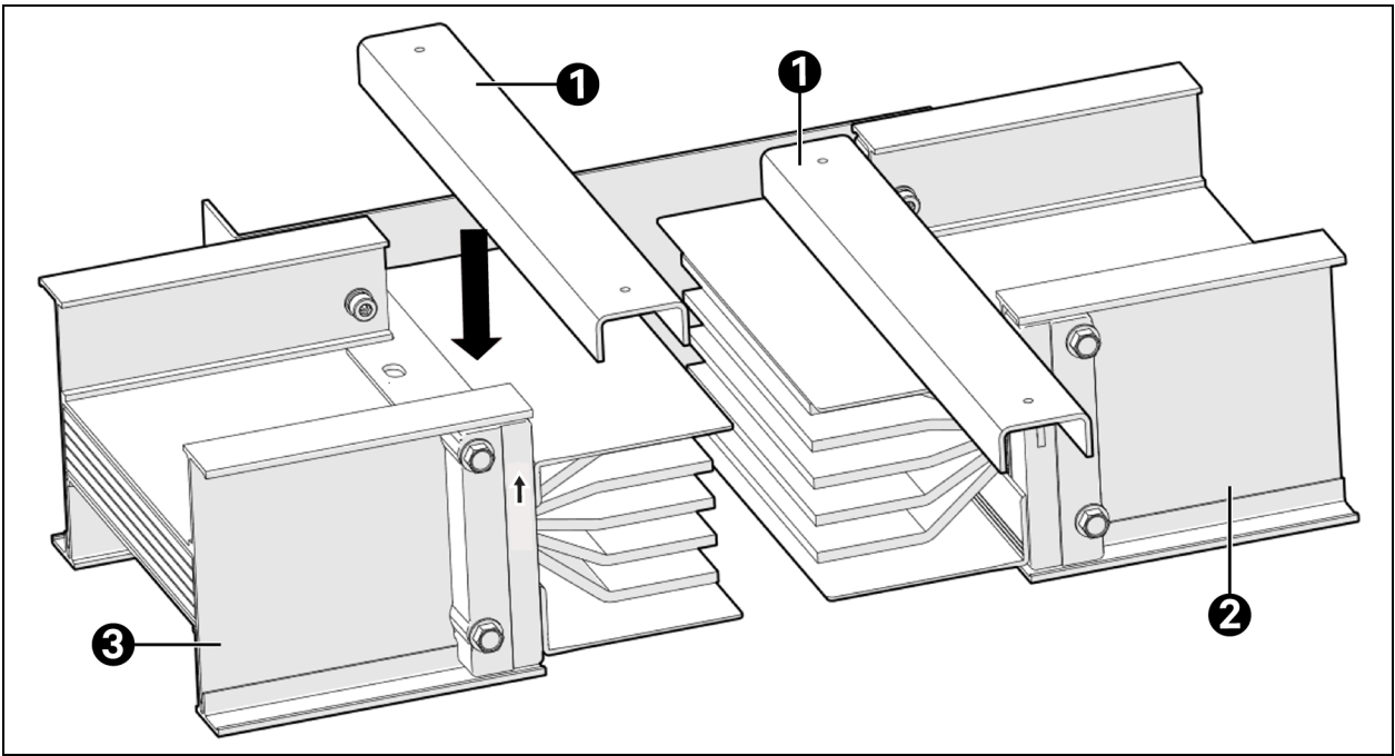
Figure 6.19 Placing Spacer Blocks on Busways
