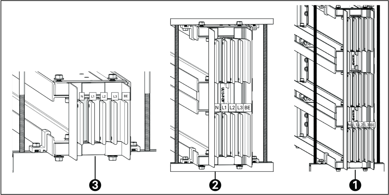
Figure 5.18 Horizontal Edgewise
