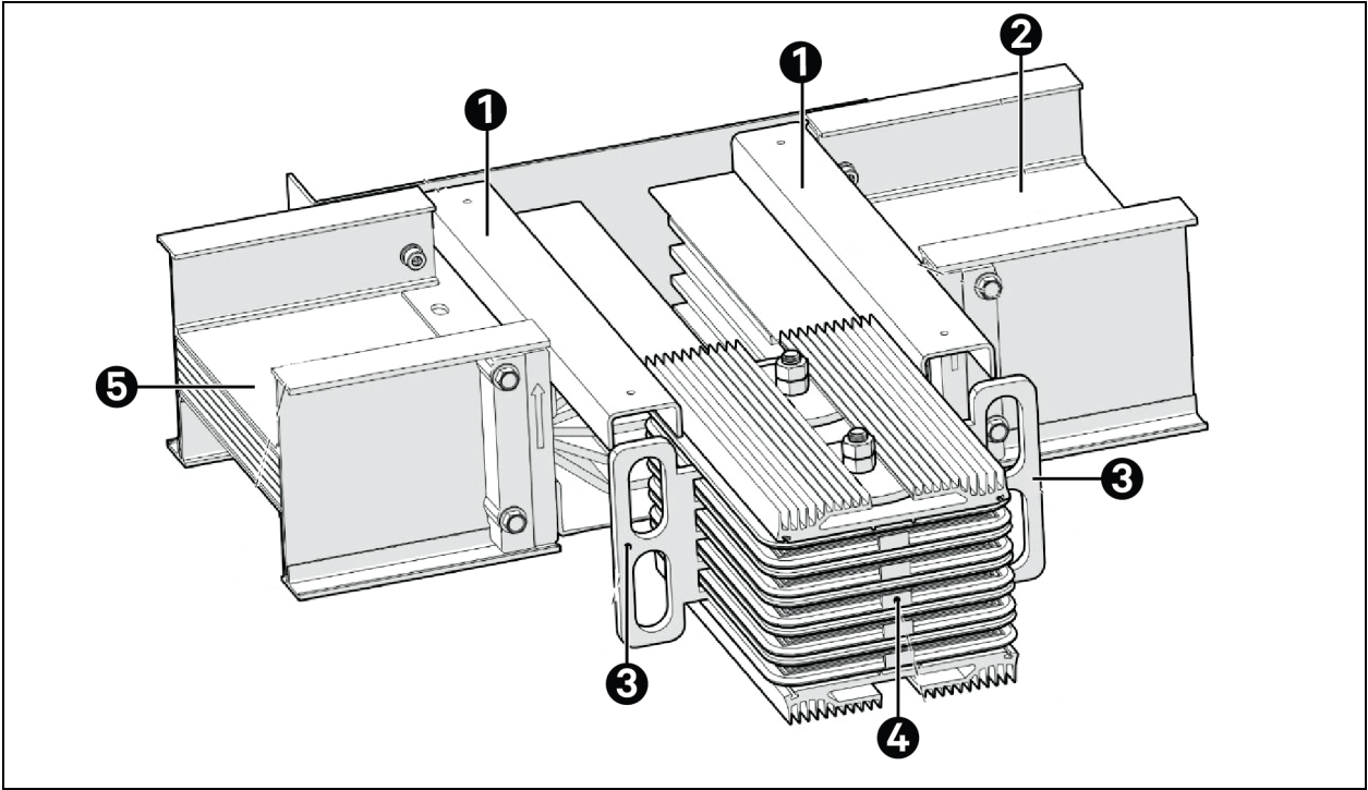
Figure 6.20 Orienting Joint Pack to Busway
