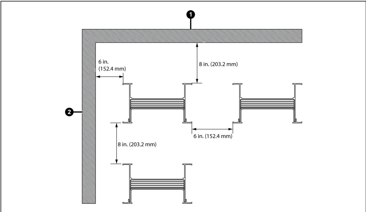
Figure 5.9 Busway Clearances
