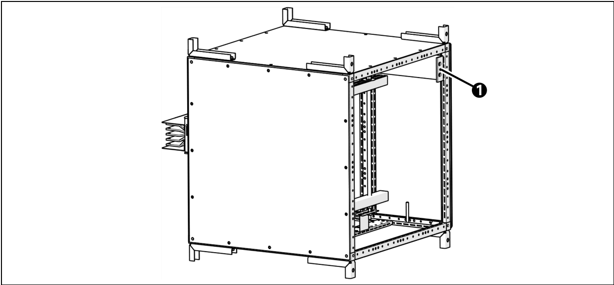
Figure 6.26 Grounding Point
