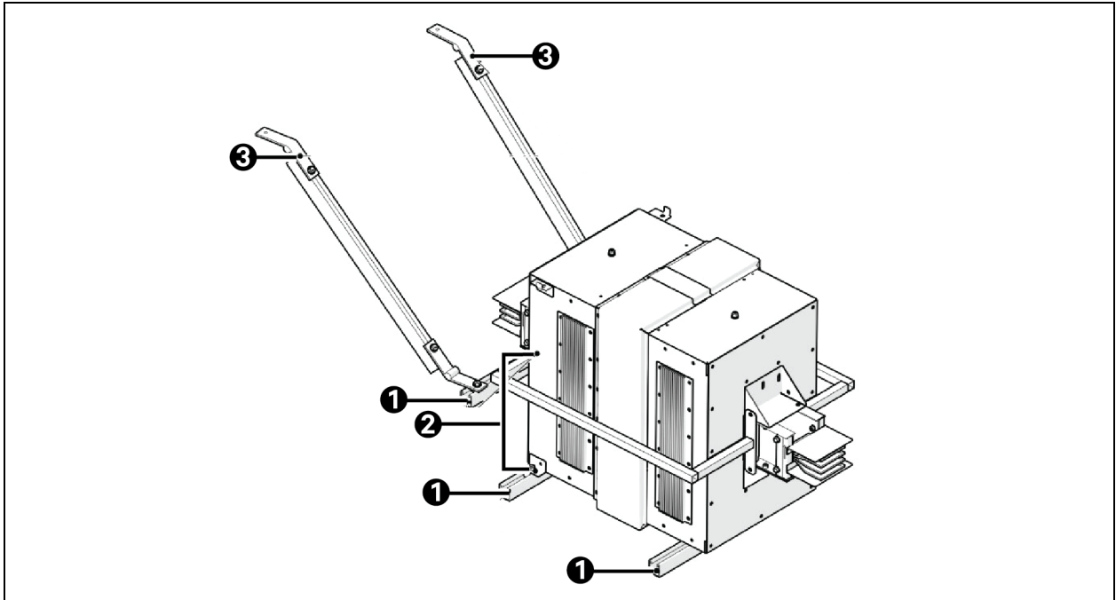
Figure 6.29 Expansion Module
