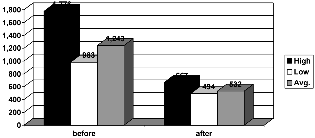
HD-300 Impedance values, before and after Rehydrating and Maximizer installation.
