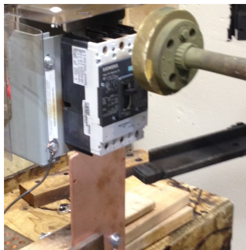
Figure 4. Arc Flash Test Set-Up
