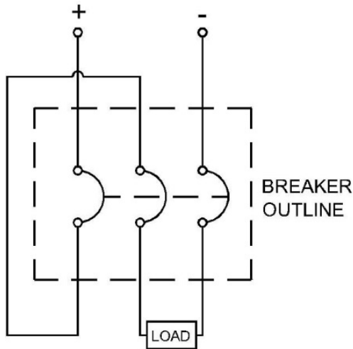
Figure 1. Typical DC Breaker Wiring
