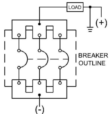
Figure 2. Connections As Tested
