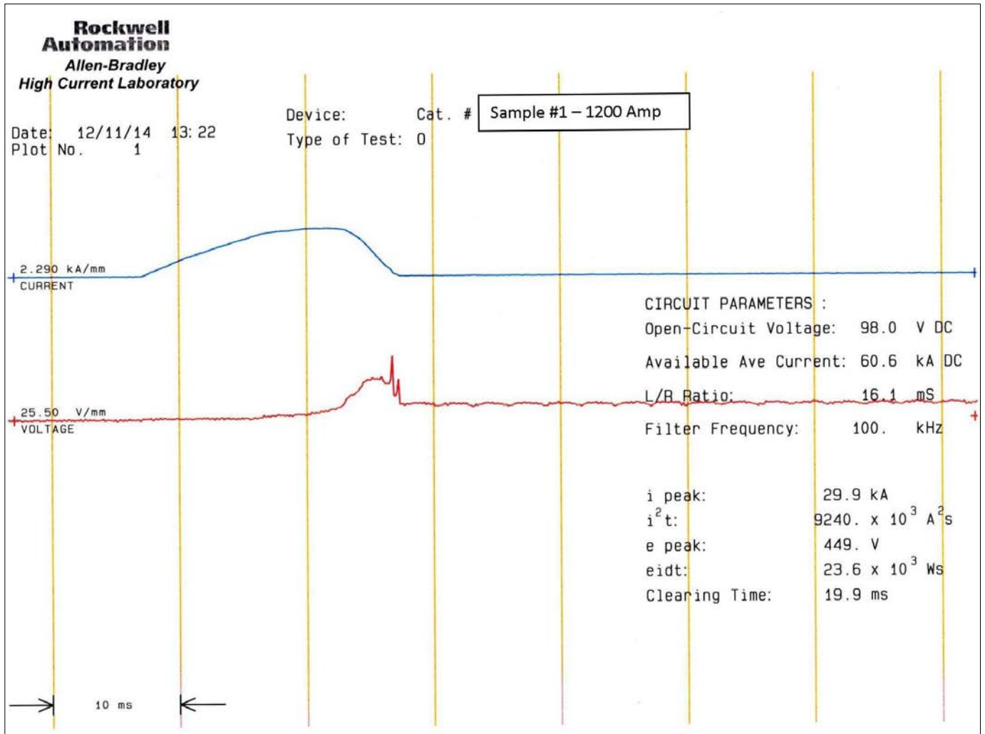
Figure 5. Short Circuit Curve (1200 Amp Sample)
