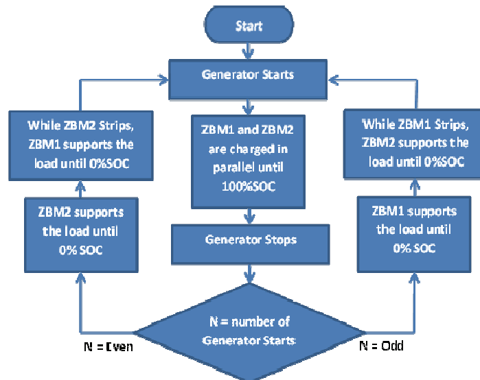
Figure 7 - Telecom Circuit Flow Chart
